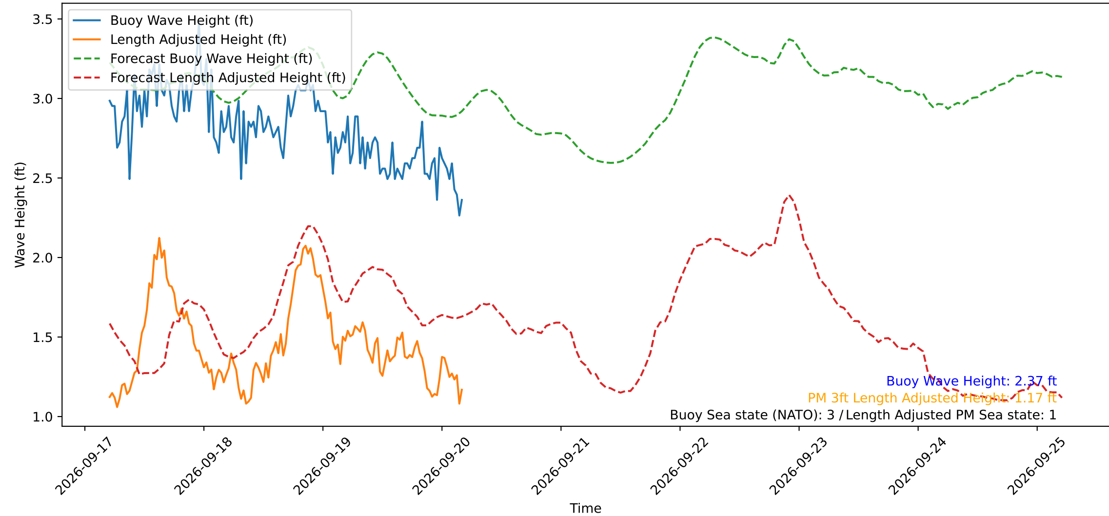
Wave Heights over Time for Green Beach at 2026-09-20 04:41:12
