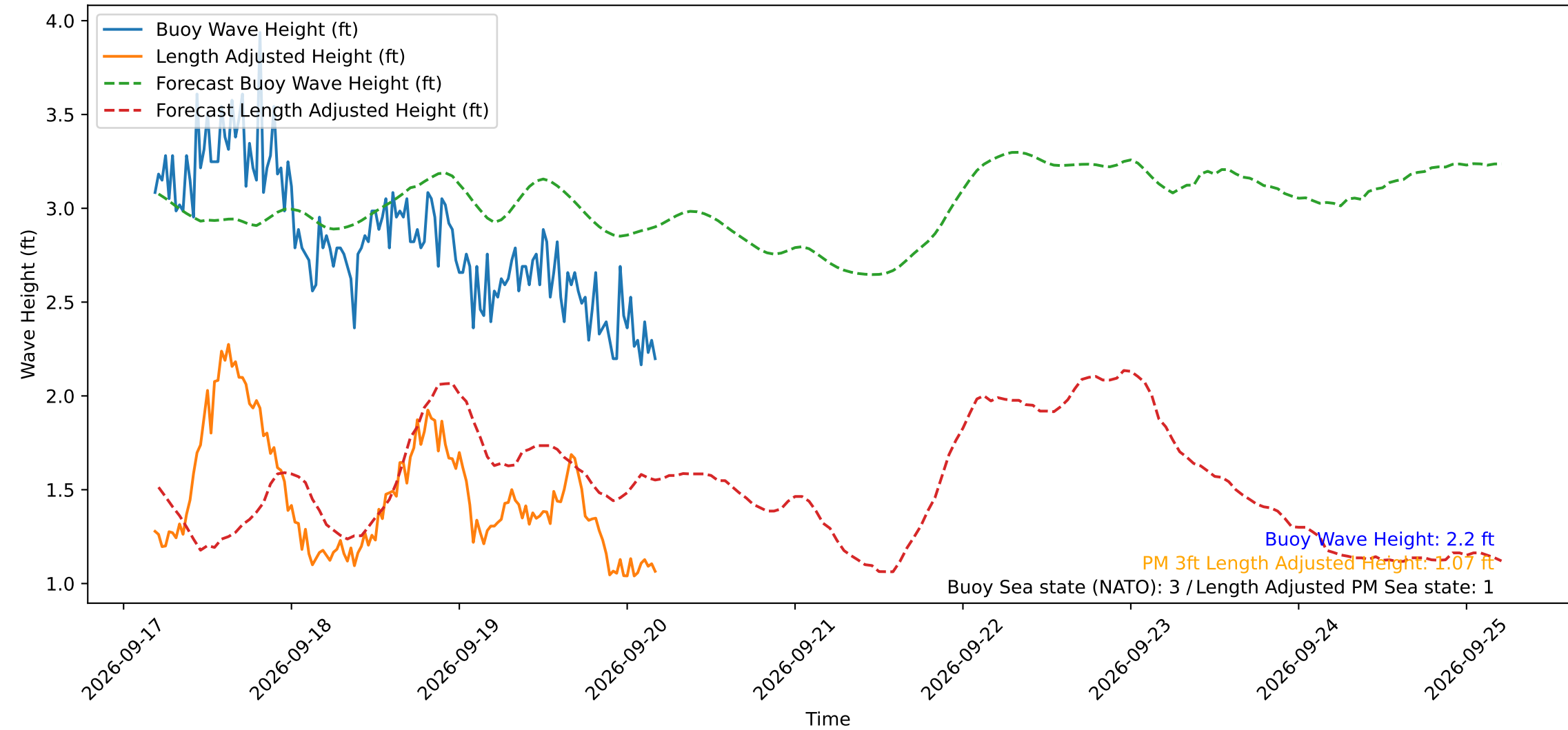
Wave Heights over Time for Oceanside Harbor at 2026-09-20 04:40:30
