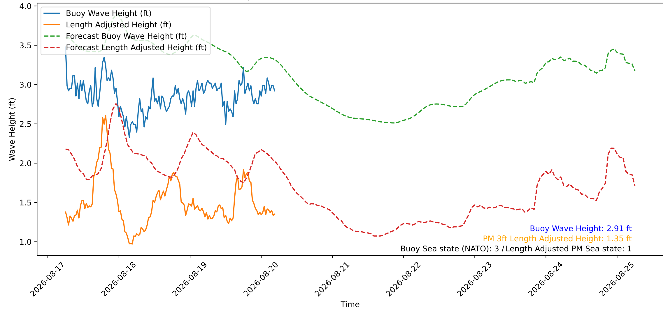
Wave Heights over Time for Red Beach at 2026-08-20 05:30:45
