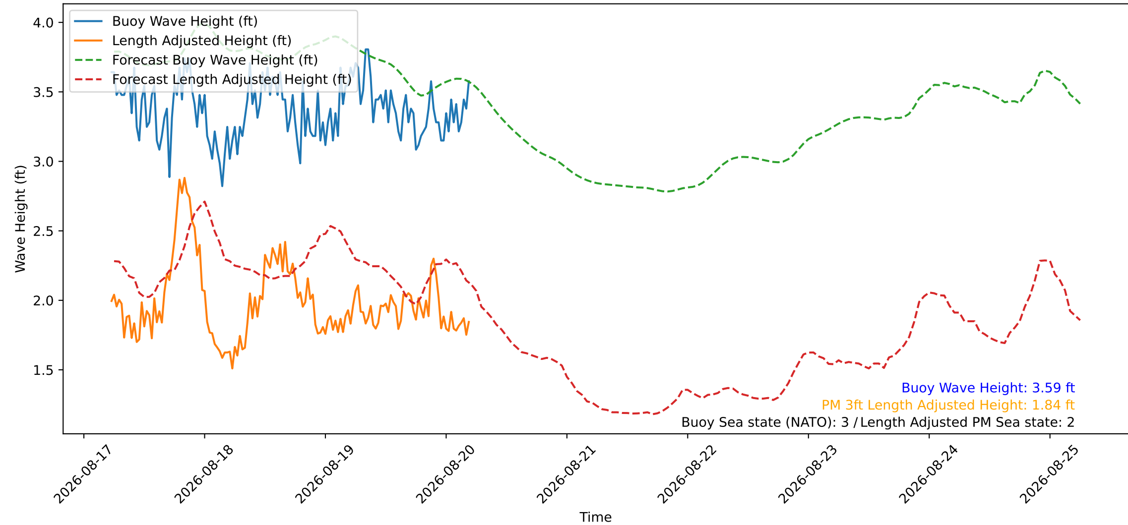
Wave Heights over Time for Oceanside Harbor at 2026-08-20 05:30:26
