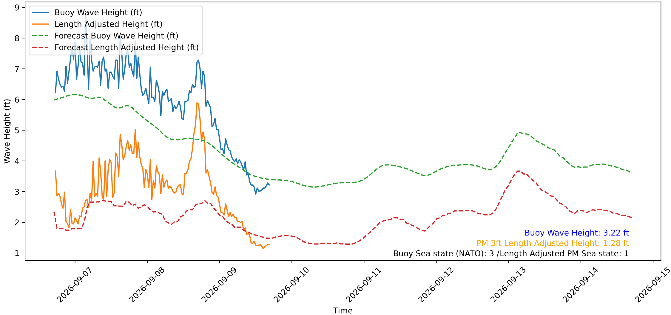
Wave Heights over Time for Green Beach at 2026-09-09 17:21:15
