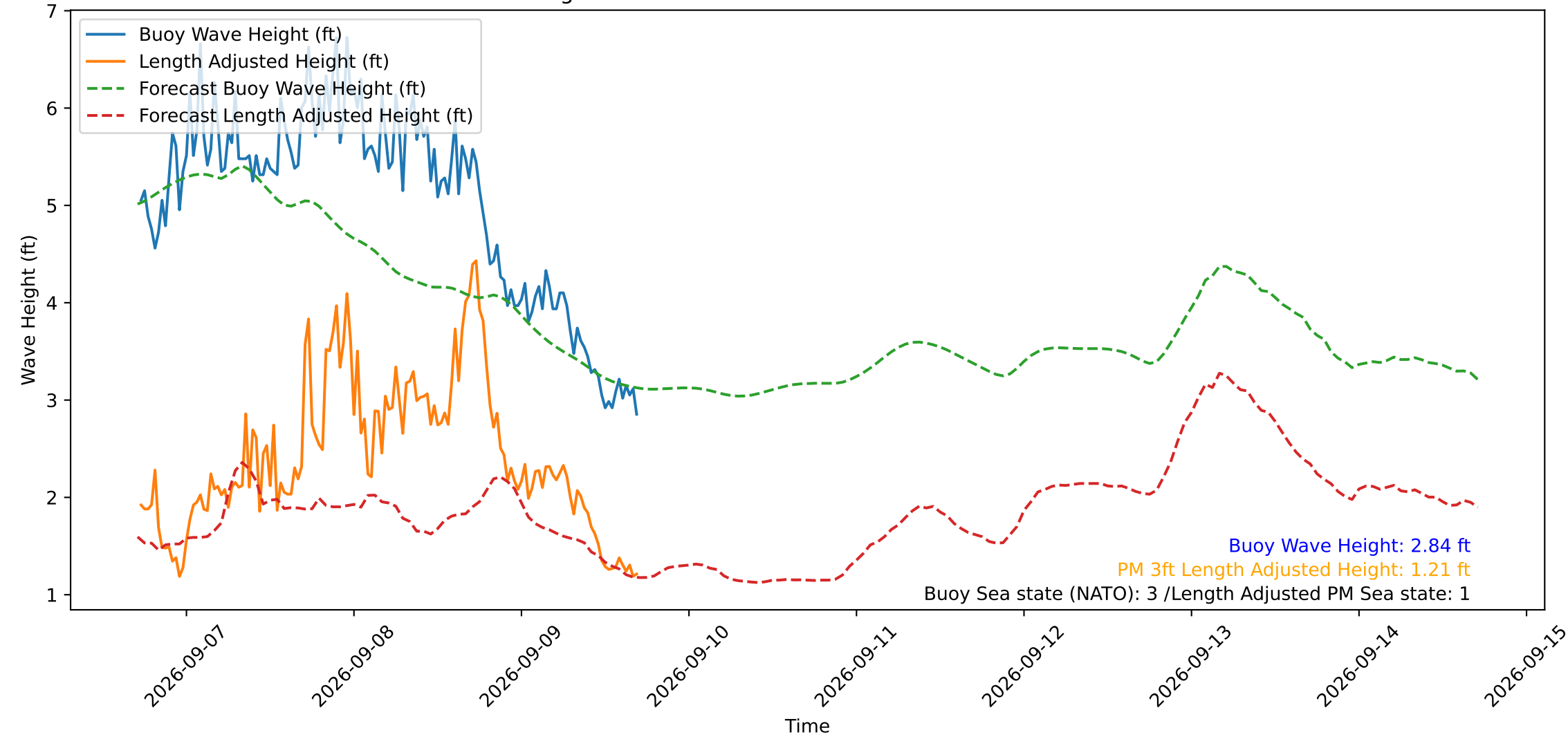
Wave Heights over Time for Red Beach at 2026-09-09 17:20:51
