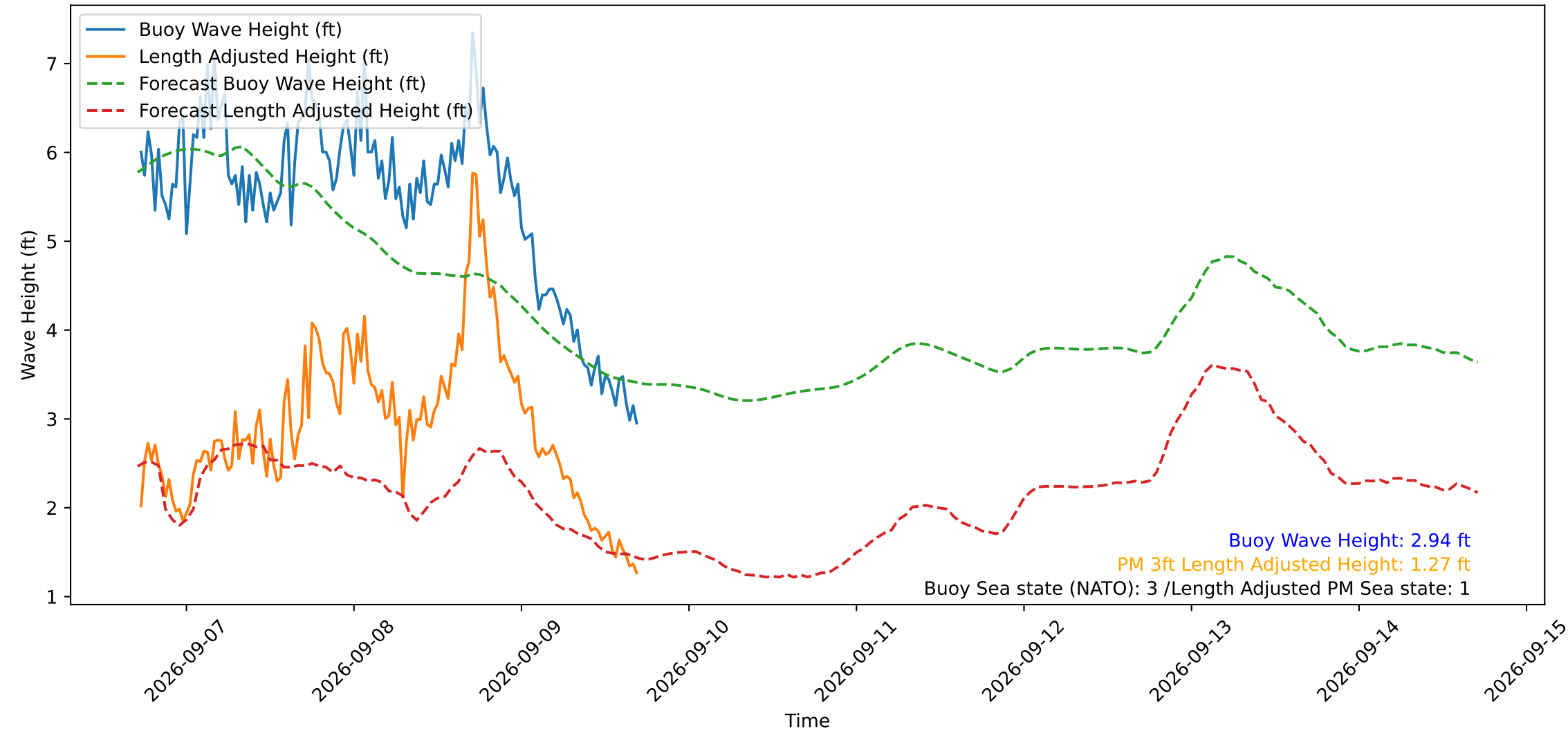
Wave Heights over Time for Oceanside Harbor at 2026-09-09 17:20:29
