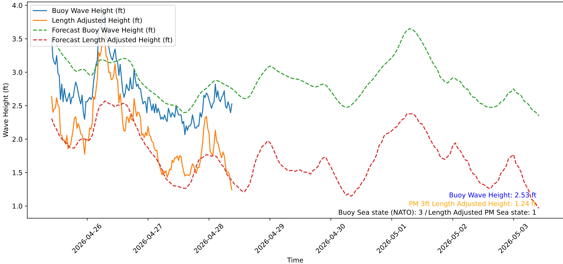
Wave Heights over Time for Oceanside Harbor at 2026-04-28 09:50:31
