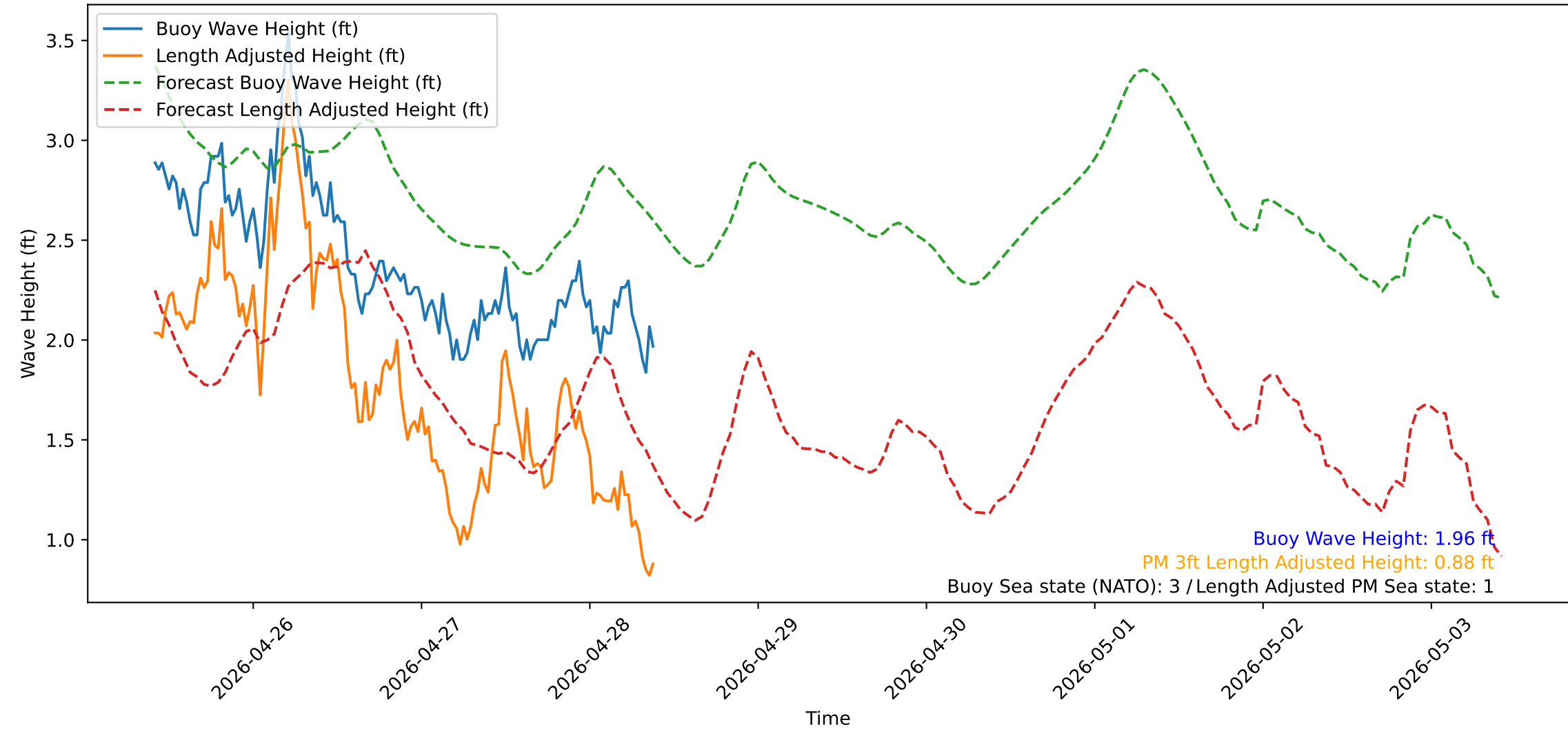
Wave Heights over Time for Red Beach at 2026-04-28 09:50:53
