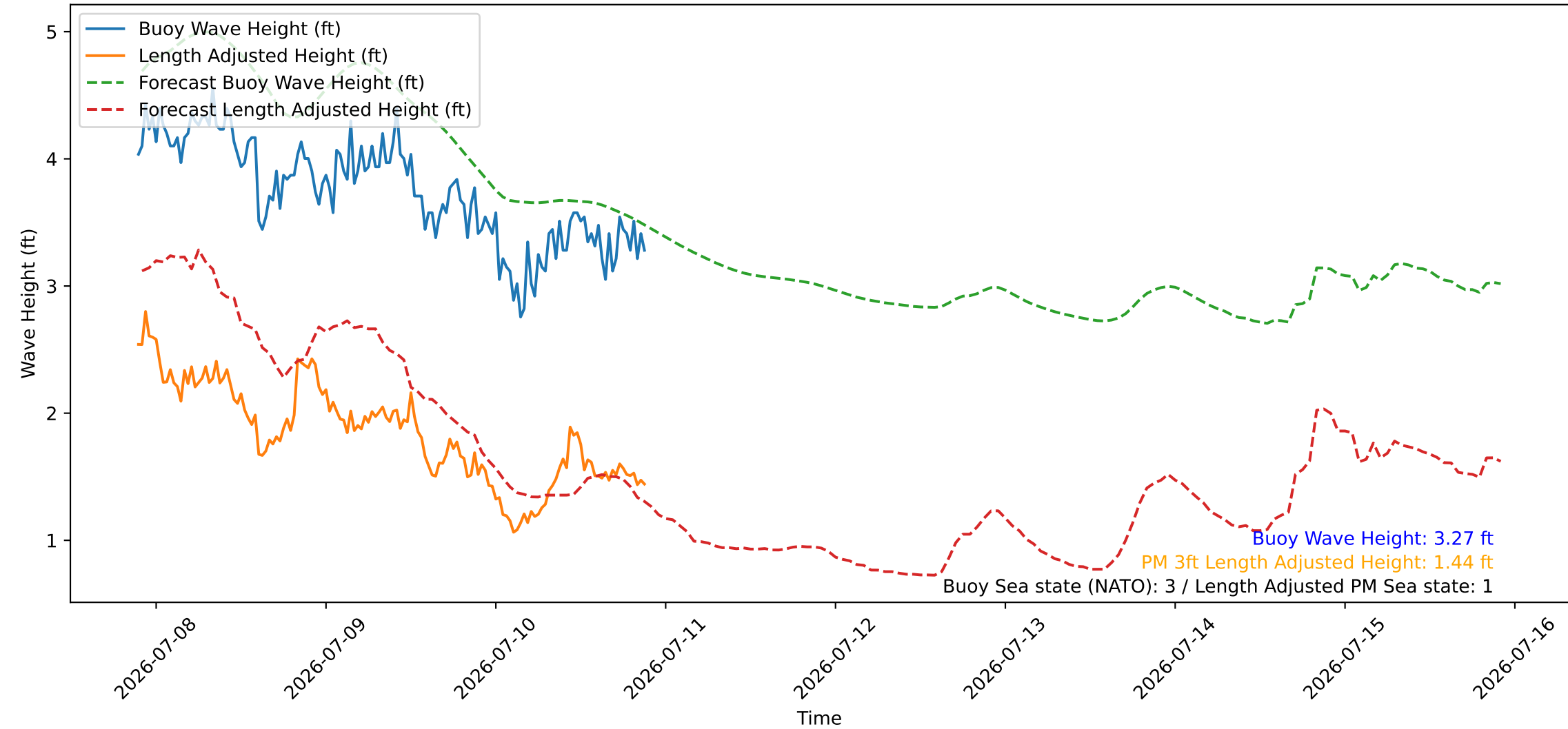
Wave Heights over Time for Green Beach at 2026-07-10 21:41:08
