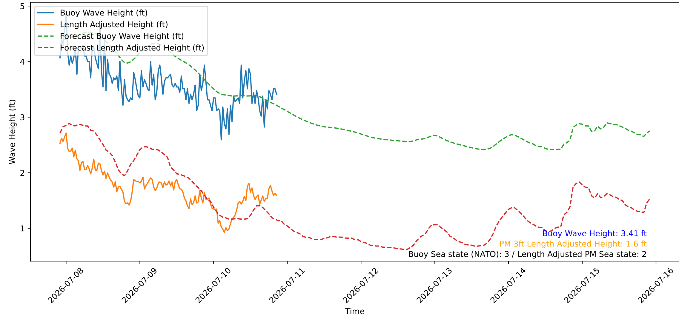
Wave Heights over Time for Red Beach at 2026-07-10 21:40:46
