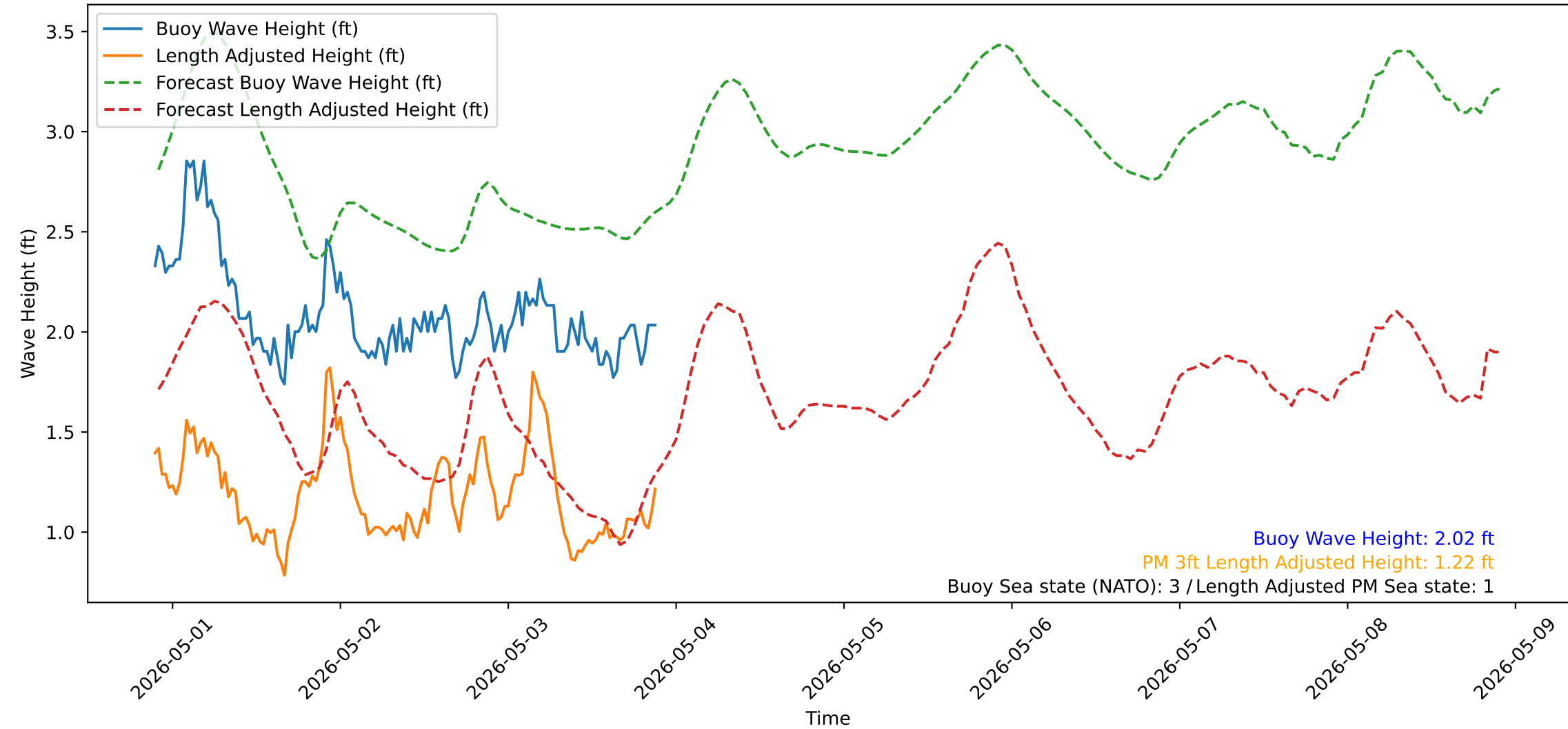
Wave Heights over Time for Green Beach at 2026-05-03 21:41:13
