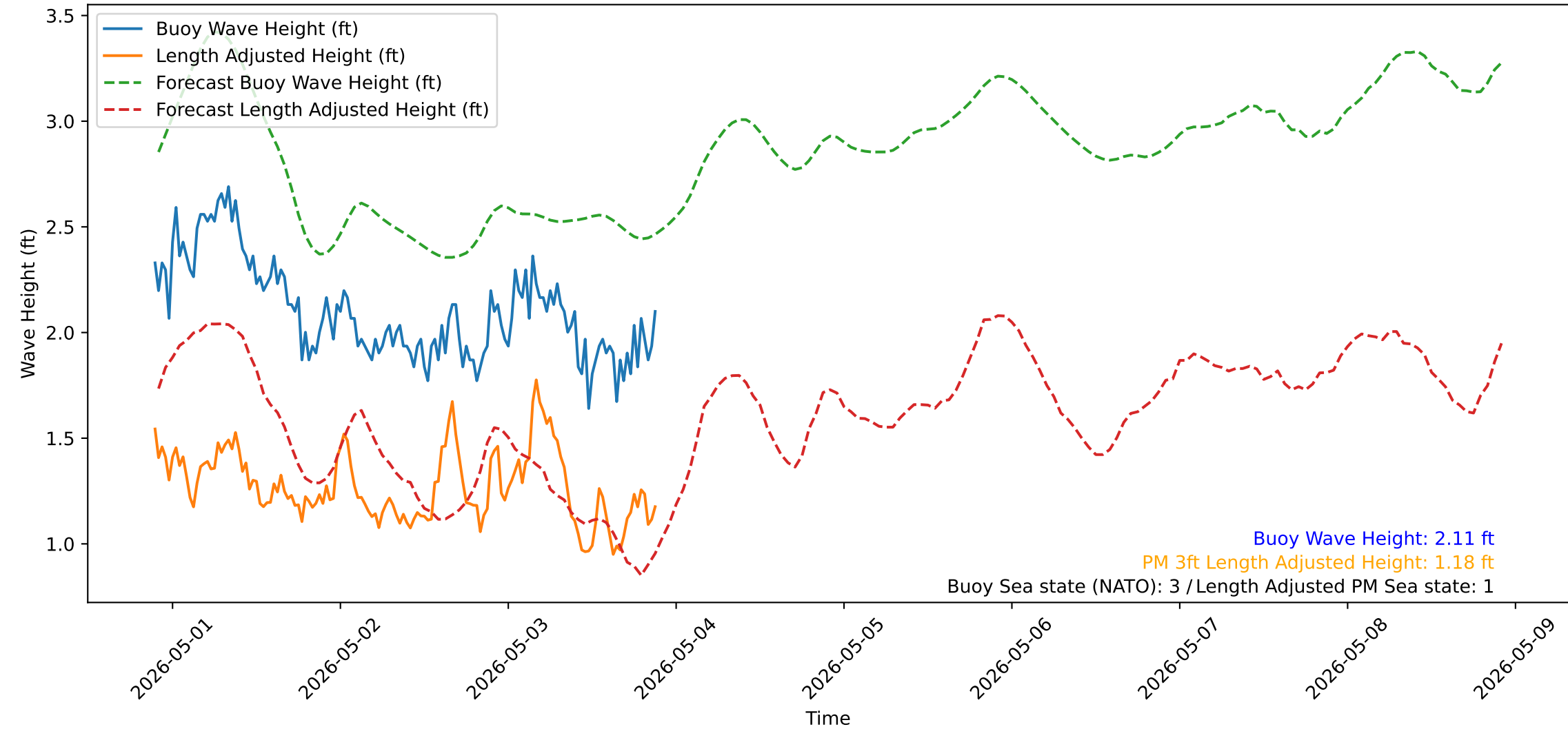
Wave Heights over Time for Oceanside Harbor at 2026-05-03 21:40:32
