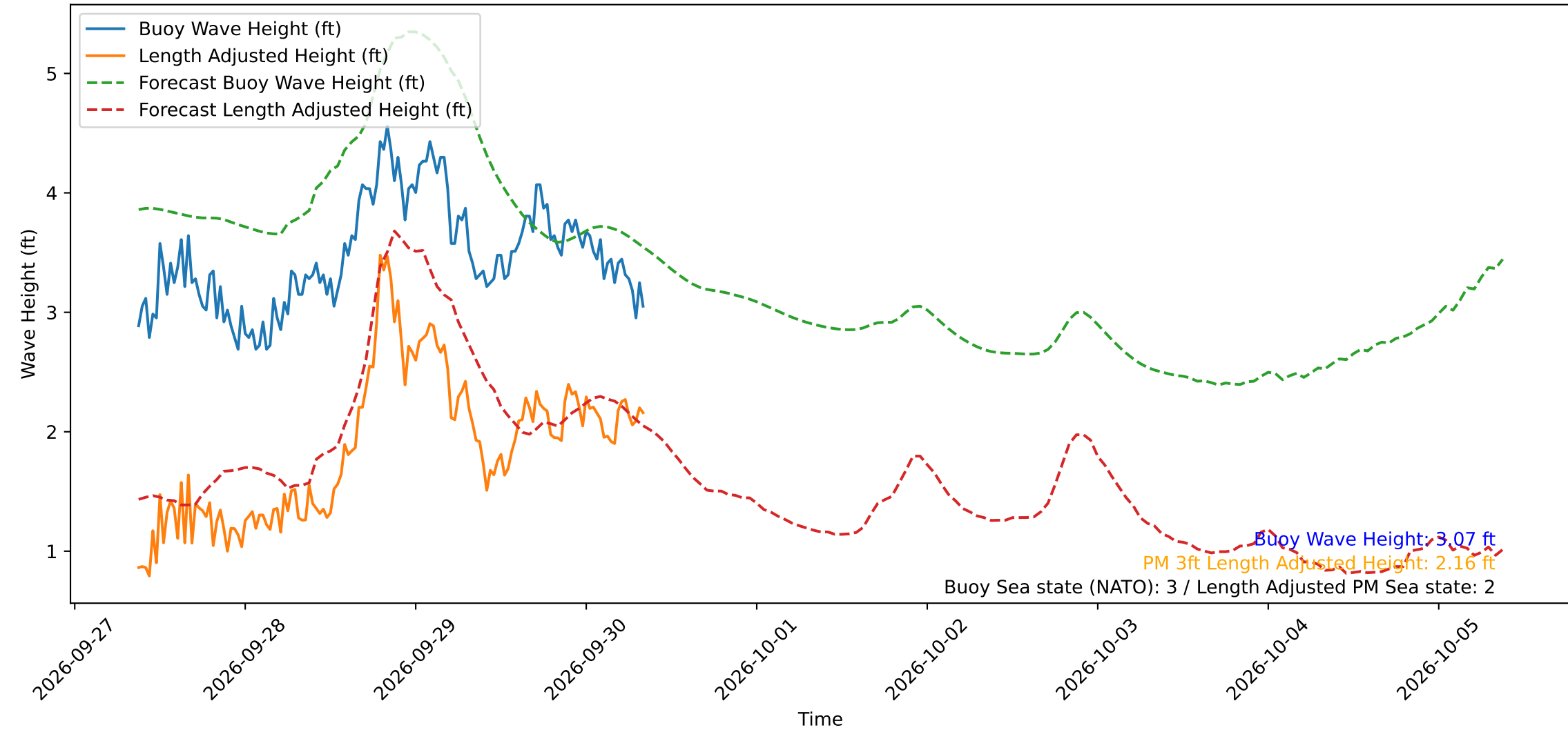
Wave Heights over Time for Green Beach at 2026-09-30 08:51:13
