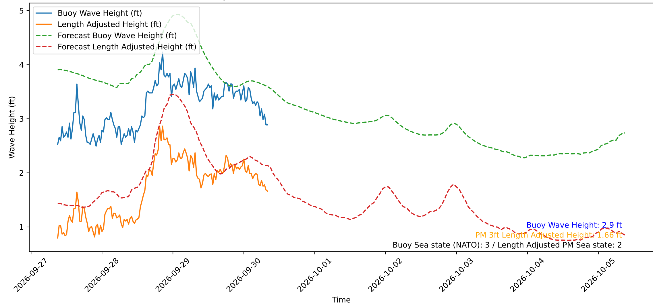
Wave Heights over Time for Oceanside Harbor at 2026-09-30 08:50:29
