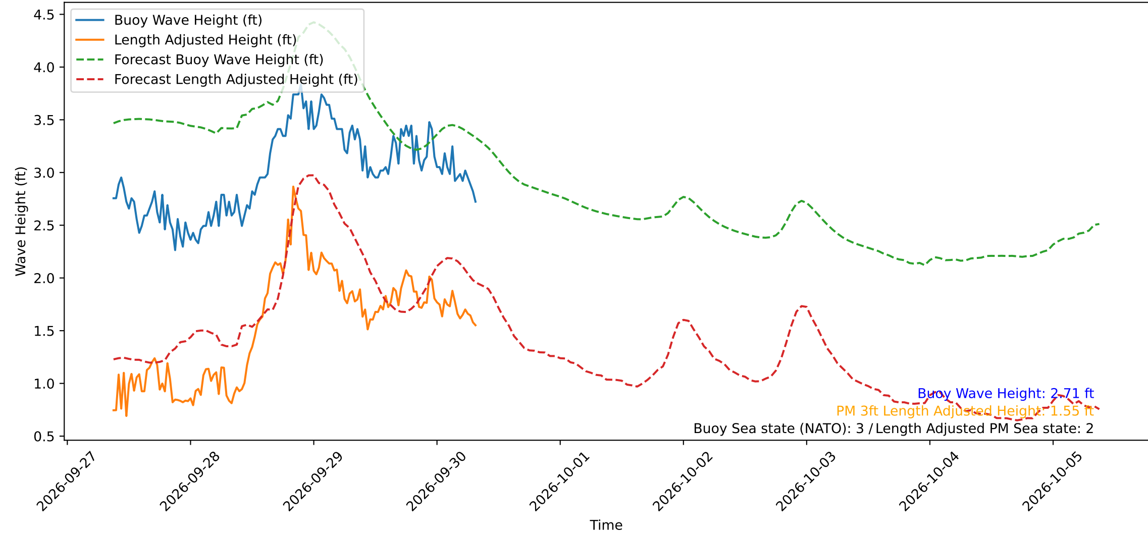
Wave Heights over Time for Red Beach at 2026-09-30 08:50:49
