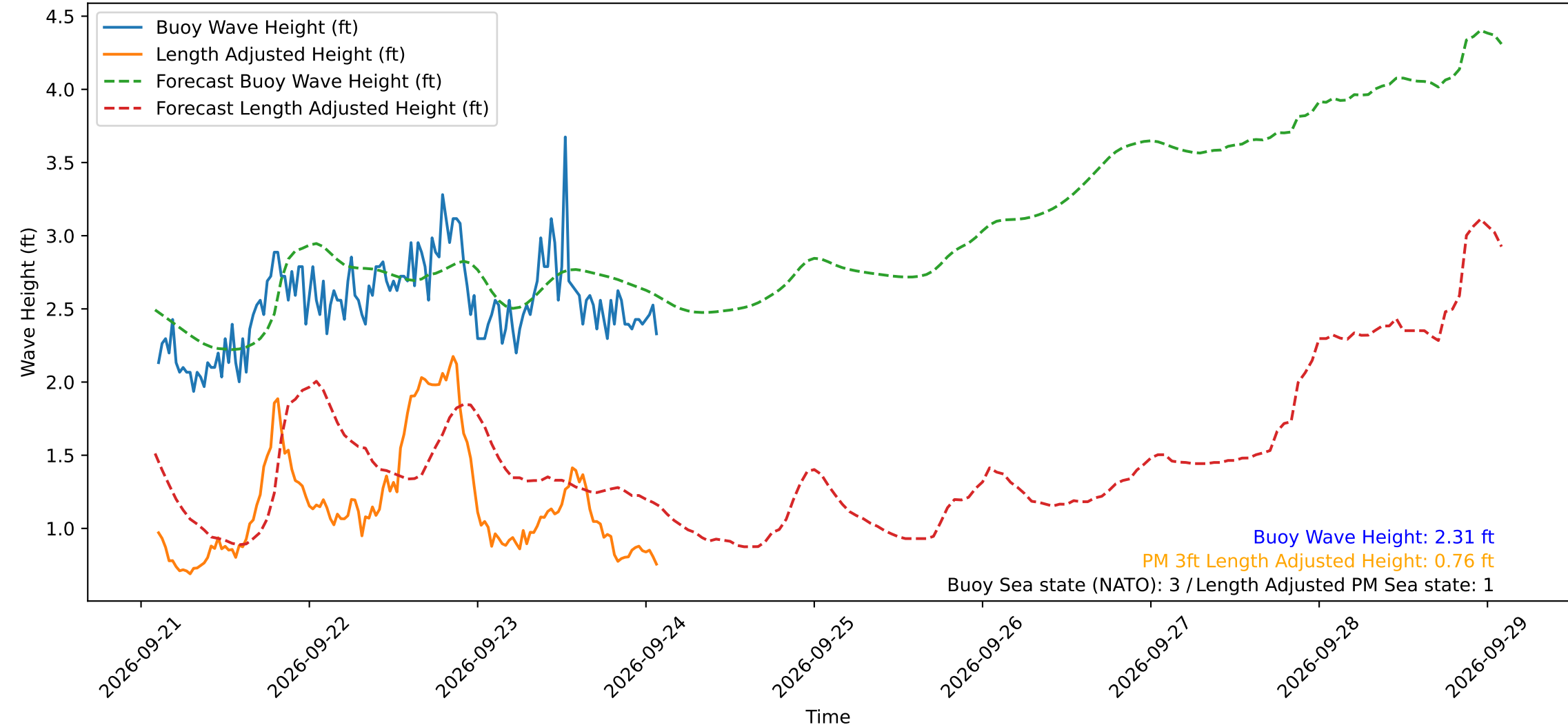
Wave Heights over Time for Red Beach at 2026-09-24 02:10:49
