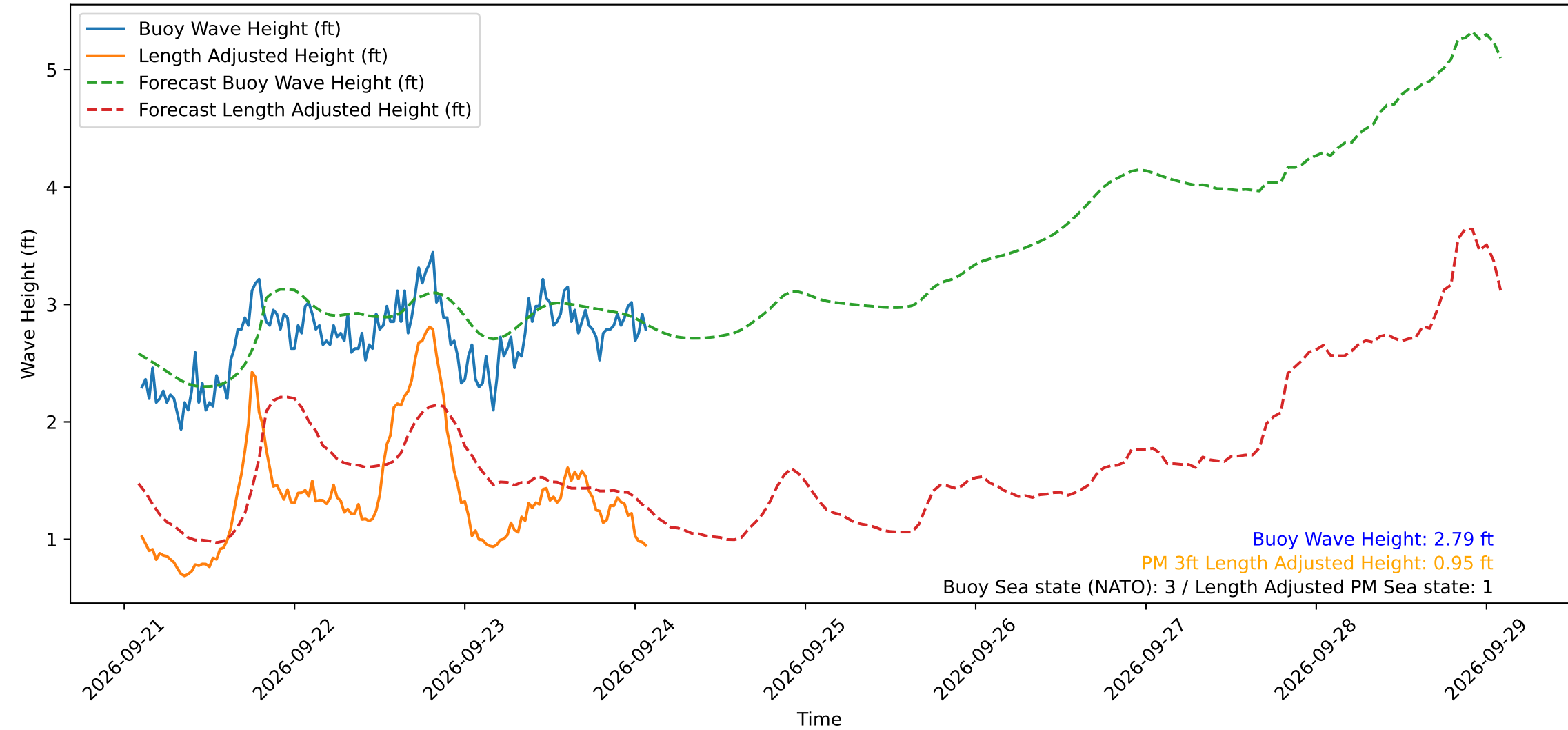
Wave Heights over Time for Green Beach at 2026-09-24 02:11:11
