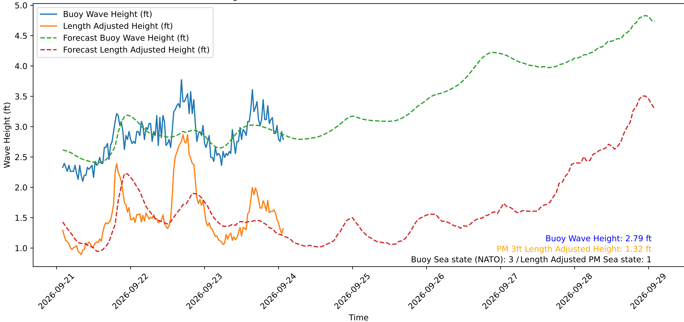
Wave Heights over Time for Oceanside Harbor at 2026-09-24 02:10:29
