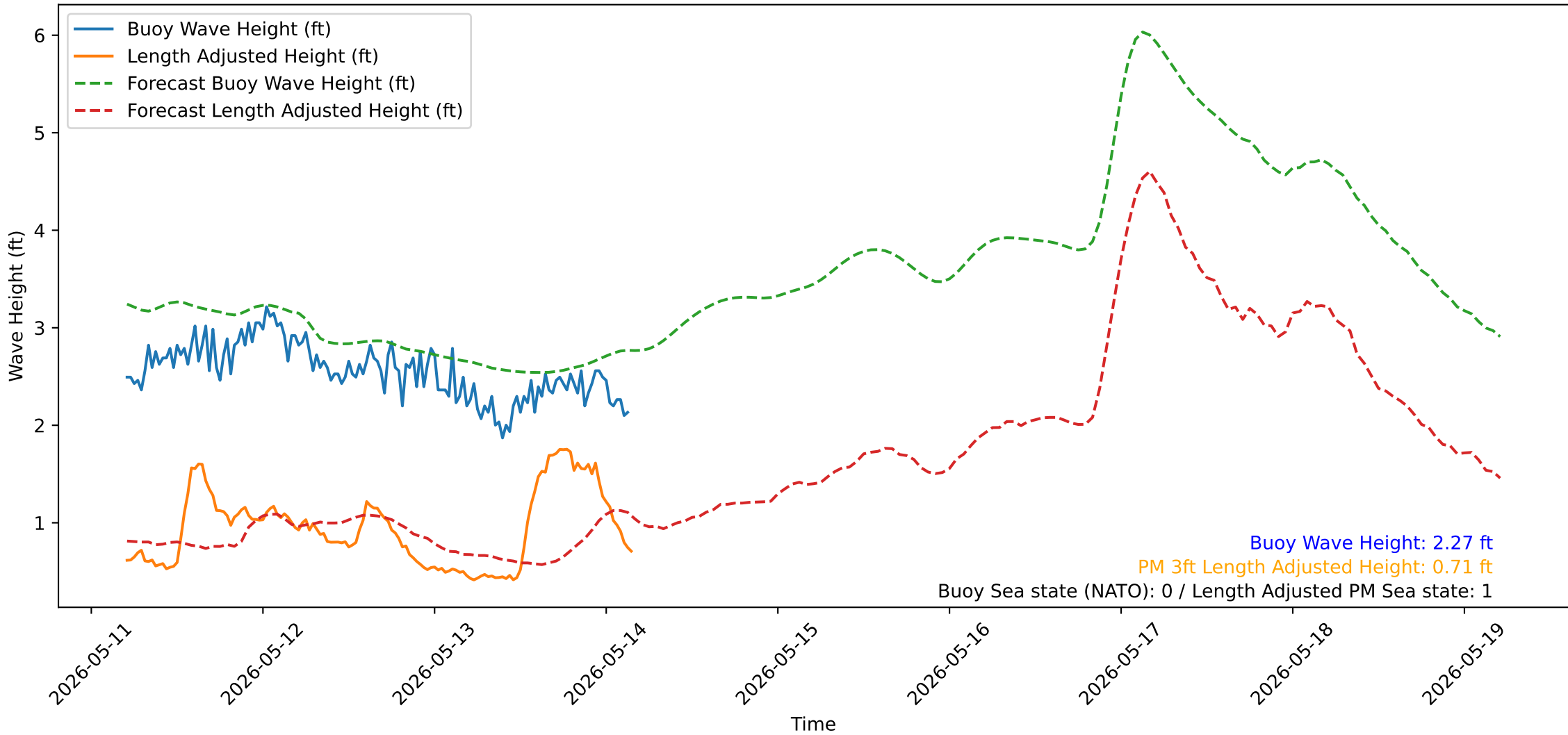
Wave Heights over Time for Red Beach at 2026-05-14 04:30:51
