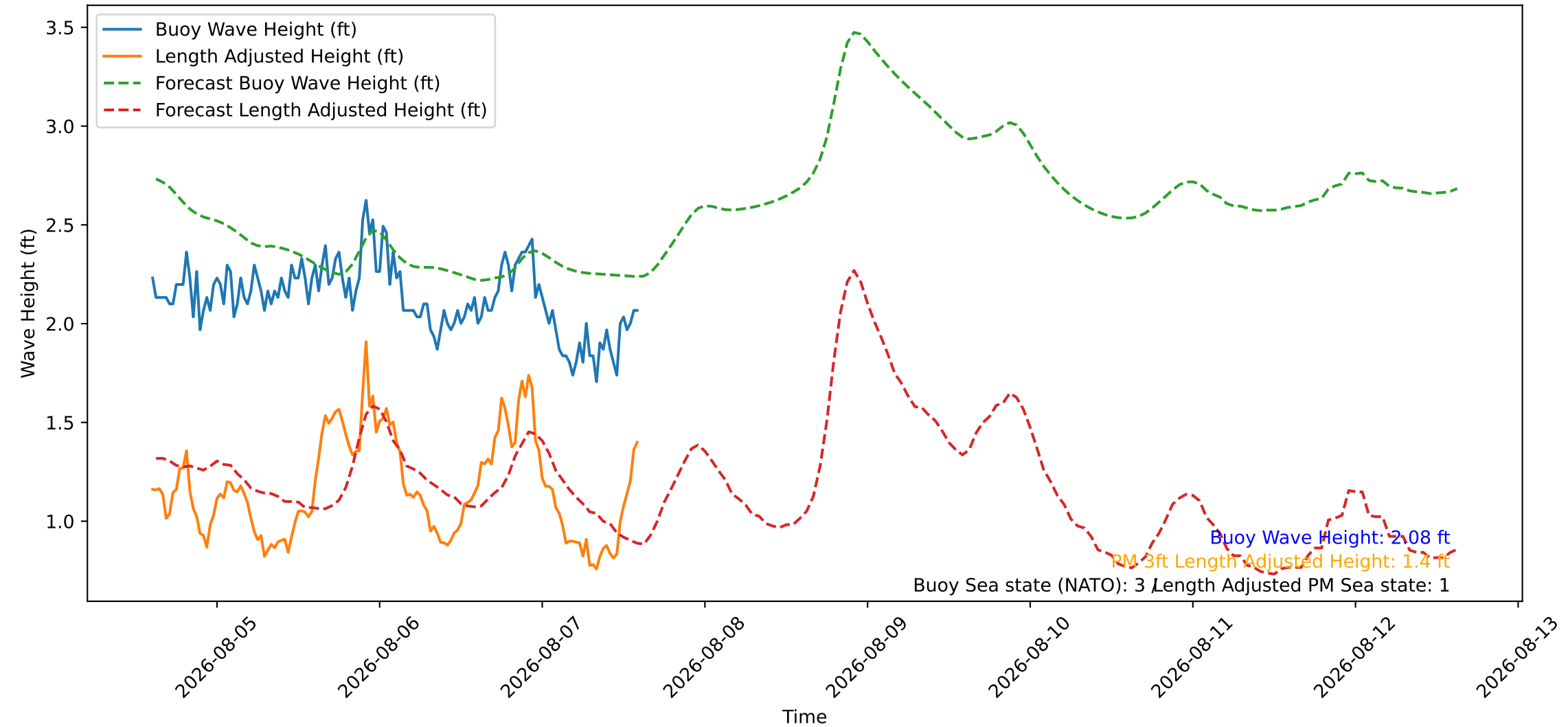
Wave Heights over Time for Green Beach at 2026-08-07 14:41:09
