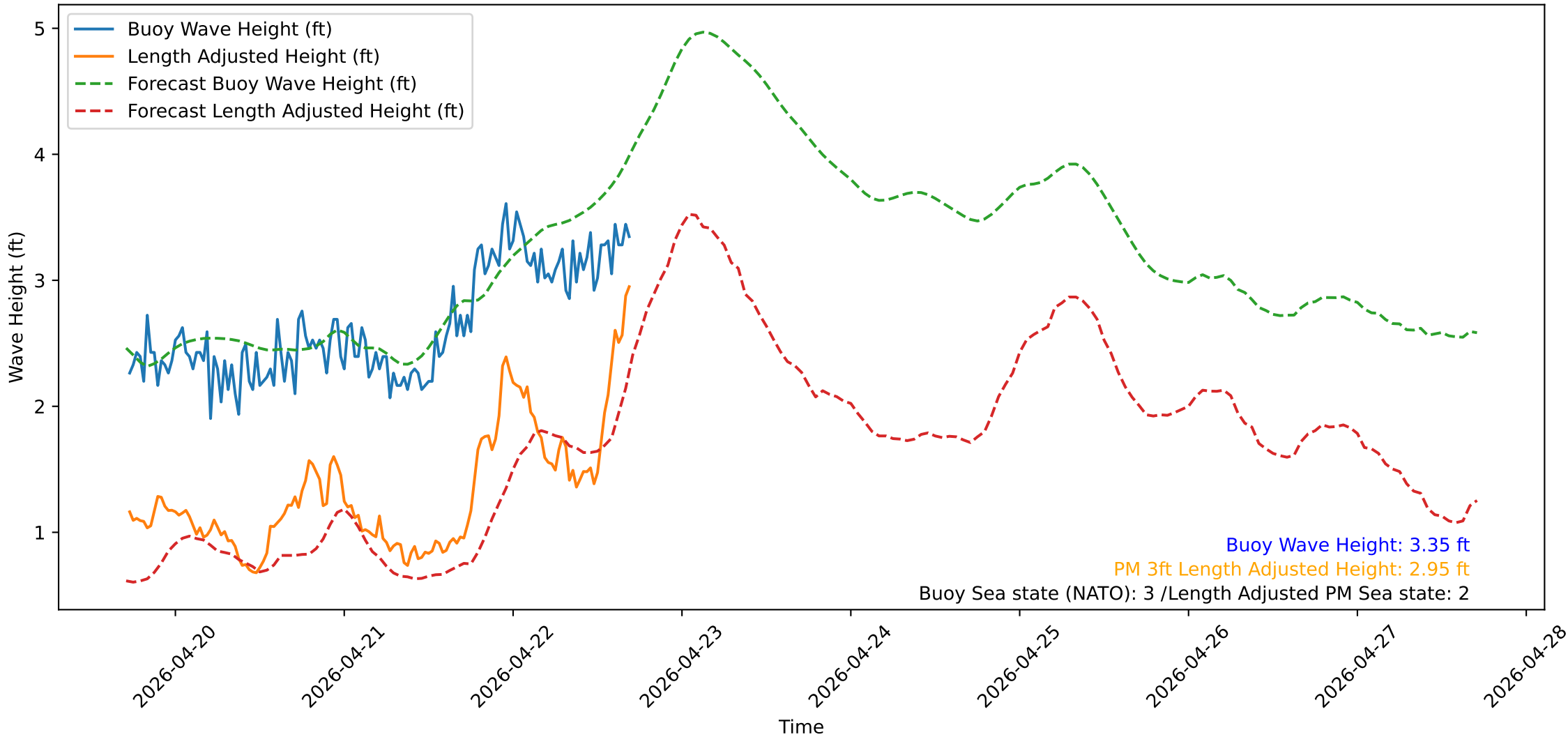
Wave Heights over Time for Oceanside Harbor at 2026-04-22 17:20:31
