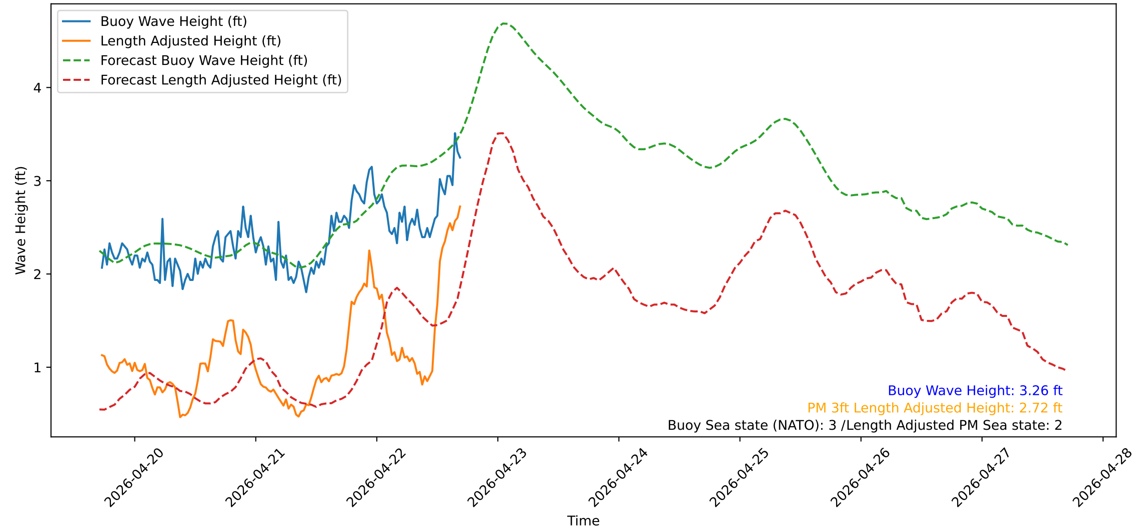
Wave Heights over Time for Red Beach at 2026-04-22 17:20:51
