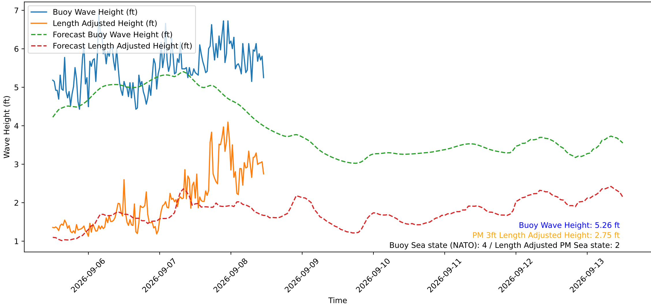
Wave Heights over Time for Red Beach at 2026-09-08 11:50:50
