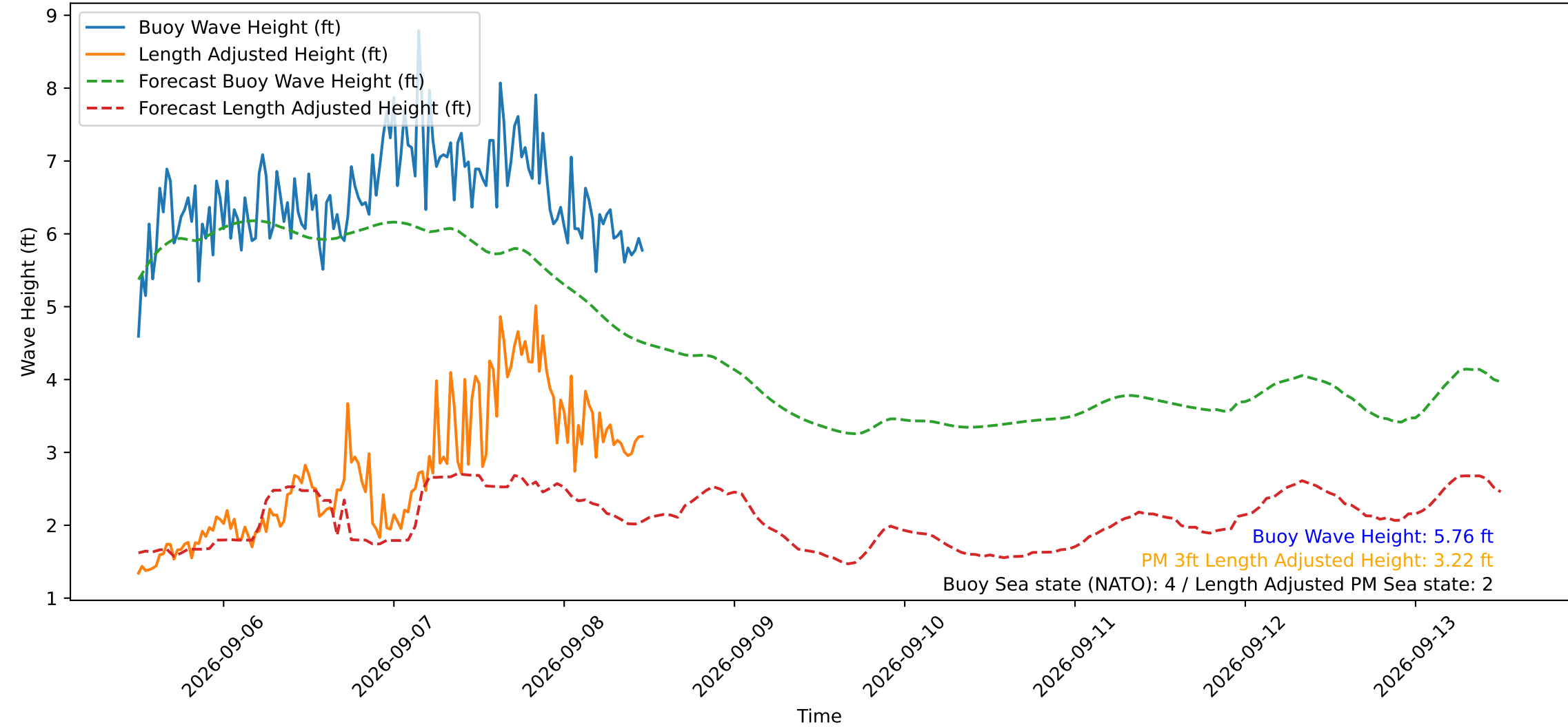
Wave Heights over Time for Green Beach at 2026-09-08 11:51:14
