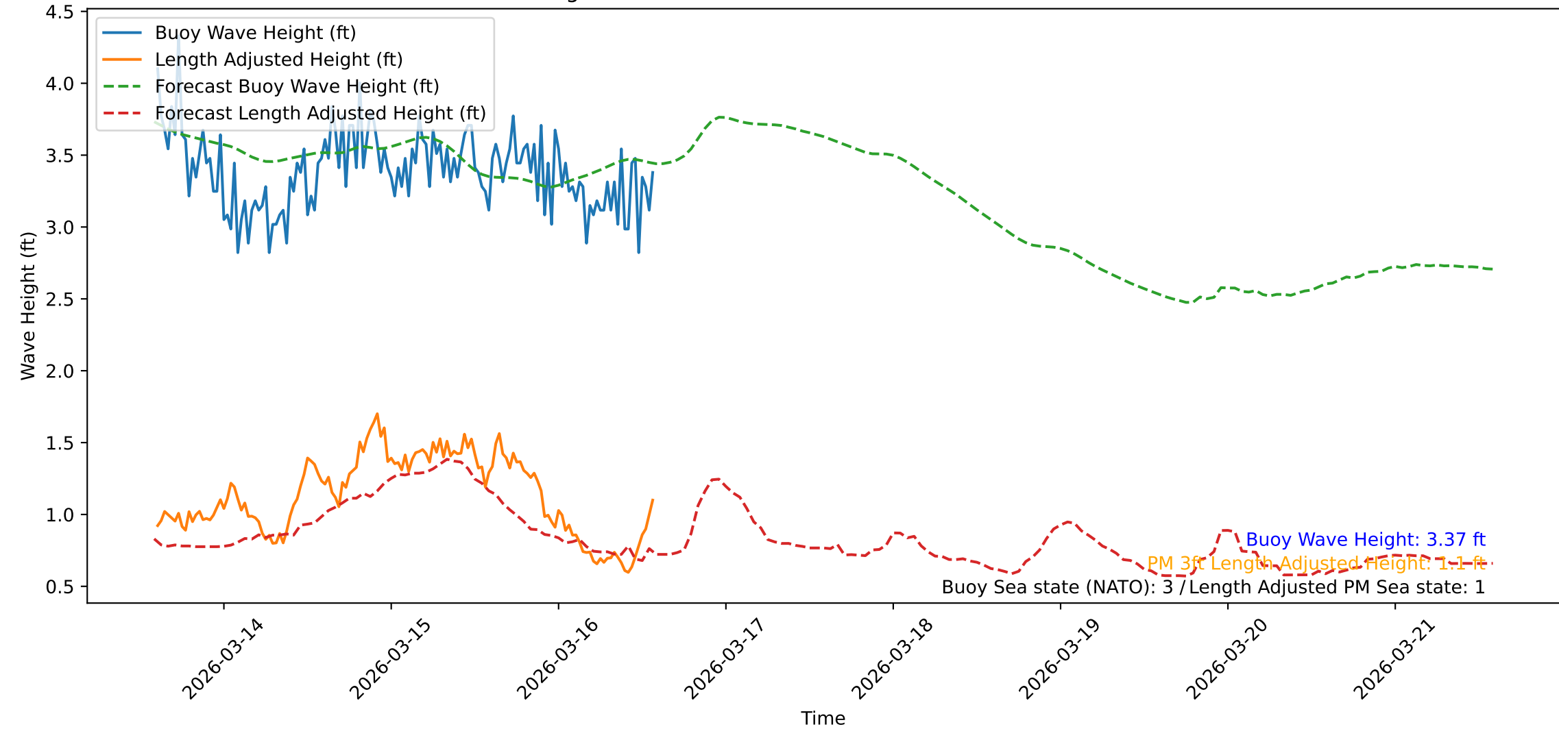
Wave Heights over Time for Green Beach at 2026-03-16 14:21:48
