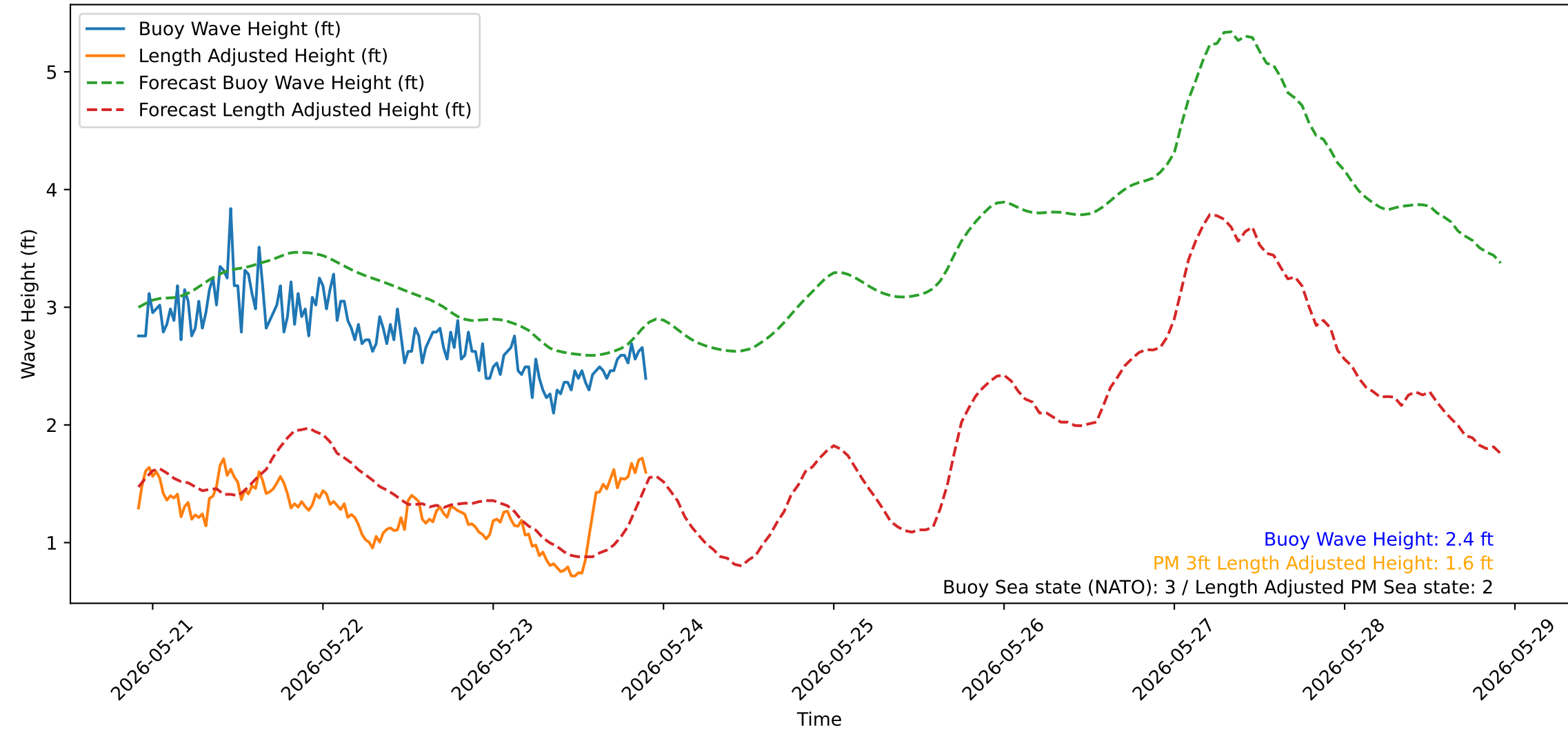
Wave Heights over Time for Oceanside Harbor at 2026-05-23 22:10:31
