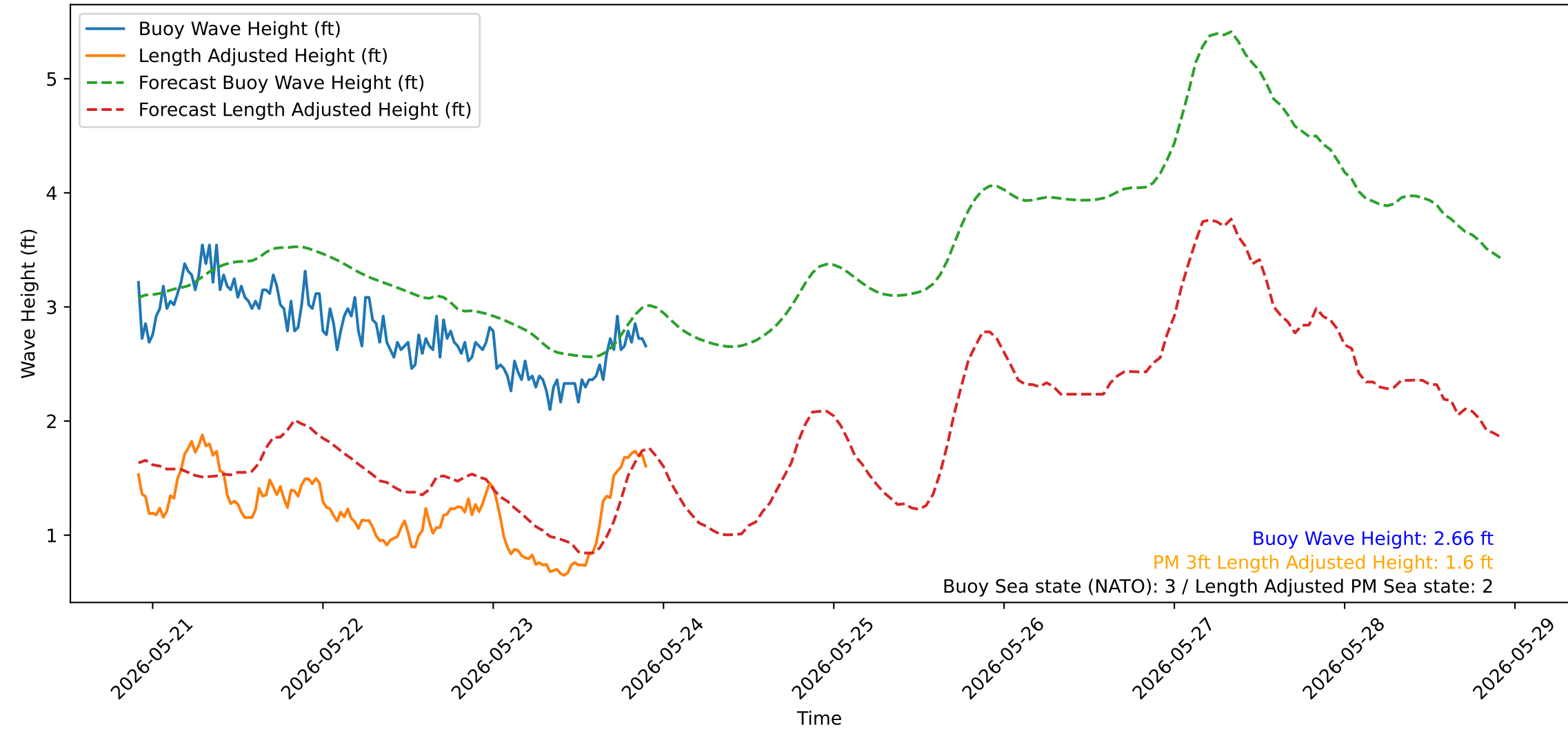
Wave Heights over Time for Green Beach at 2026-05-23 22:11:13
