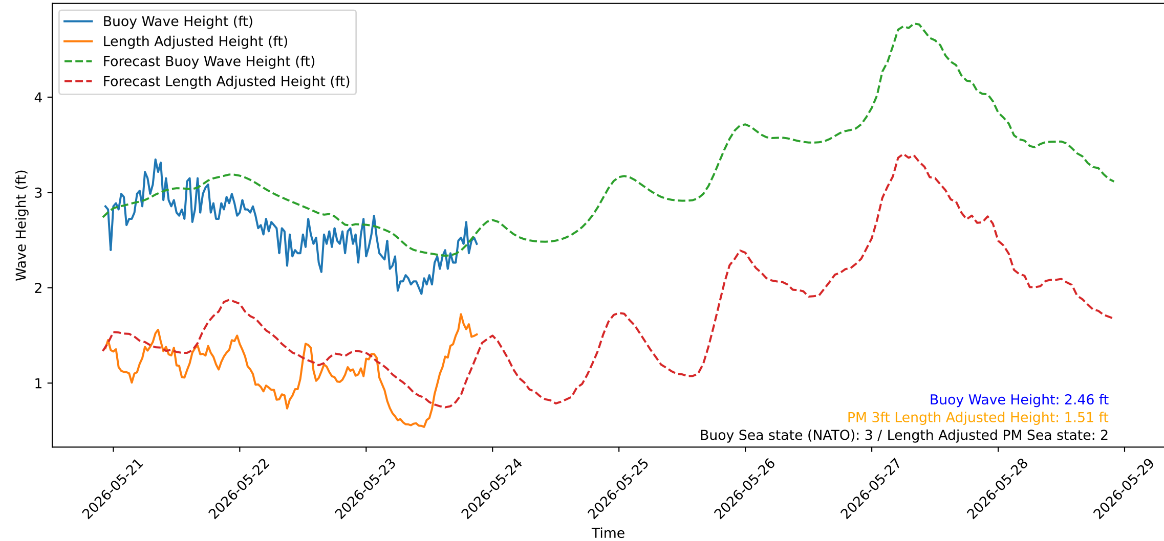
Wave Heights over Time for Red Beach at 2026-05-23 22:10:50
