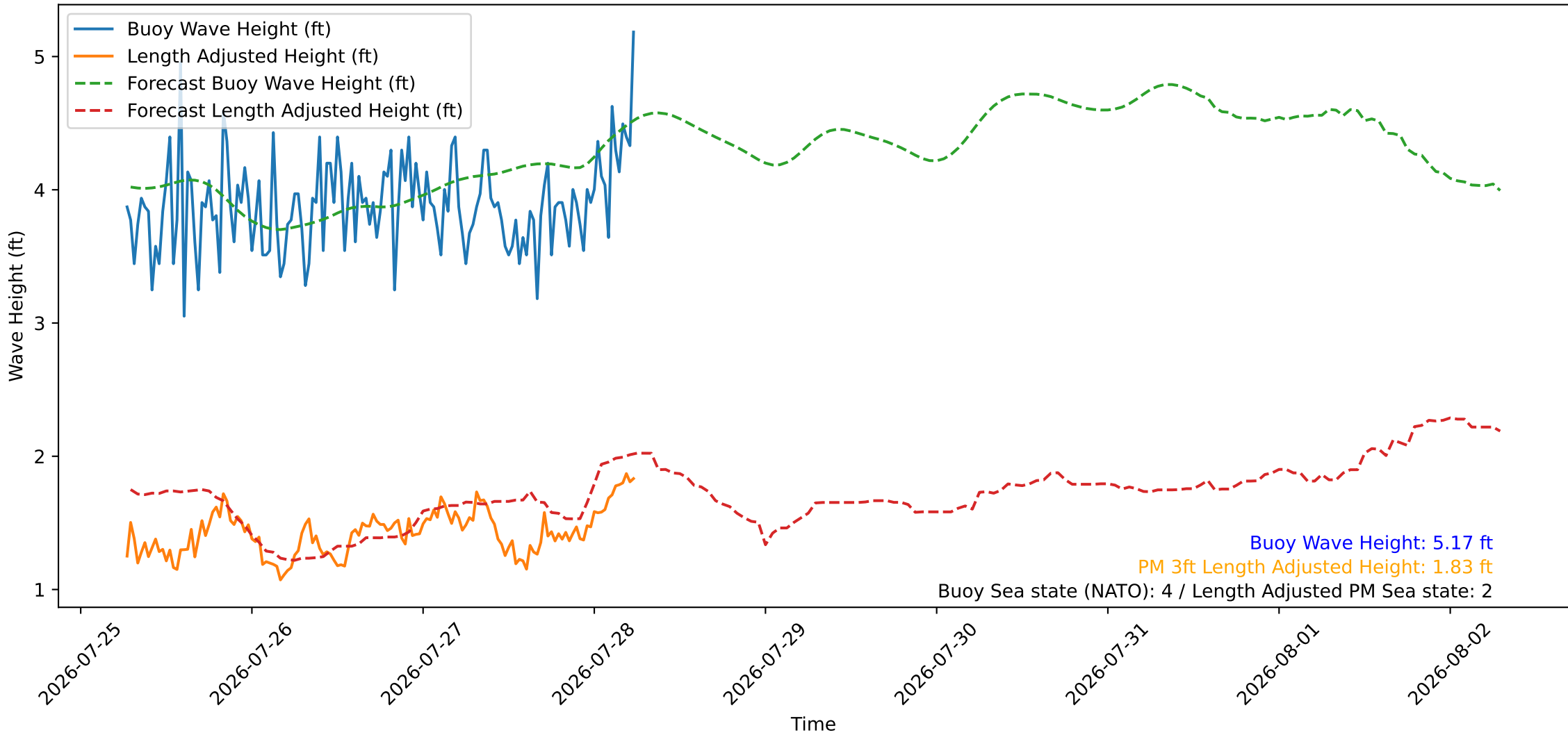
Wave Heights over Time for Oceanside Harbor at 2026-07-28 06:40:27
