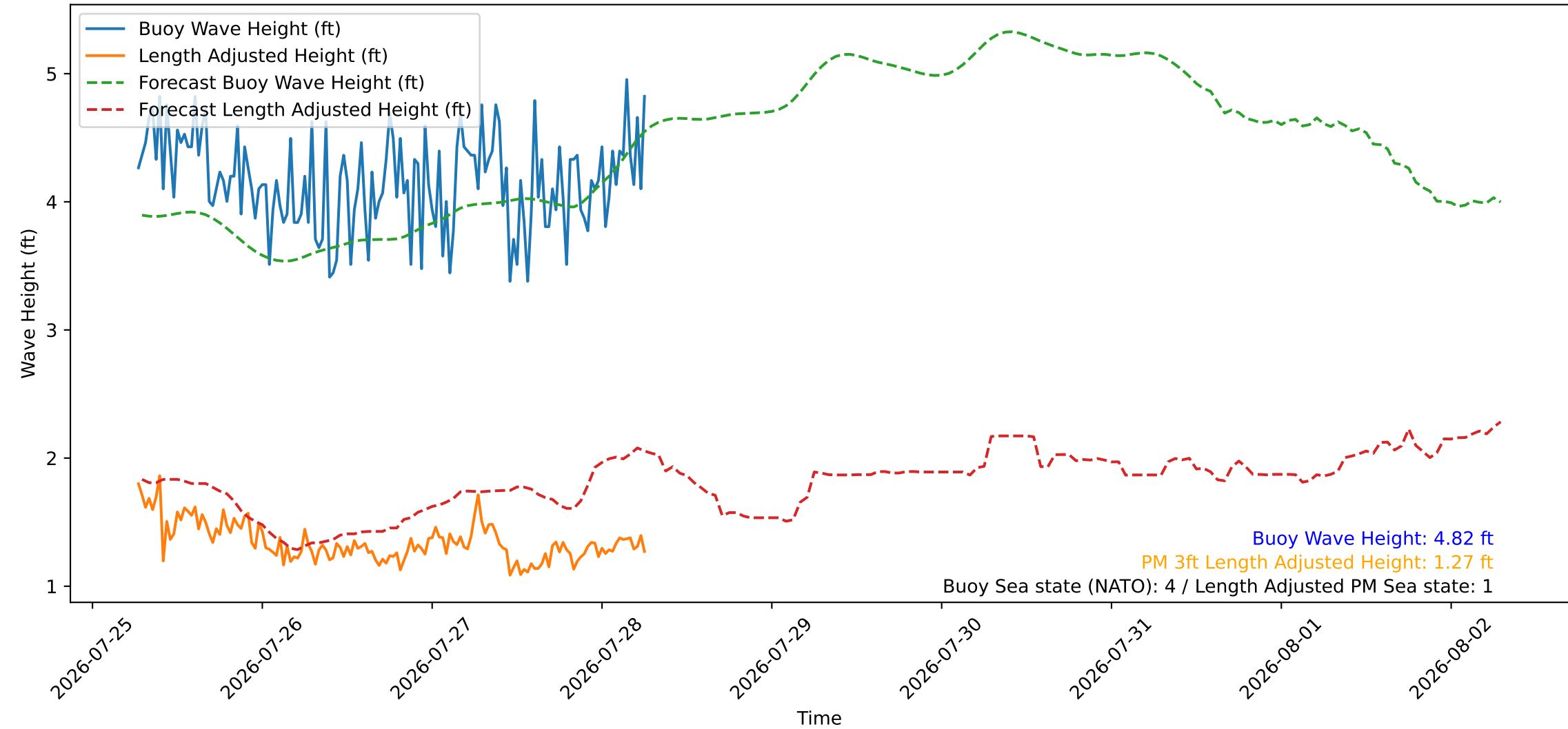
Wave Heights over Time for Green Beach at 2026-07-28 06:41:08
