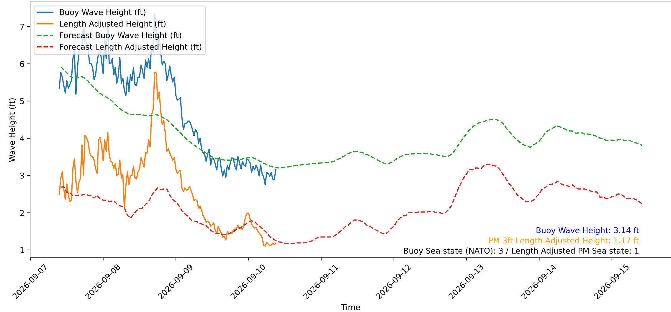
Wave Heights over Time for Oceanside Harbor at 2026-09-10 09:30:30
