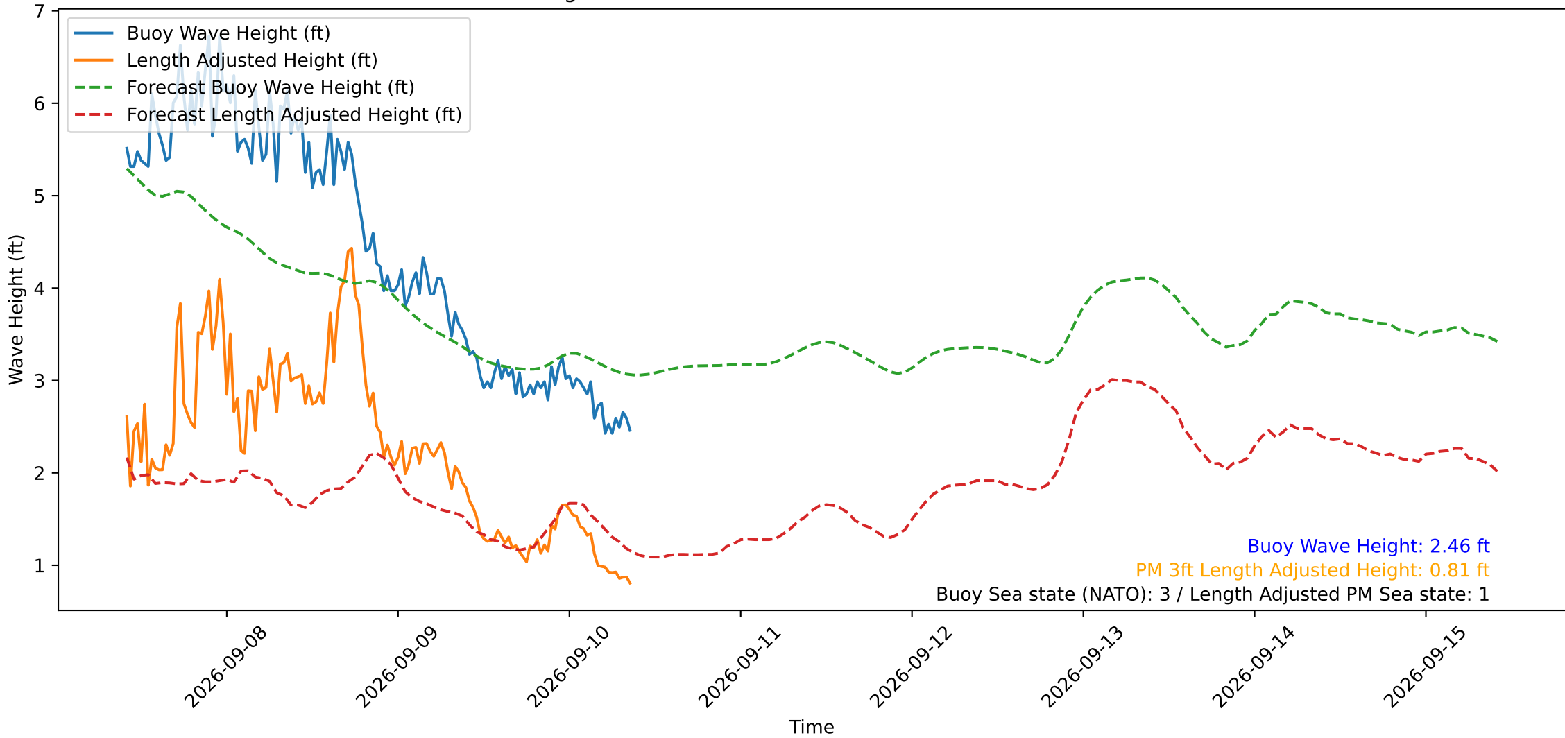
Wave Heights over Time for Red Beach at 2026-09-10 09:30:50
