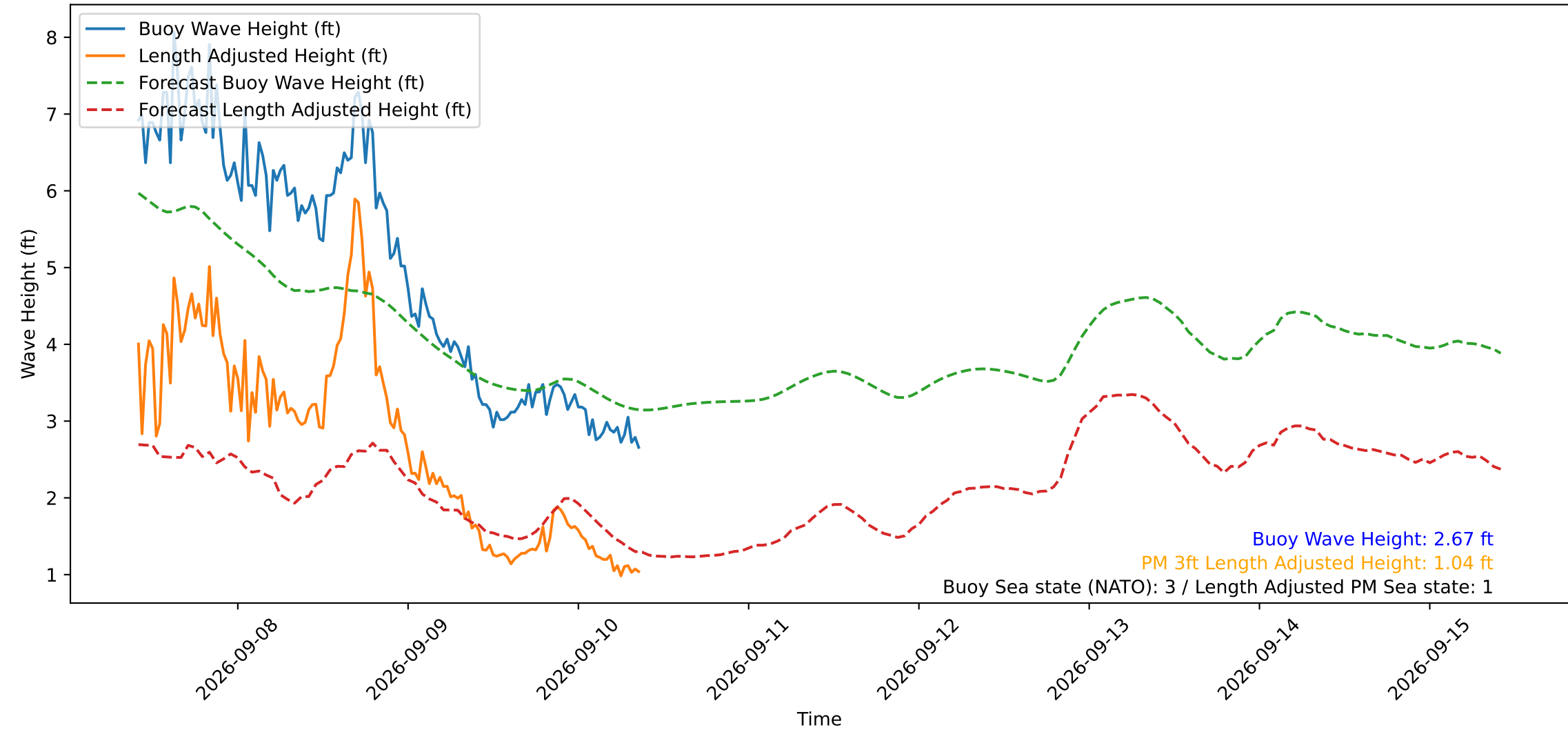
Wave Heights over Time for Green Beach at 2026-09-10 09:31:13
