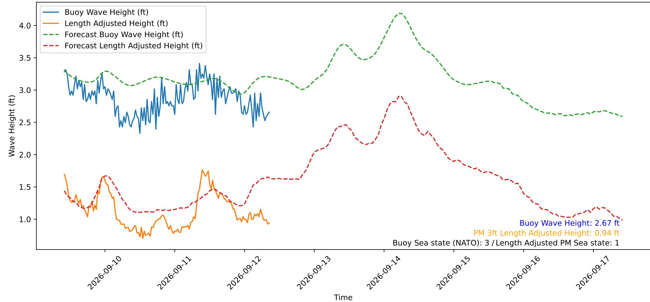
Wave Heights over Time for Red Beach at 2026-09-12 09:30:49
