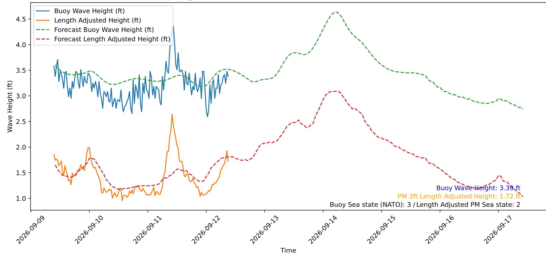
Wave Heights over Time for Oceanside Harbor at 2026-09-12 09:30:30
