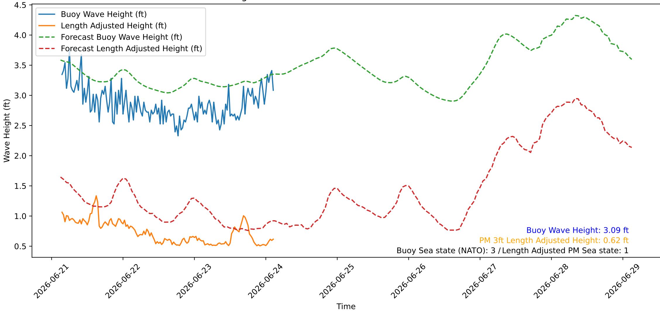
Wave Heights over Time for Red Beach at 2026-06-24 03:10:45
