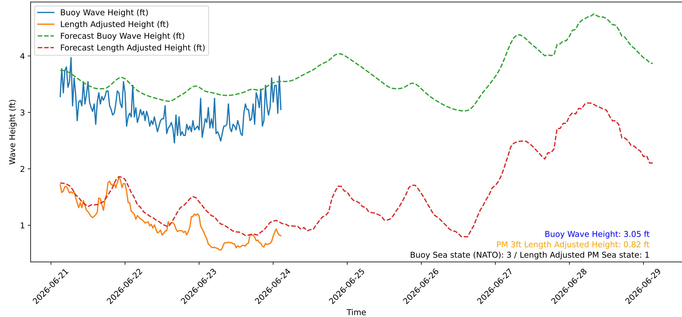
Wave Heights over Time for Green Beach at 2026-06-24 03:11:08
