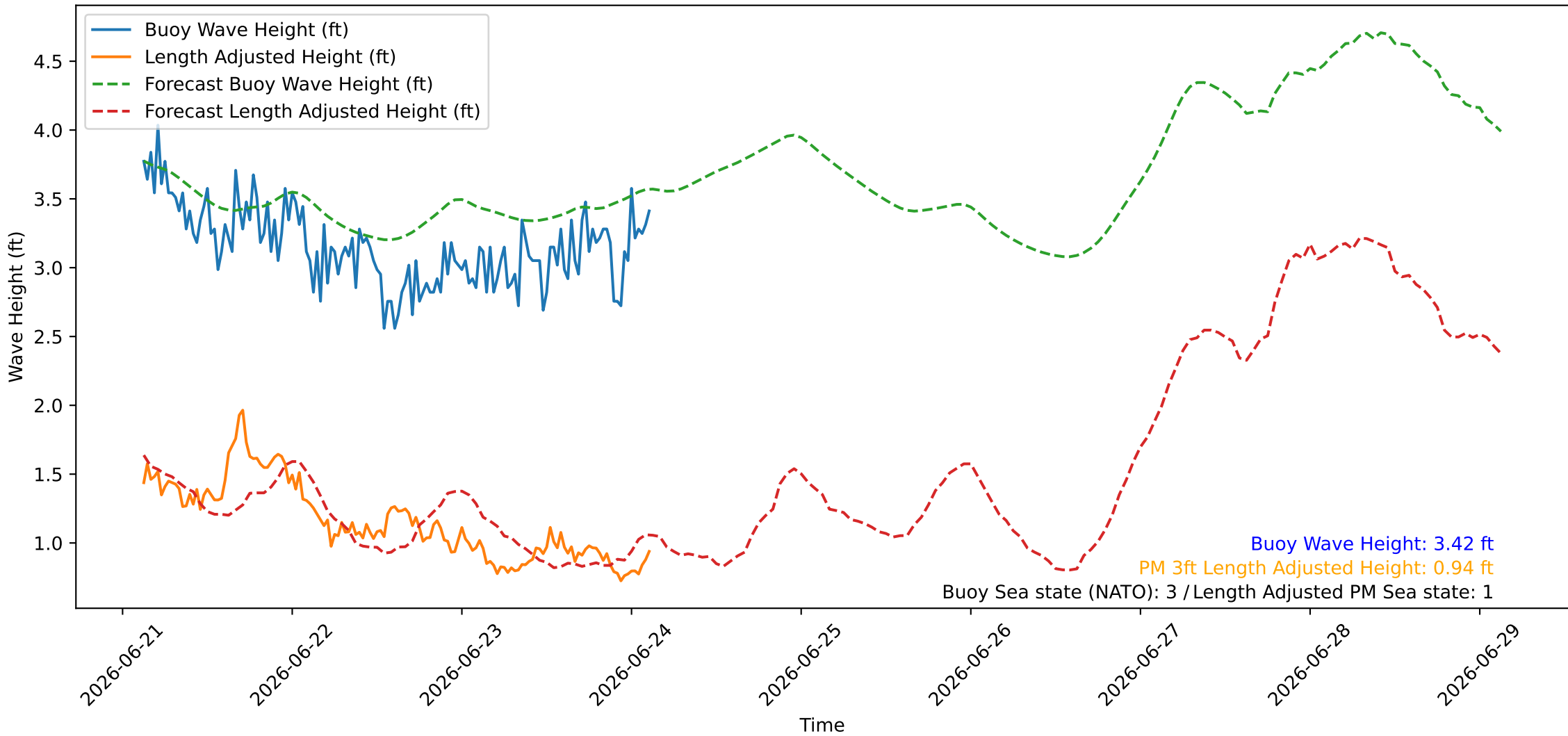
Wave Heights over Time for Oceanside Harbor at 2026-06-24 03:10:26
