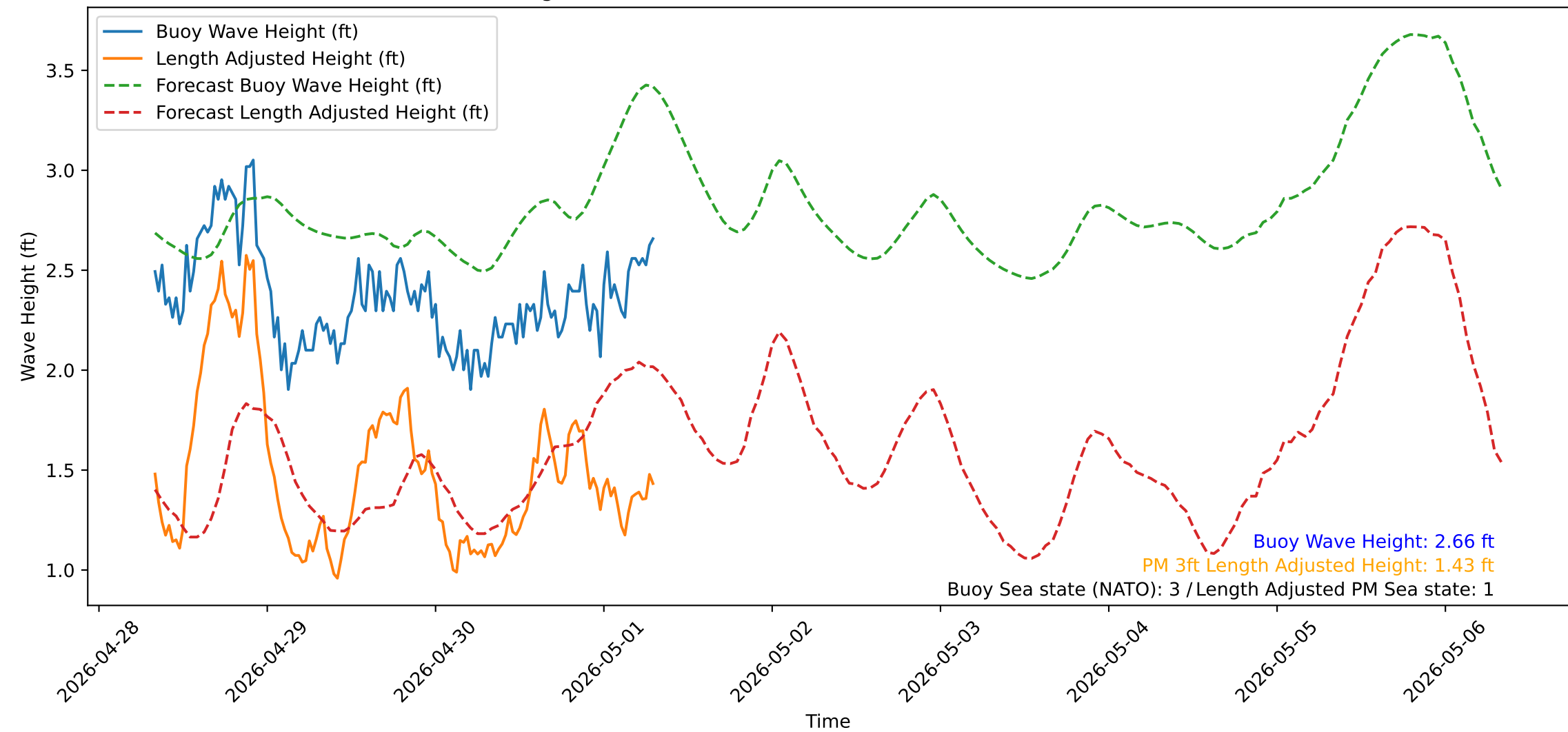
Wave Heights over Time for Oceanside Harbor at 2026-05-01 08:10:32
