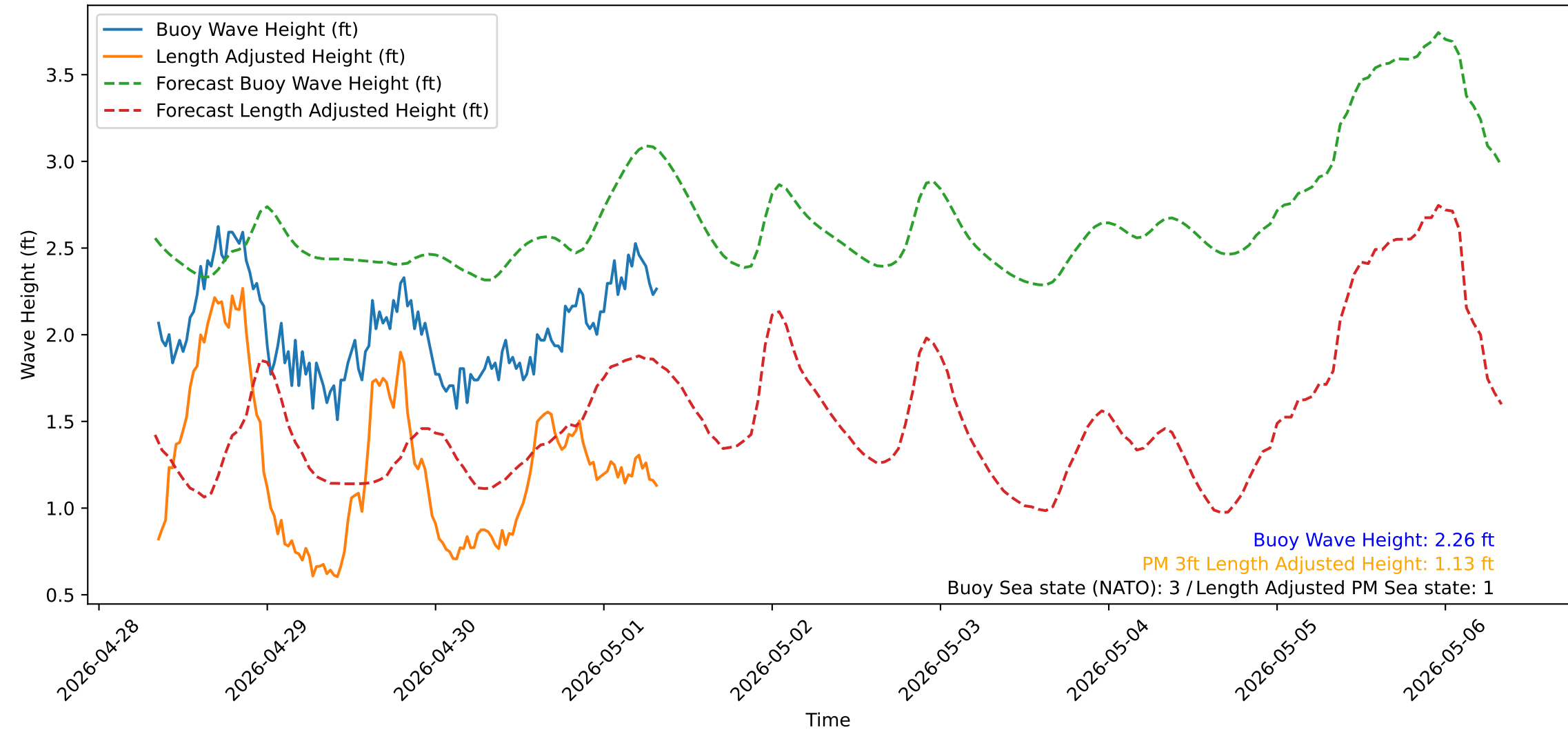
Wave Heights over Time for Red Beach at 2026-05-01 08:10:51
