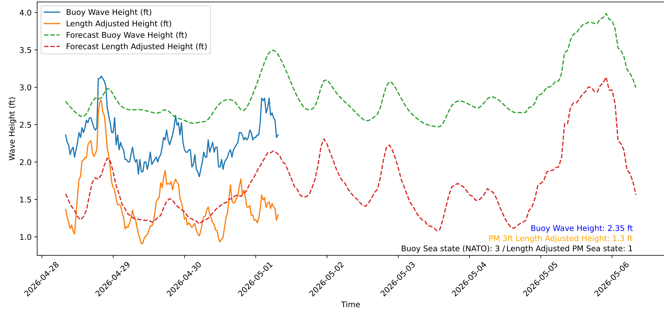
Wave Heights over Time for Green Beach at 2026-05-01 08:11:13
