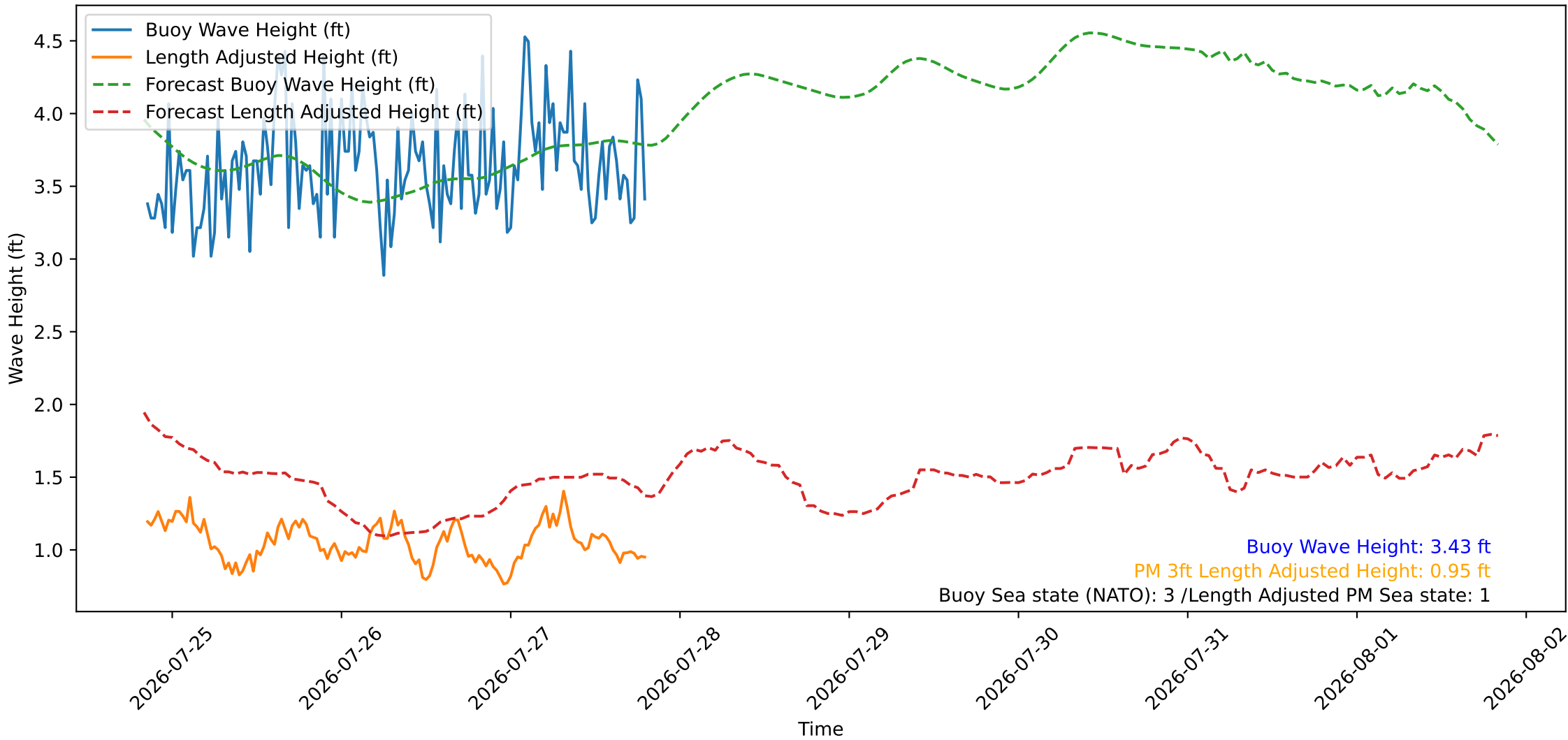
Wave Heights over Time for Red Beach at 2026-07-27 20:00:46
