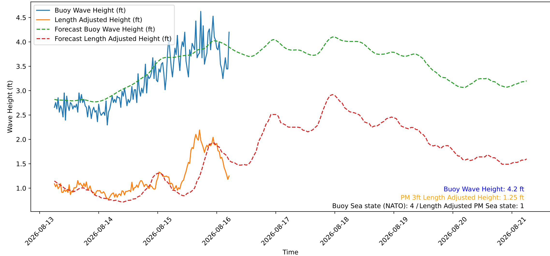
Wave Heights over Time for Oceanside Harbor at 2026-08-16 05:50:26
