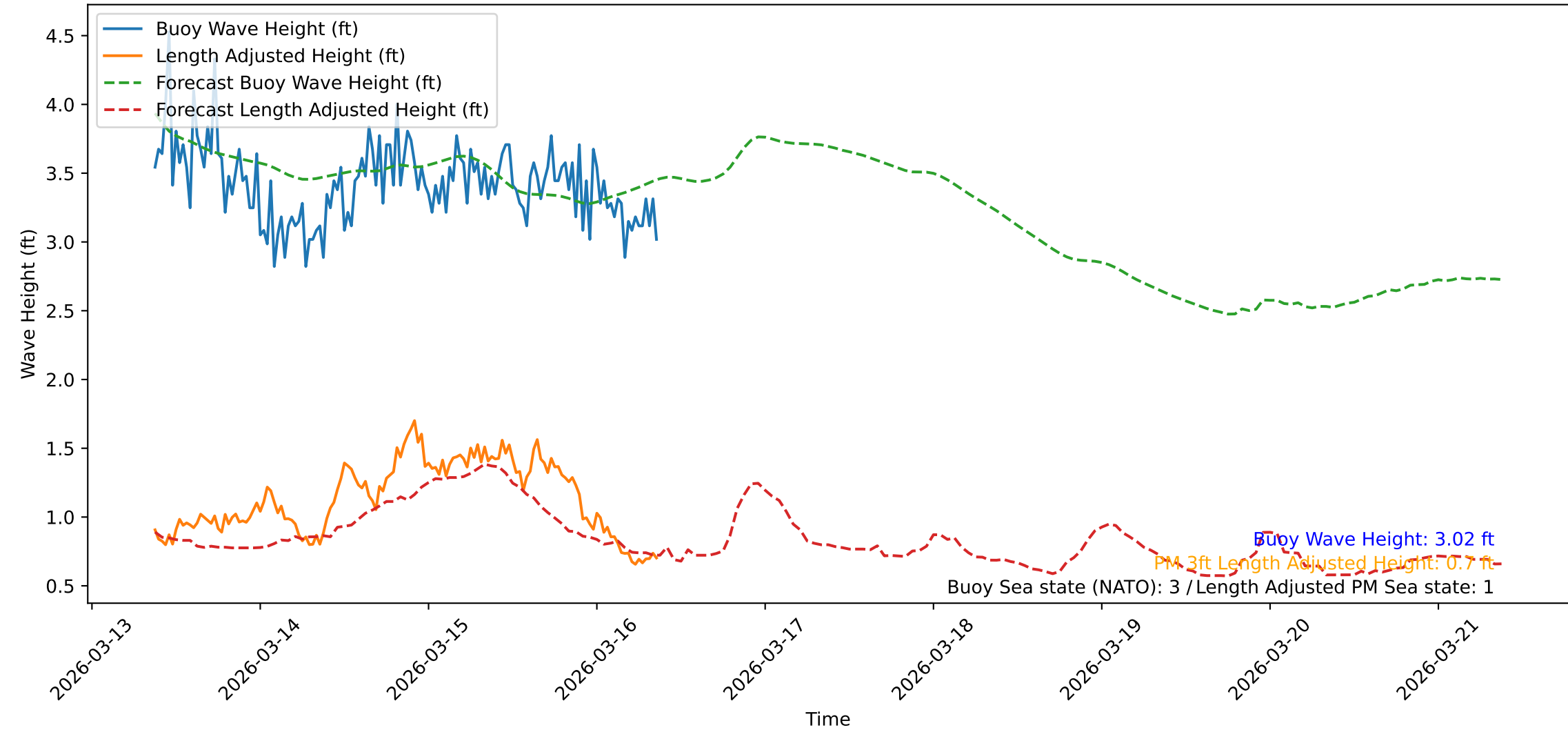
Wave Heights over Time for Green Beach at 2026-03-16 09:11:40
