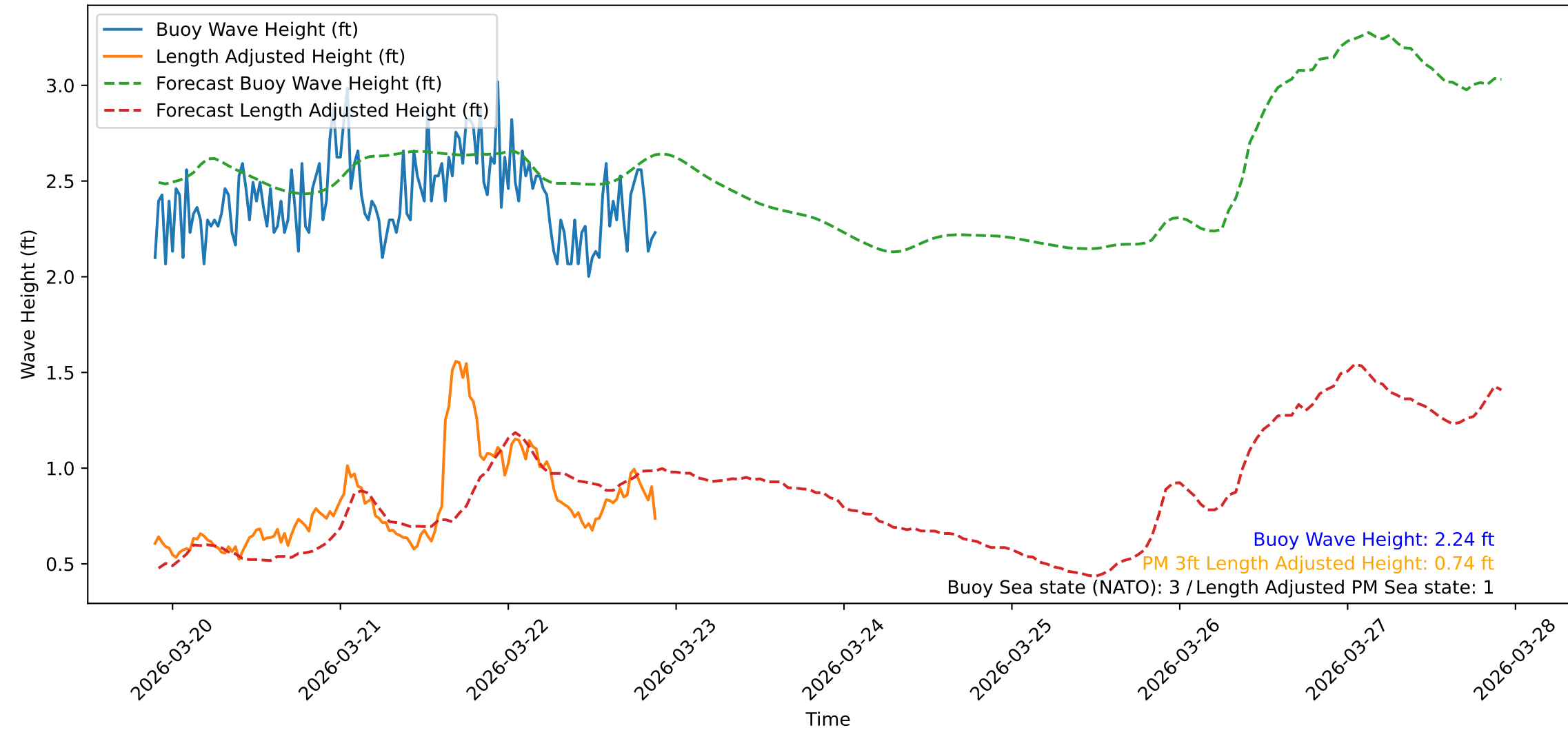
Wave Heights over Time for Oceanside Harbor at 2026-03-22 21:30:32
