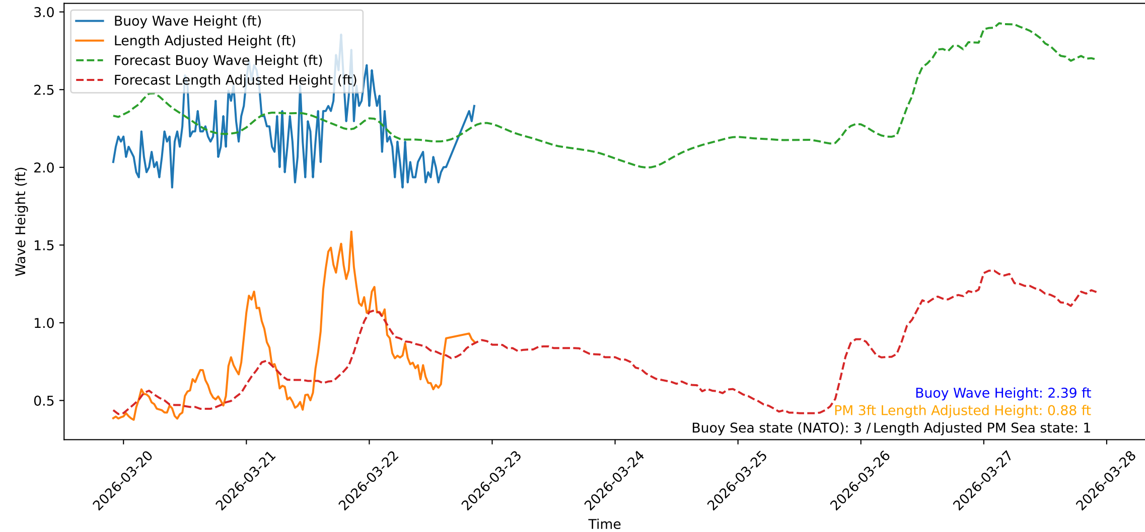
Wave Heights over Time for Red Beach at 2026-03-22 21:30:47
