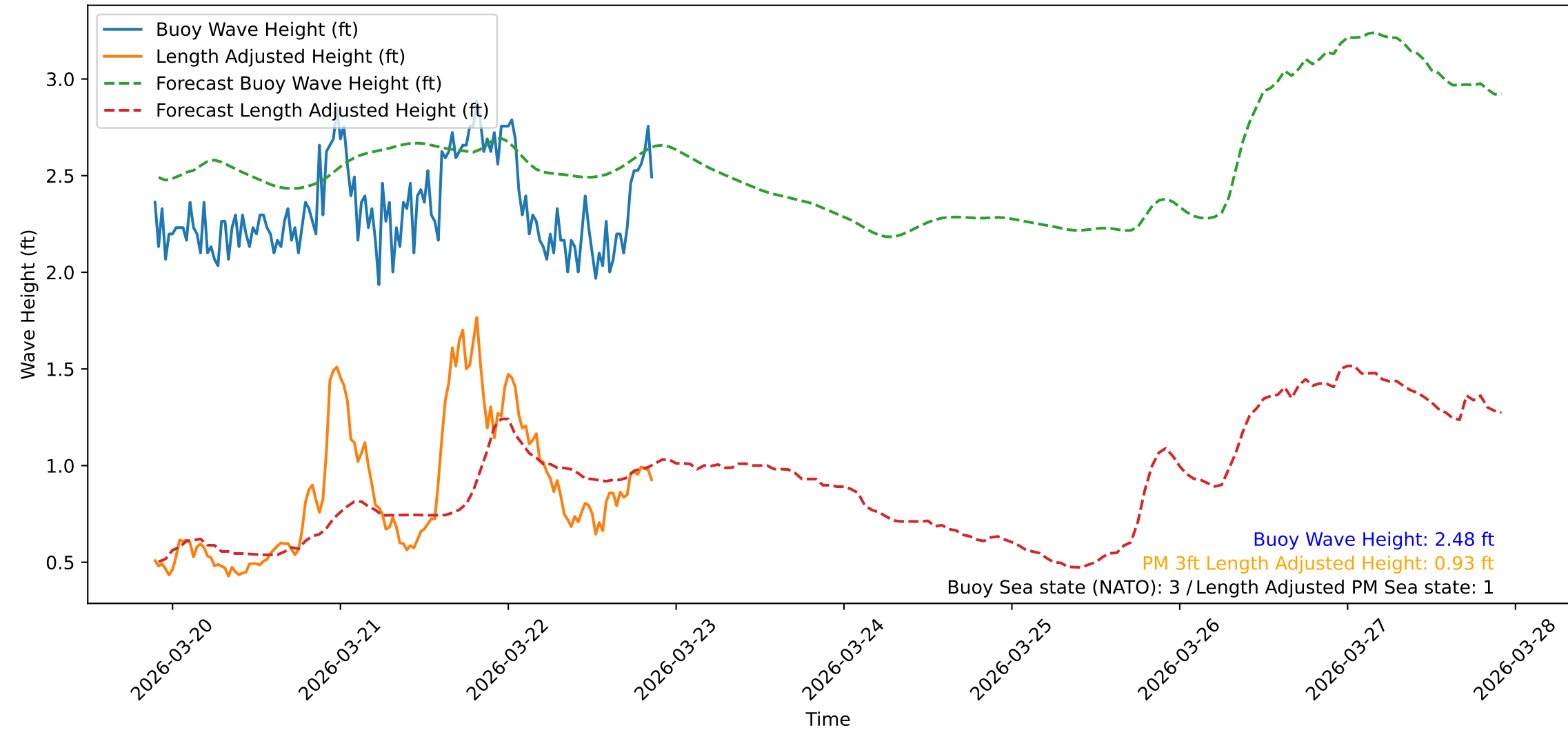
Wave Heights over Time for Green Beach at 2026-03-22 21:31:09
