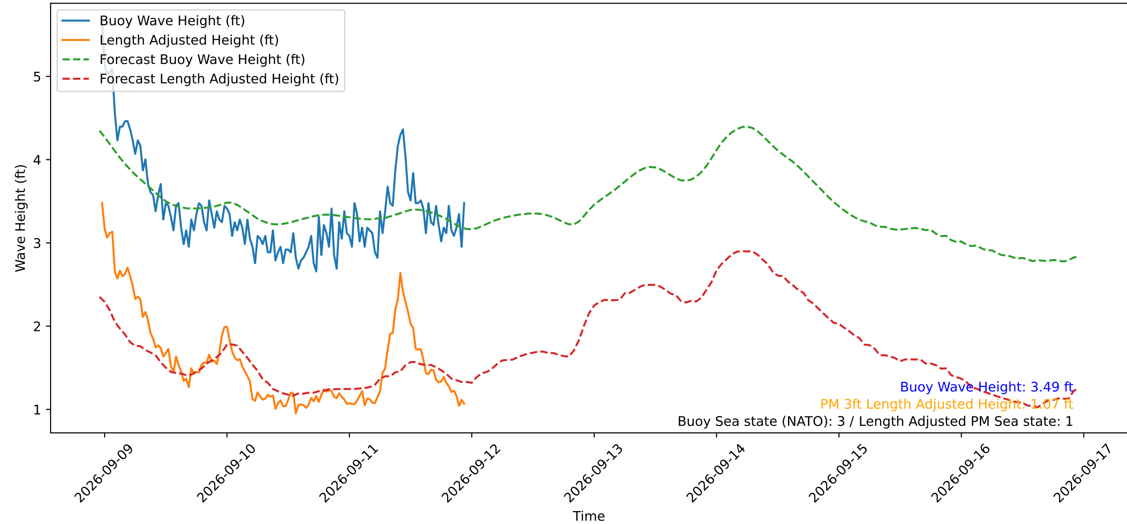
Wave Heights over Time for Oceanside Harbor at 2026-09-11 23:20:29
