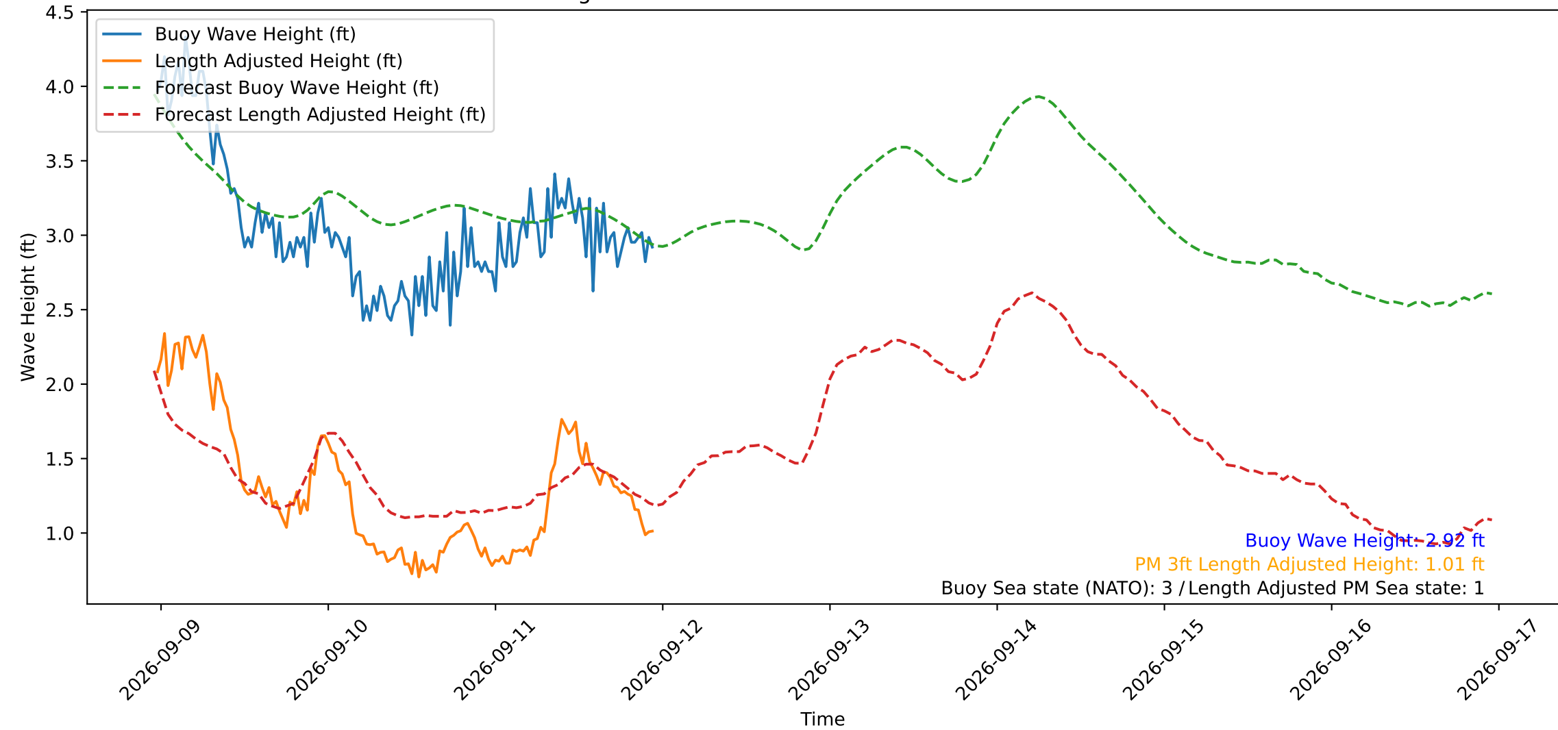
Wave Heights over Time for Red Beach at 2026-09-11 23:20:50
