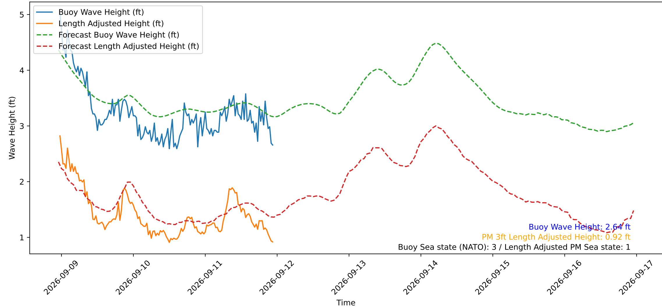
Wave Heights over Time for Green Beach at 2026-09-11 23:21:14
