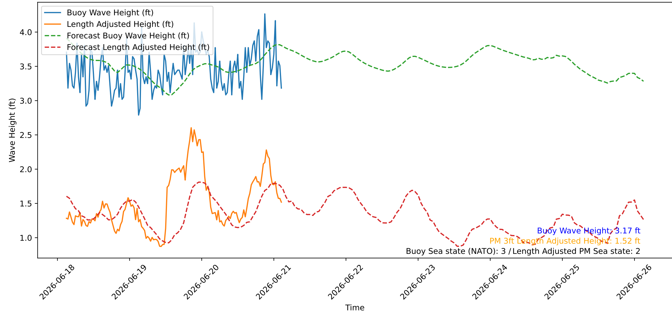
Wave Heights over Time for Oceanside Harbor at 2026-06-21 03:10:26
