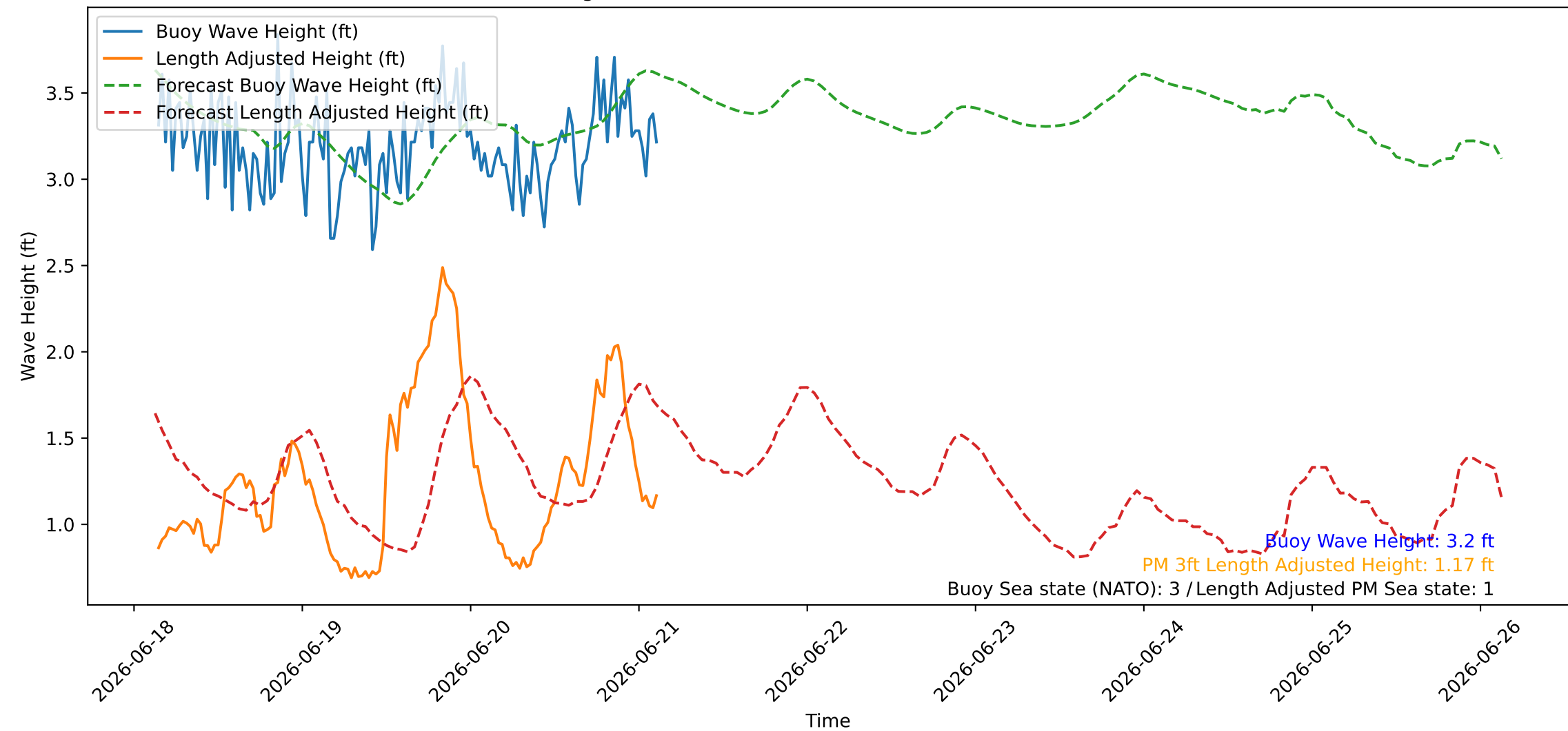
Wave Heights over Time for Red Beach at 2026-06-21 03:10:45
