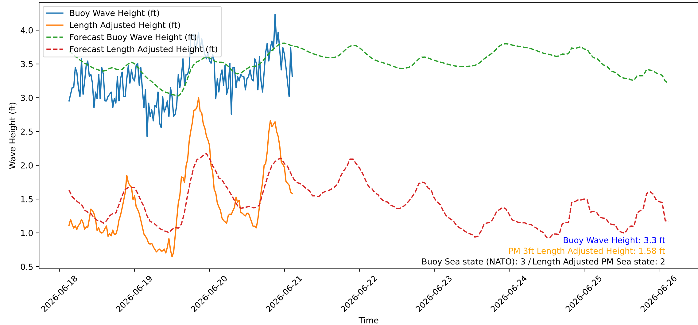
Wave Heights over Time for Green Beach at 2026-06-21 03:11:08
