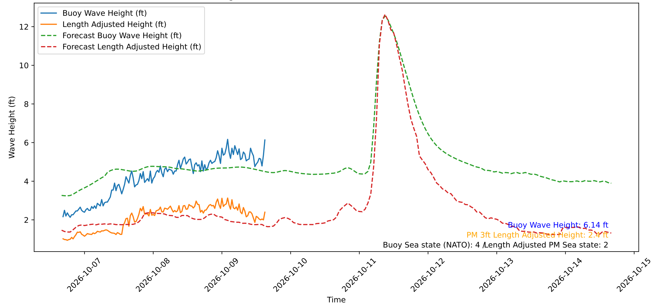
Wave Heights over Time for Green Beach at 2026-10-09 16:01:12
