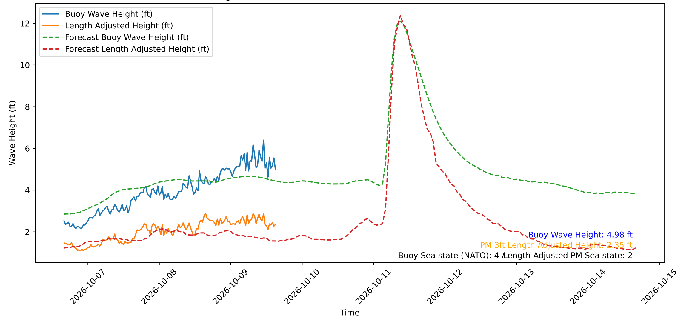
Wave Heights over Time for Oceanside Harbor at 2026-10-09 16:00:30
