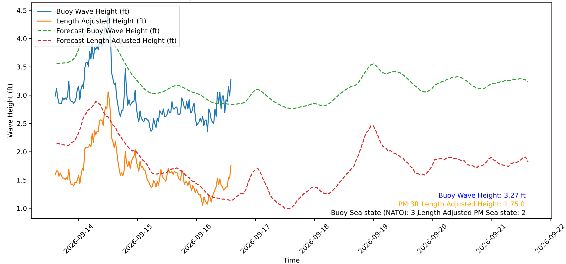
Wave Heights over Time for Oceanside Harbor at 2026-09-16 14:40:29
