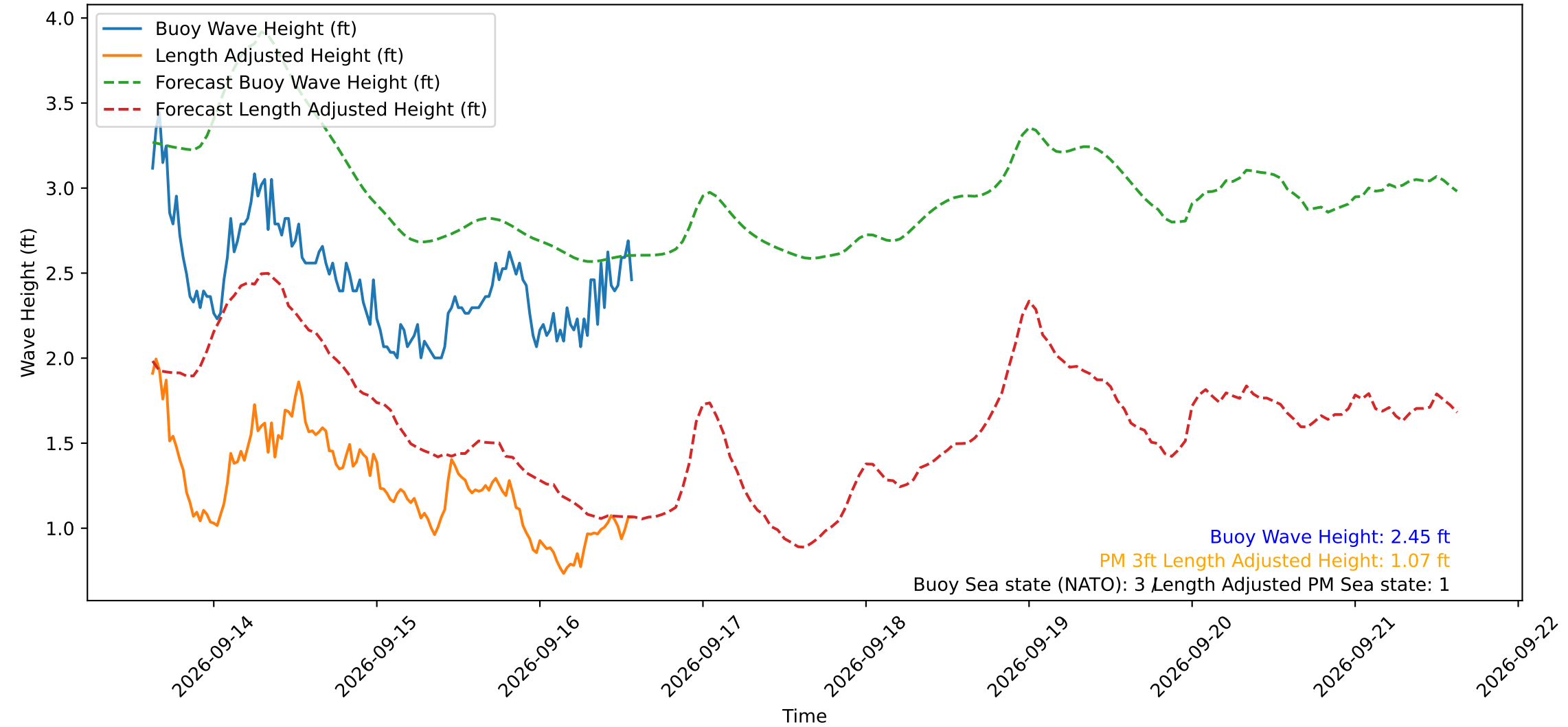
Wave Heights over Time for Red Beach at 2026-09-16 14:40:49
