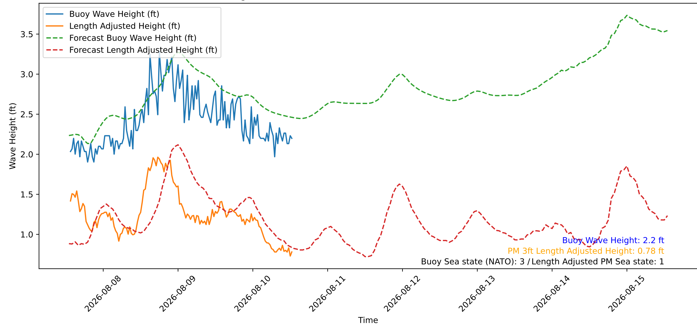
Wave Heights over Time for Oceanside Harbor at 2026-08-10 13:20:27
