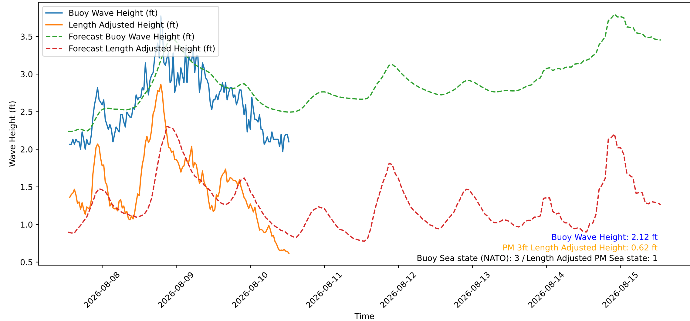
Wave Heights over Time for Green Beach at 2026-08-10 13:21:10
