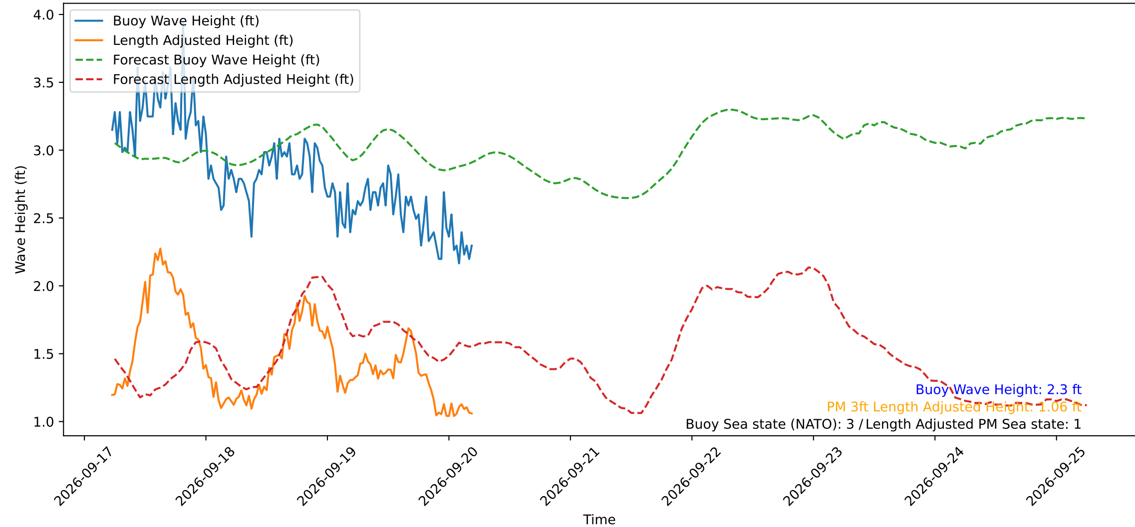
Wave Heights over Time for Oceanside Harbor at 2026-09-20 05:30:29
