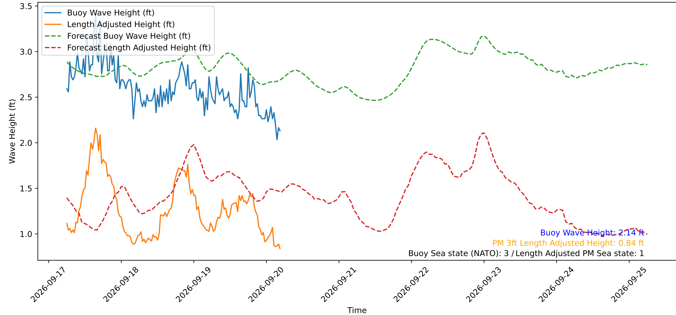
Wave Heights over Time for Red Beach at 2026-09-20 05:30:48
