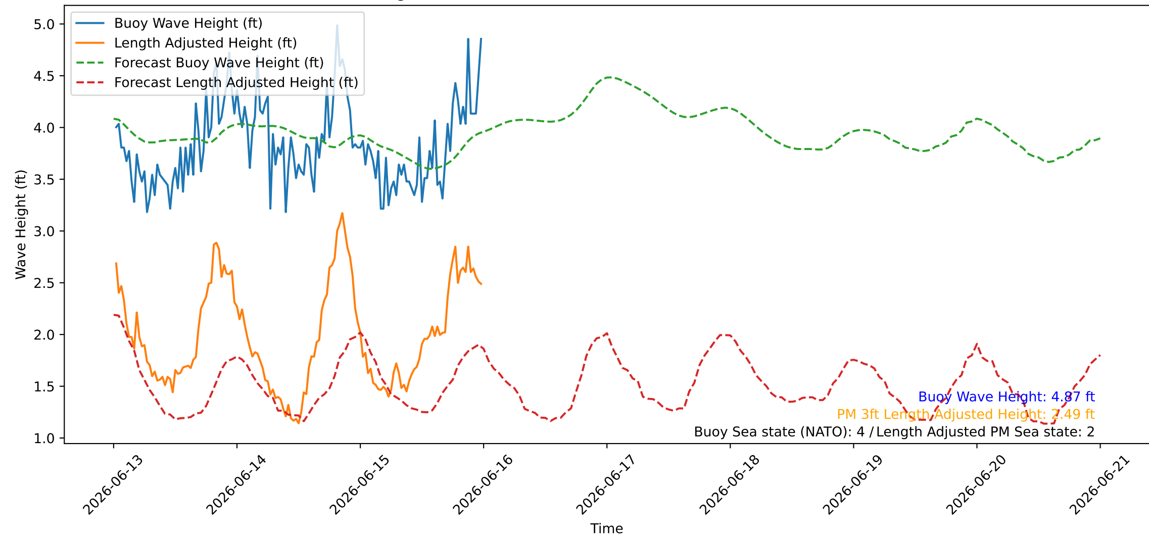
Wave Heights over Time for Oceanside Harbor at 2026-06-16 00:20:26
