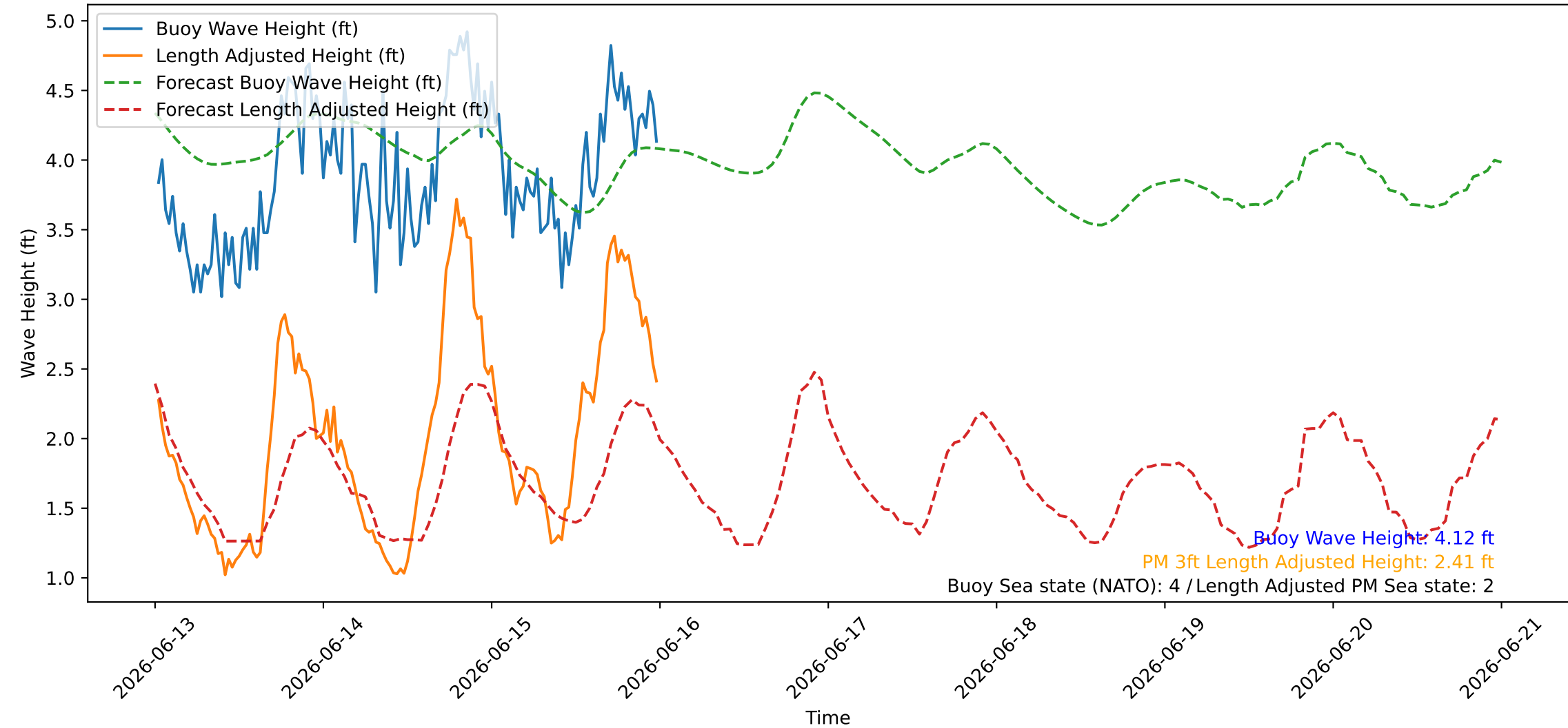
Wave Heights over Time for Green Beach at 2026-06-16 00:21:08
