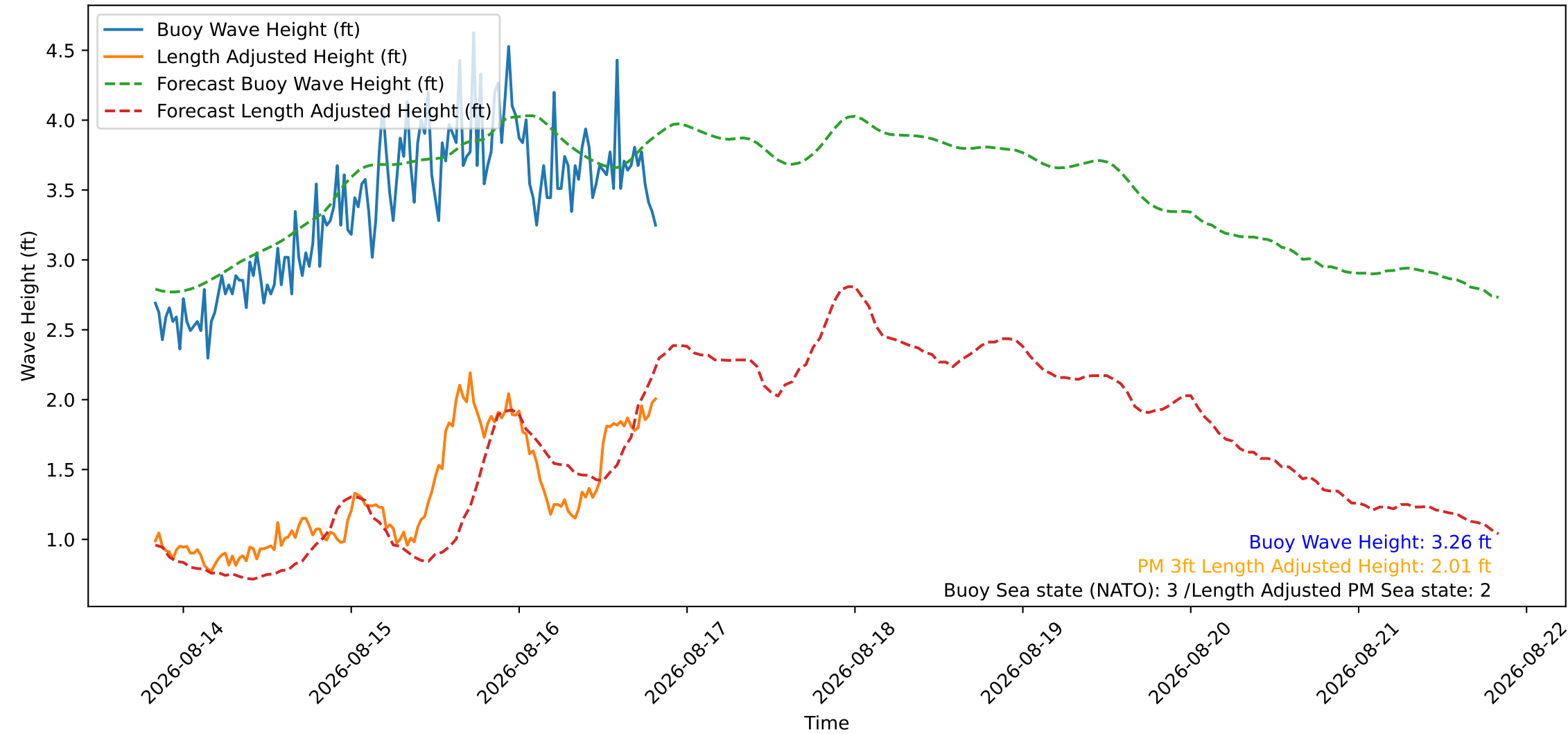
Wave Heights over Time for Oceanside Harbor at 2026-08-16 20:10:26
