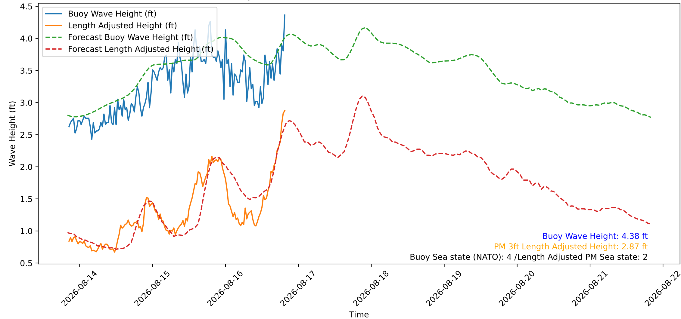
Wave Heights over Time for Green Beach at 2026-08-16 20:11:09
