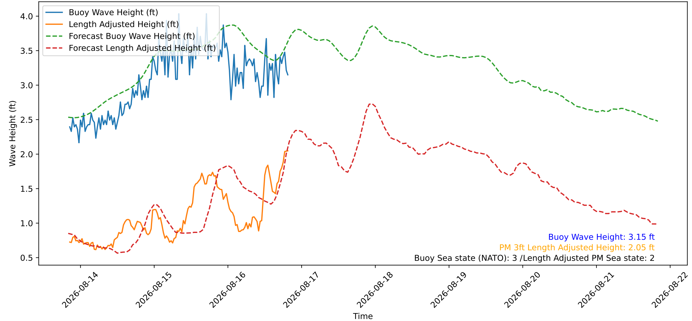
Wave Heights over Time for Red Beach at 2026-08-16 20:10:46
