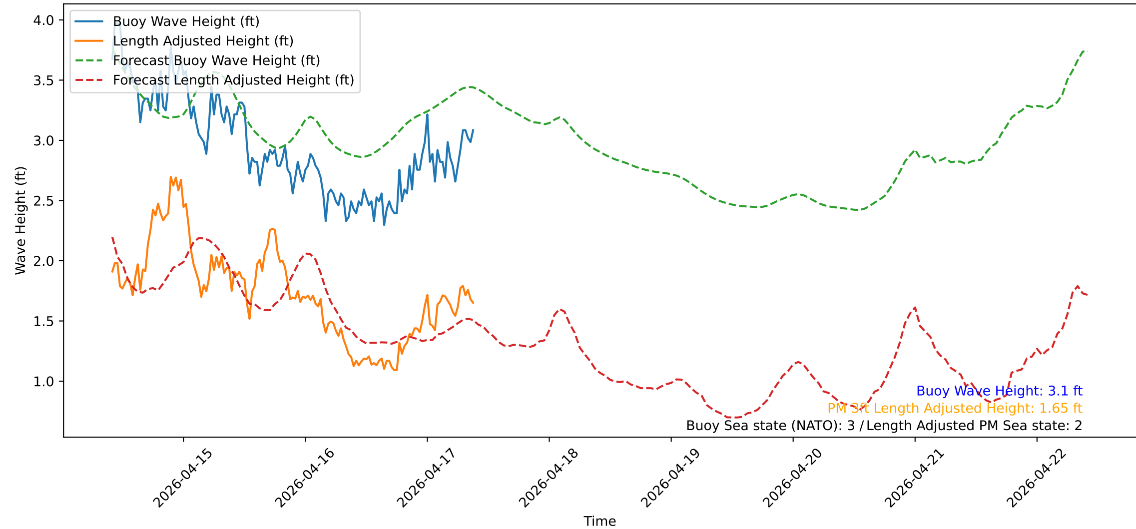
Wave Heights over Time for Oceanside Harbor at 2026-04-17 09:50:33
