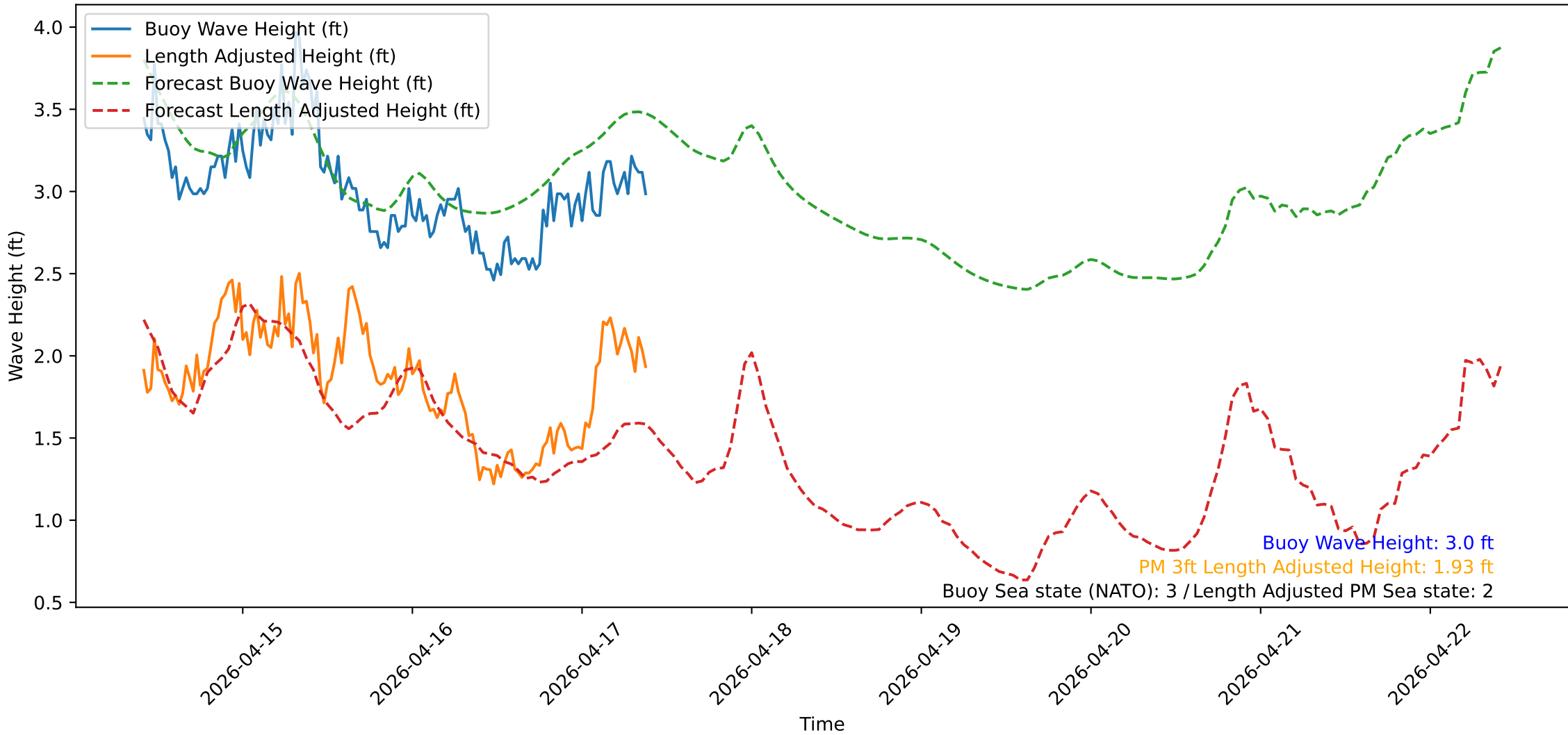
Wave Heights over Time for Green Beach at 2026-04-17 09:51:16
