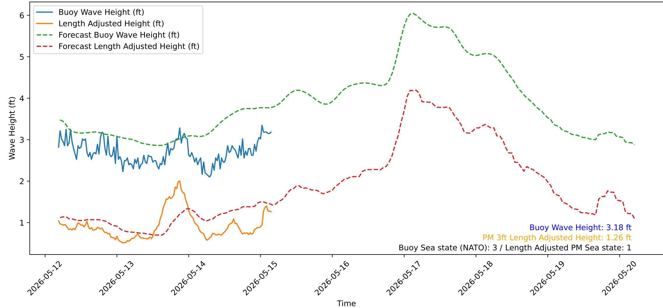
Wave Heights over Time for Green Beach at 2026-05-15 04:31:14
