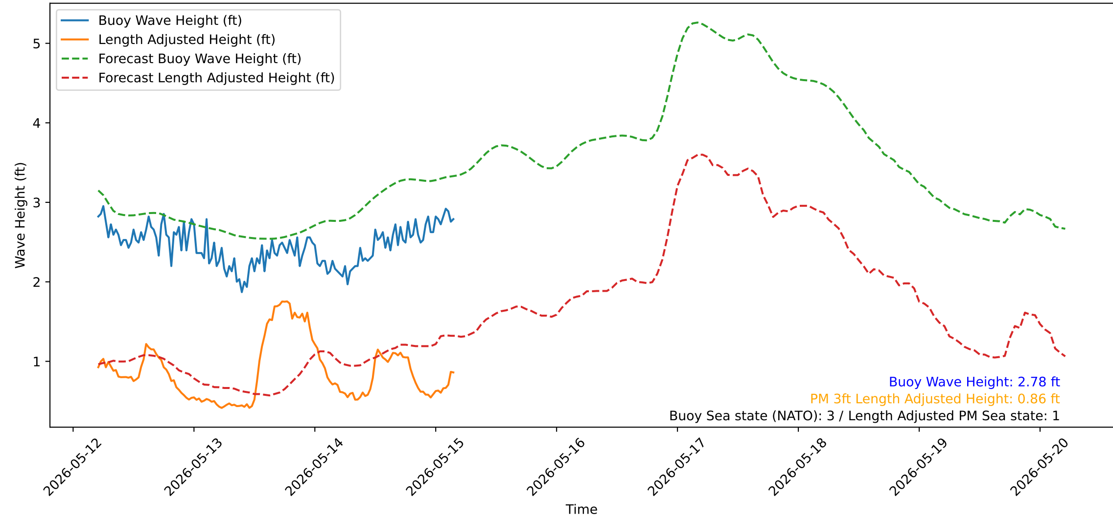
Wave Heights over Time for Red Beach at 2026-05-15 04:30:51
