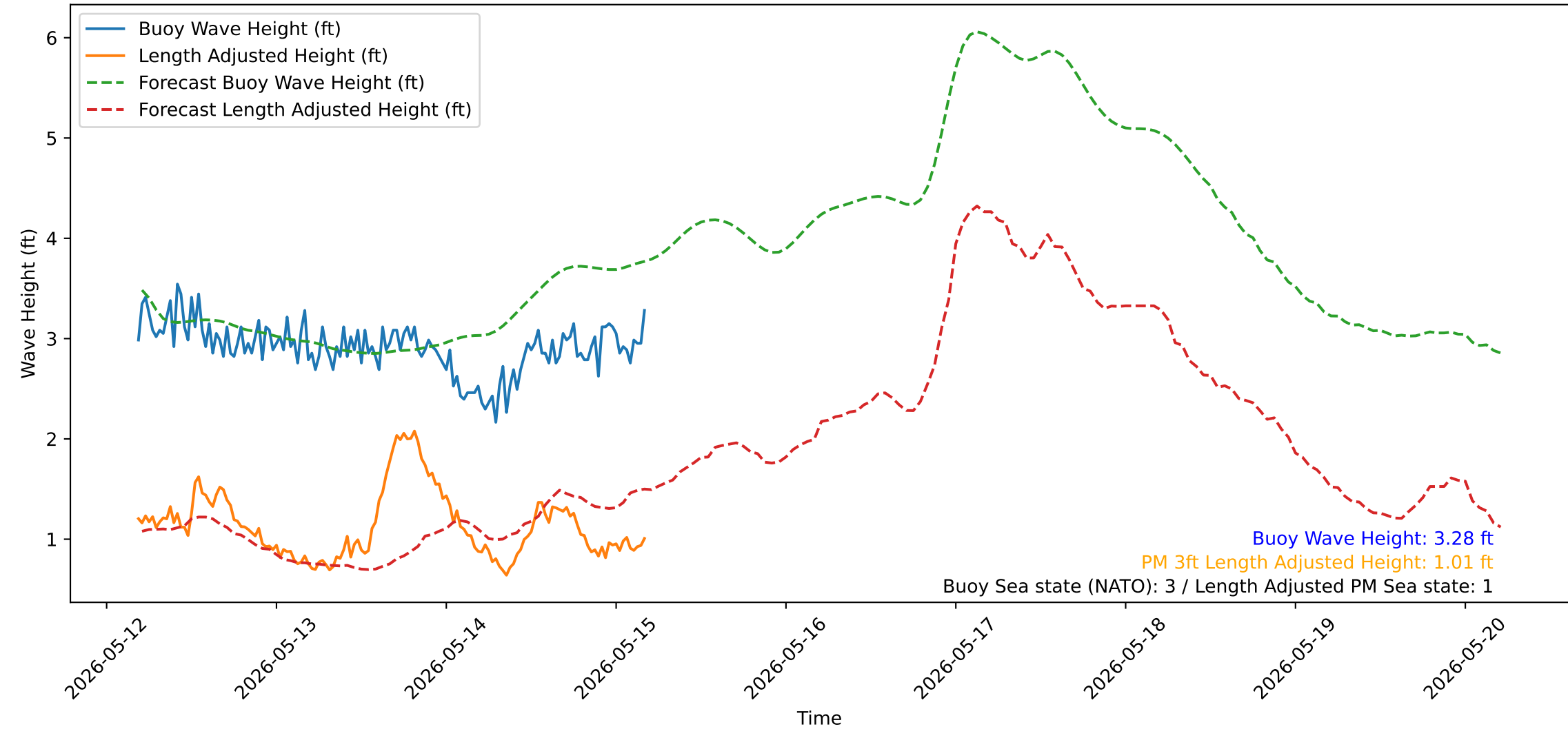
Wave Heights over Time for Oceanside Harbor at 2026-05-15 04:30:32
