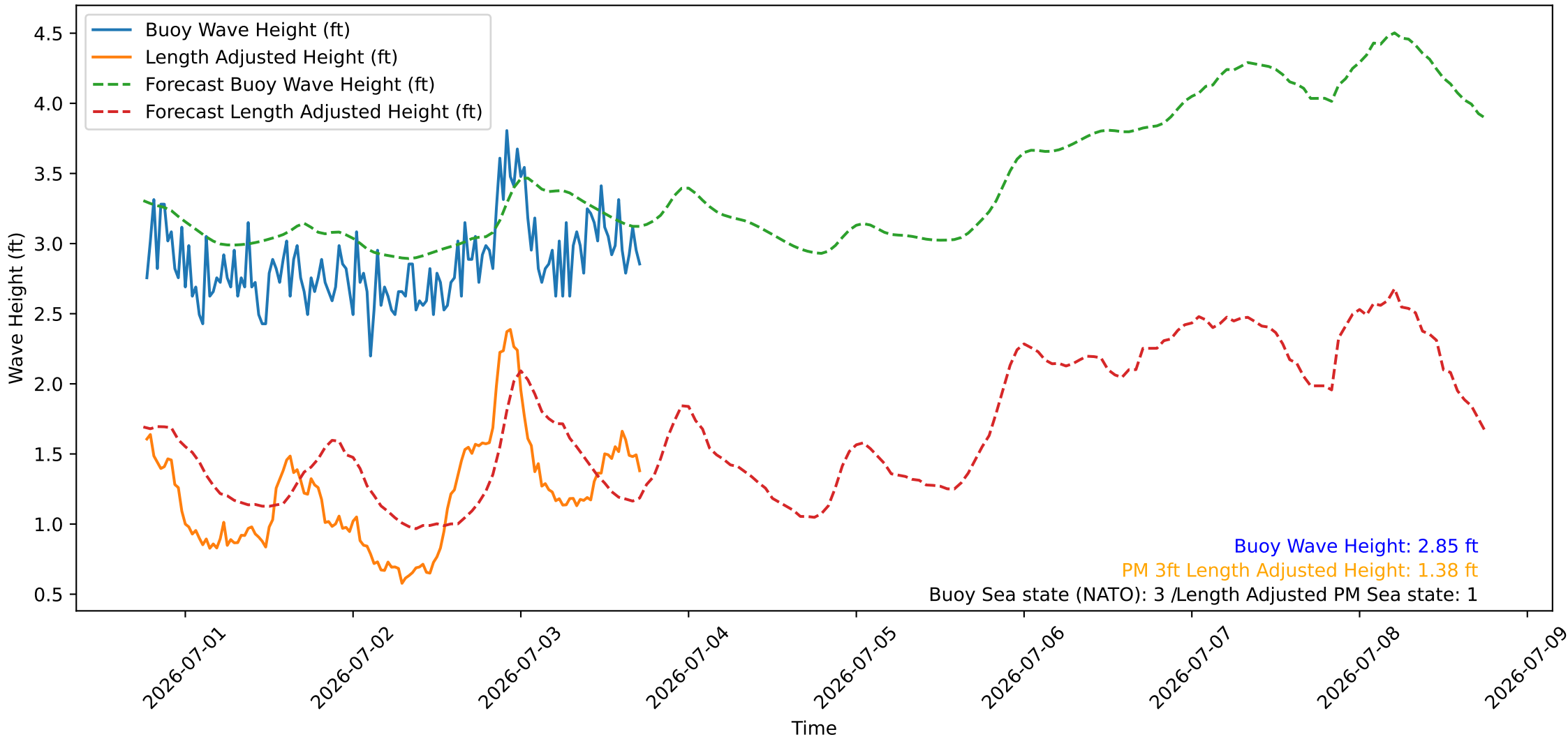
Wave Heights over Time for Red Beach at 2026-07-03 18:10:46
