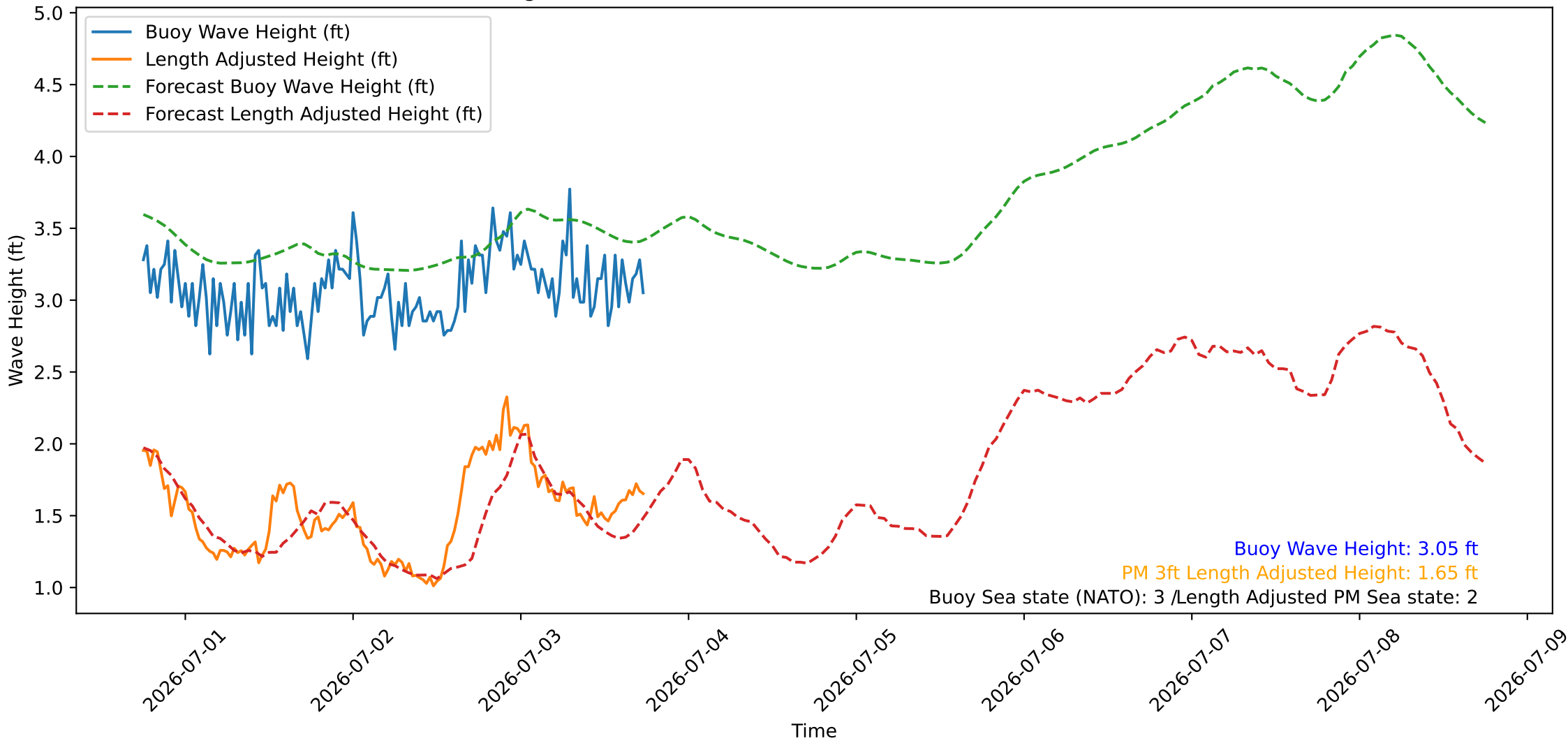
Wave Heights over Time for Oceanside Harbor at 2026-07-03 18:10:26
