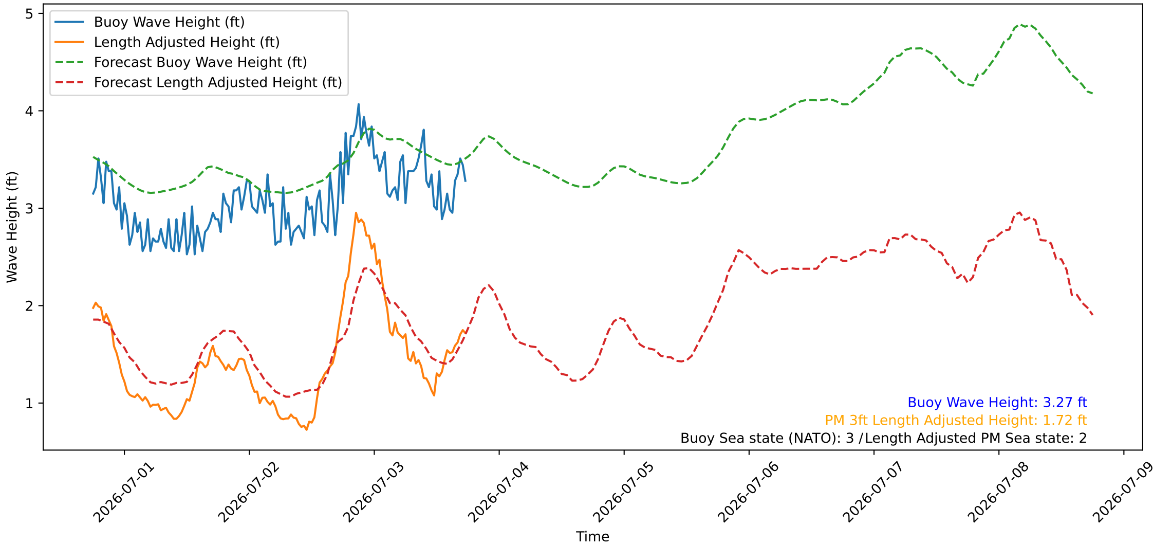
Wave Heights over Time for Green Beach at 2026-07-03 18:11:08
