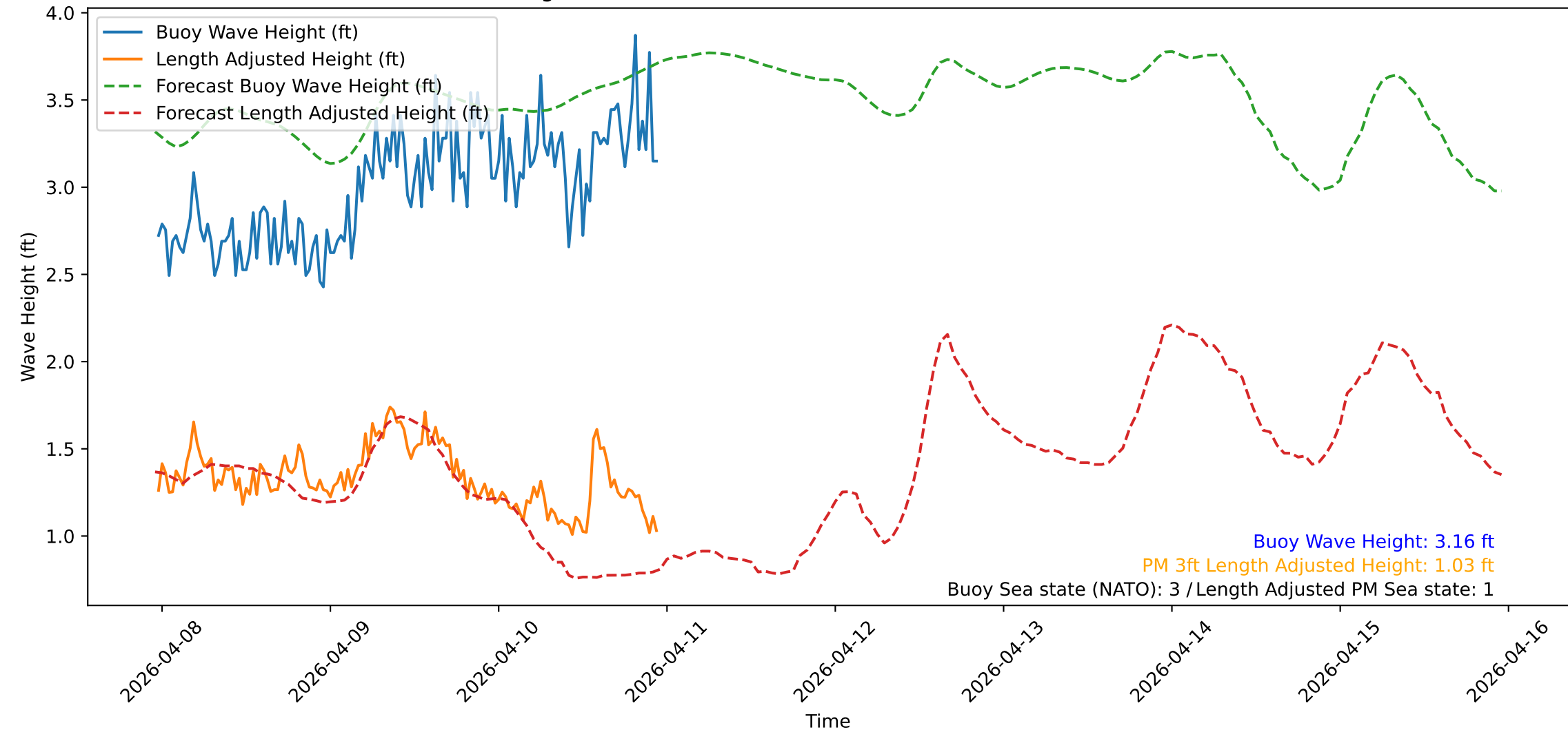
Wave Heights over Time for Oceanside Harbor at 2026-04-10 23:20:31
