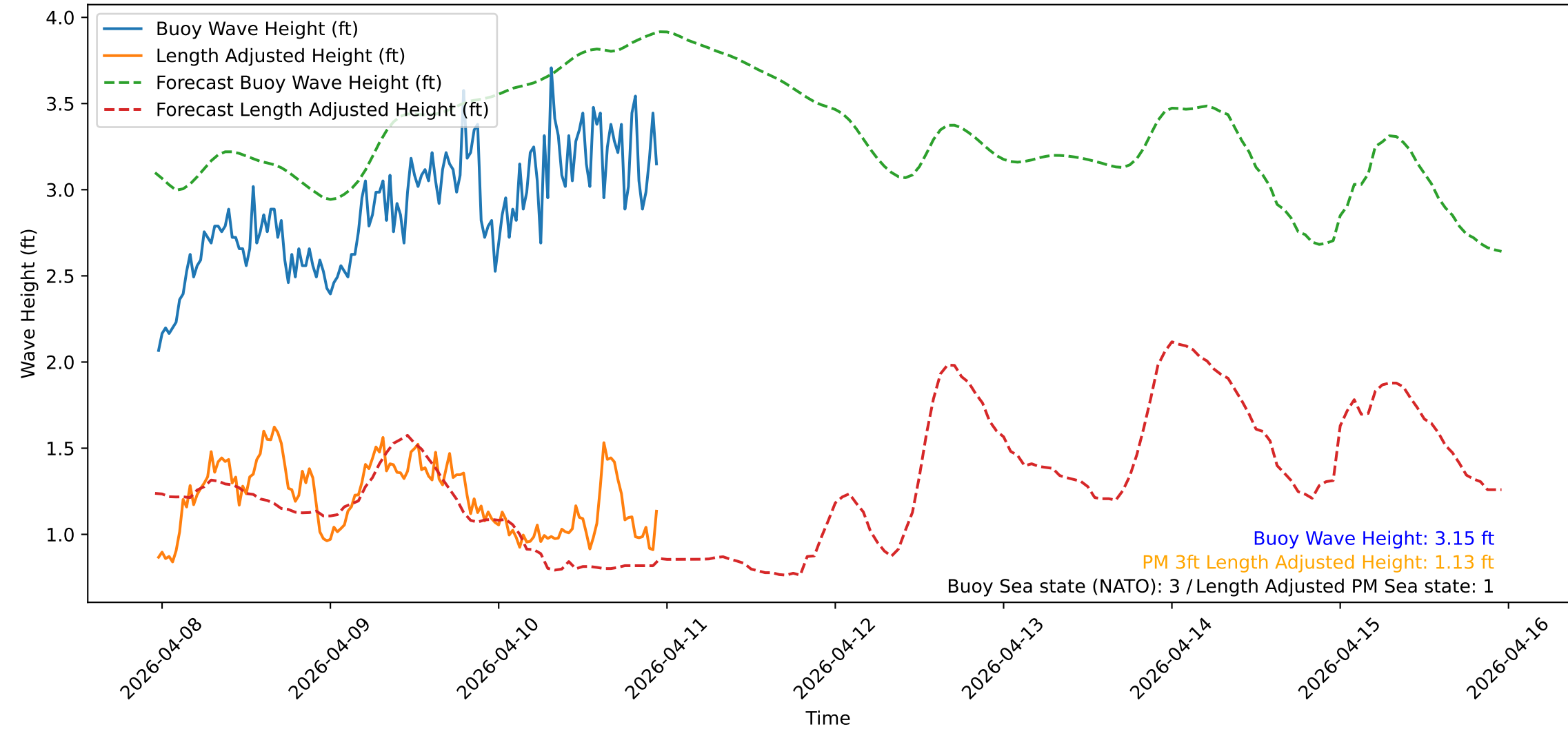
Wave Heights over Time for Red Beach at 2026-04-10 23:20:51
