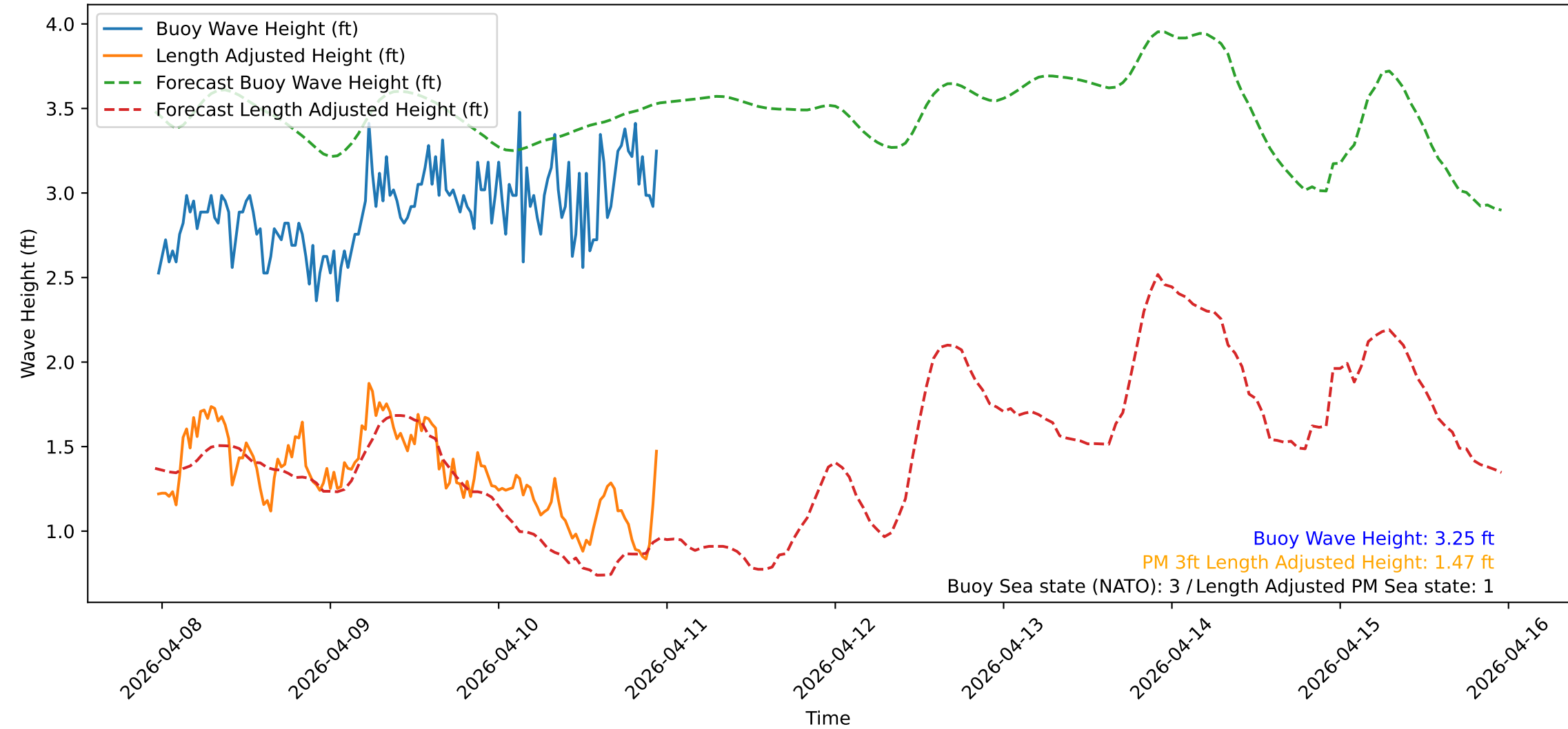
Wave Heights over Time for Green Beach at 2026-04-10 23:21:14
