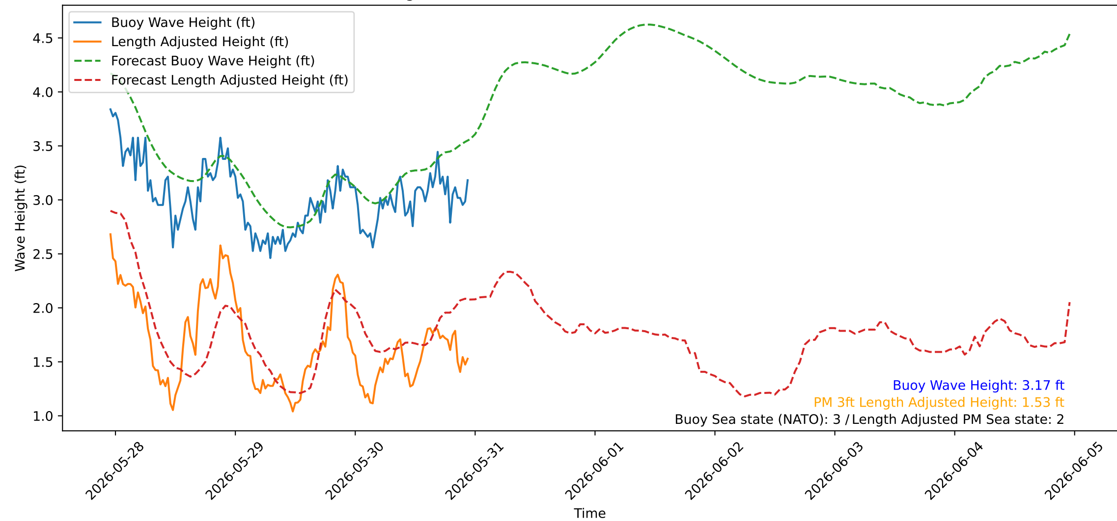
Wave Heights over Time for Green Beach at 2026-05-30 23:11:06
