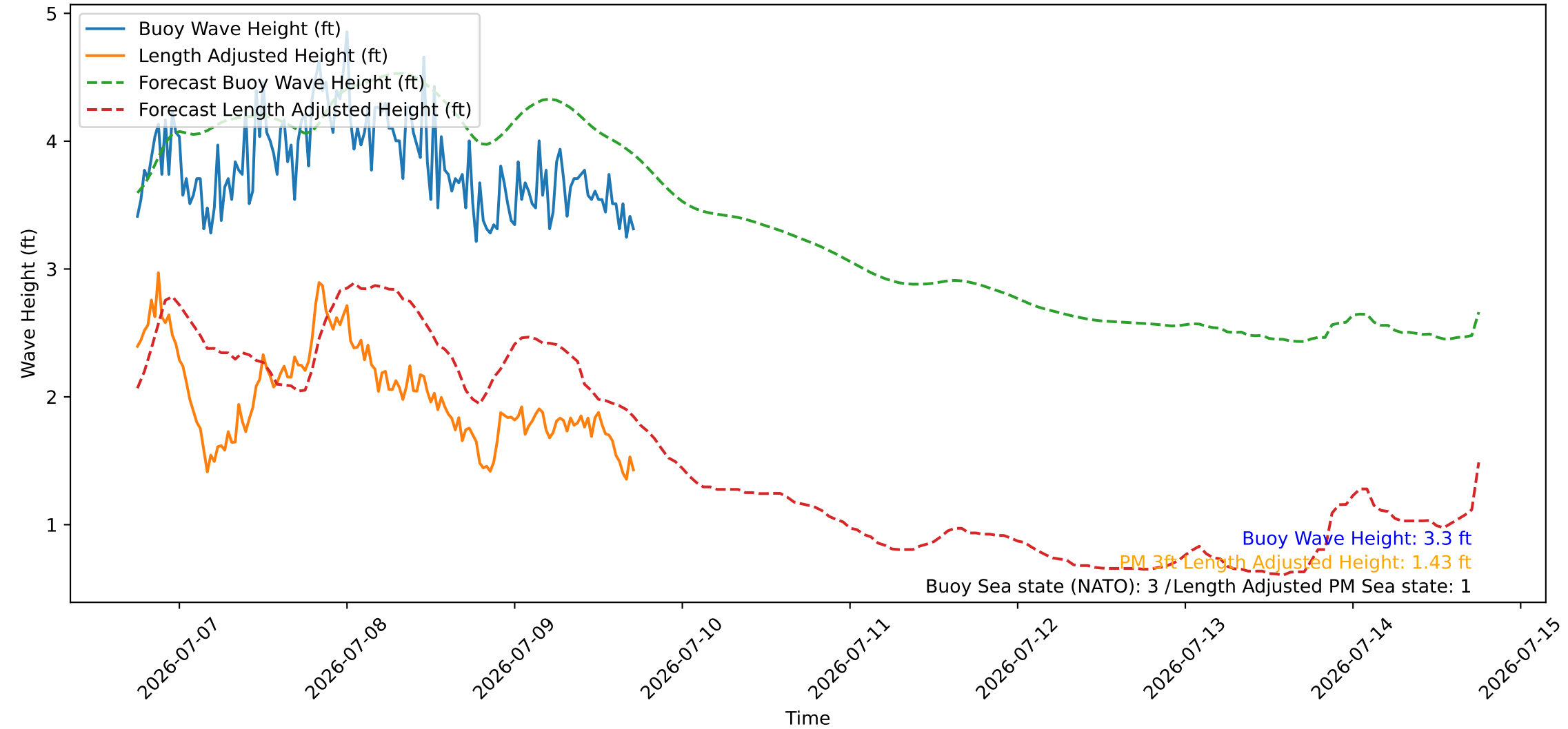
Wave Heights over Time for Red Beach at 2026-07-09 17:50:48
