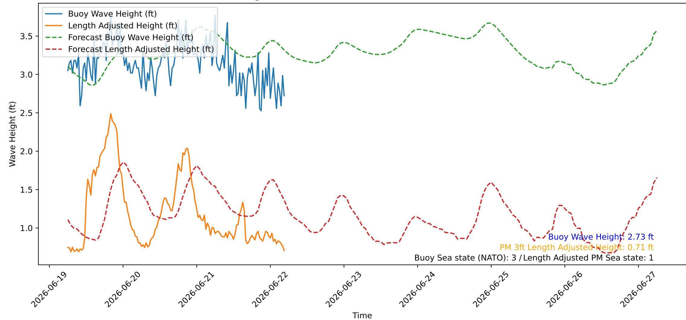
Wave Heights over Time for Red Beach at 2026-06-22 05:40:46
