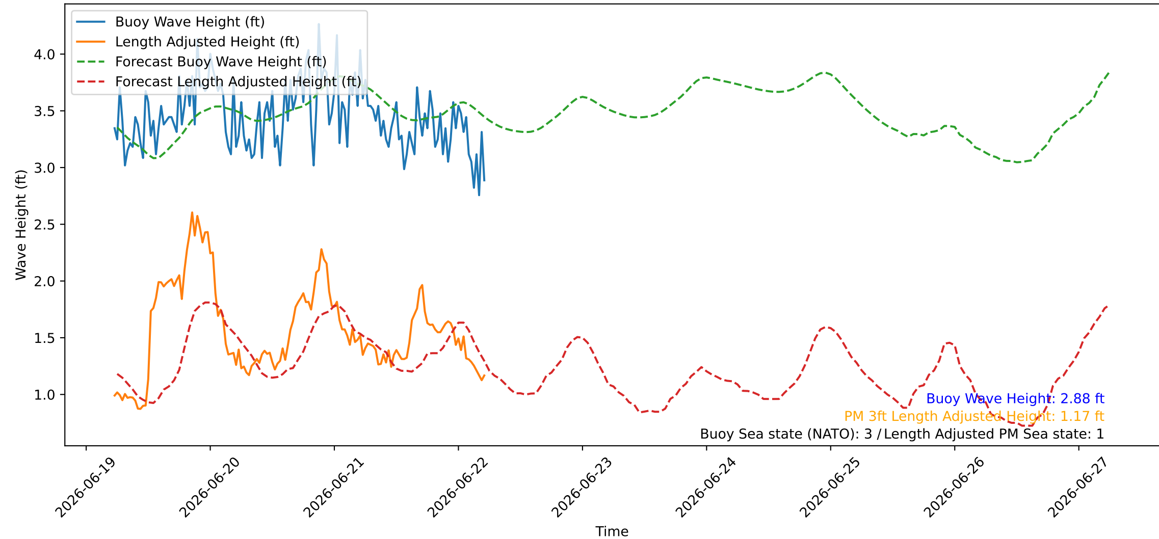
Wave Heights over Time for Oceanside Harbor at 2026-06-22 05:40:27
