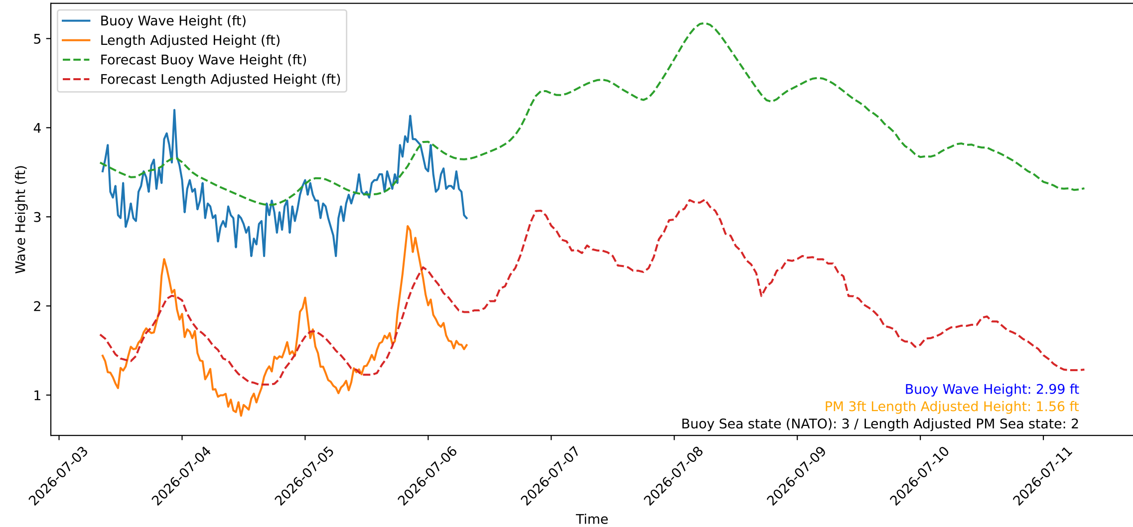
Wave Heights over Time for Green Beach at 2026-07-06 08:21:10
