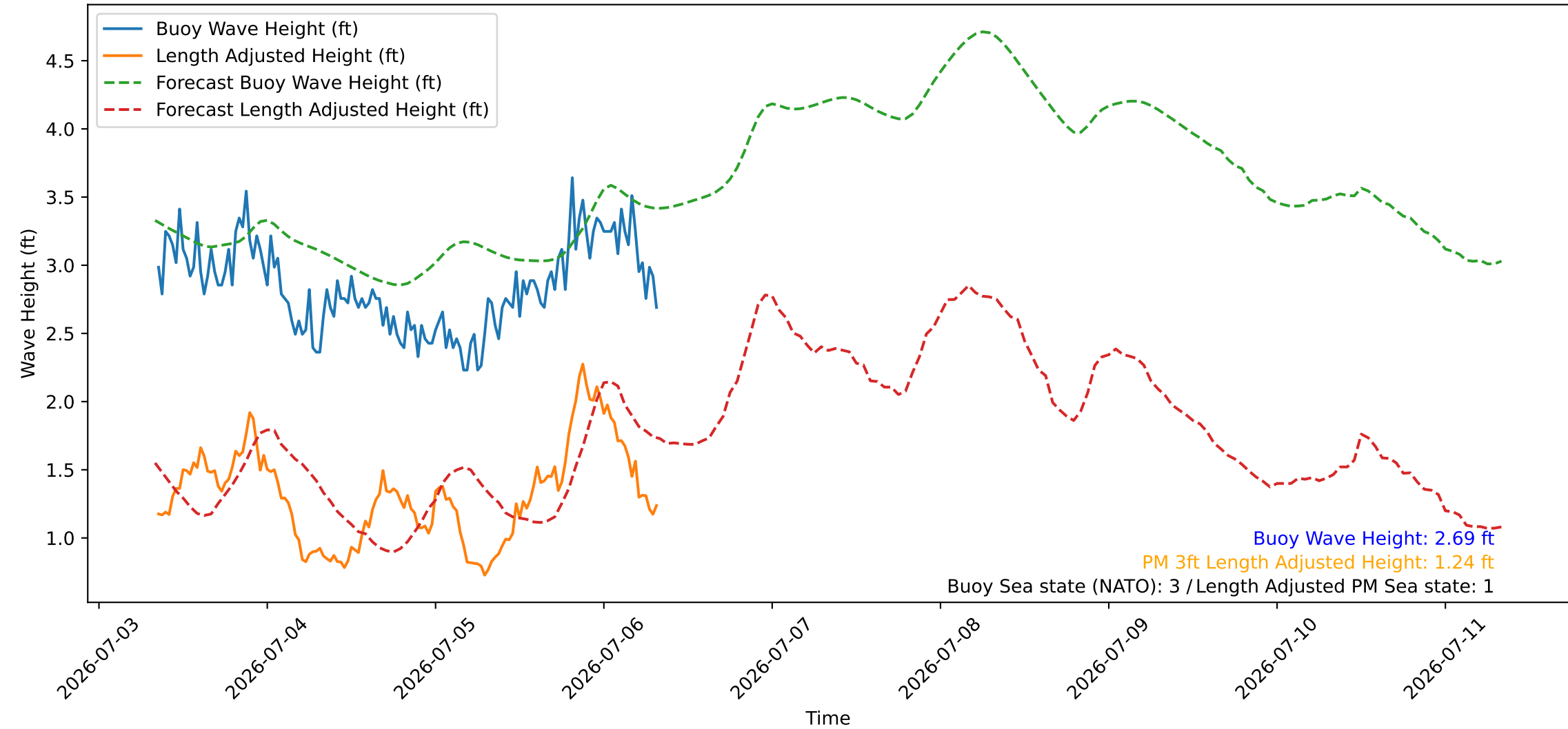
Wave Heights over Time for Red Beach at 2026-07-06 08:20:47
