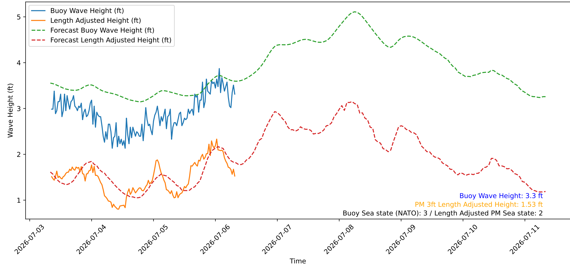
Wave Heights over Time for Oceanside Harbor at 2026-07-06 08:20:27
