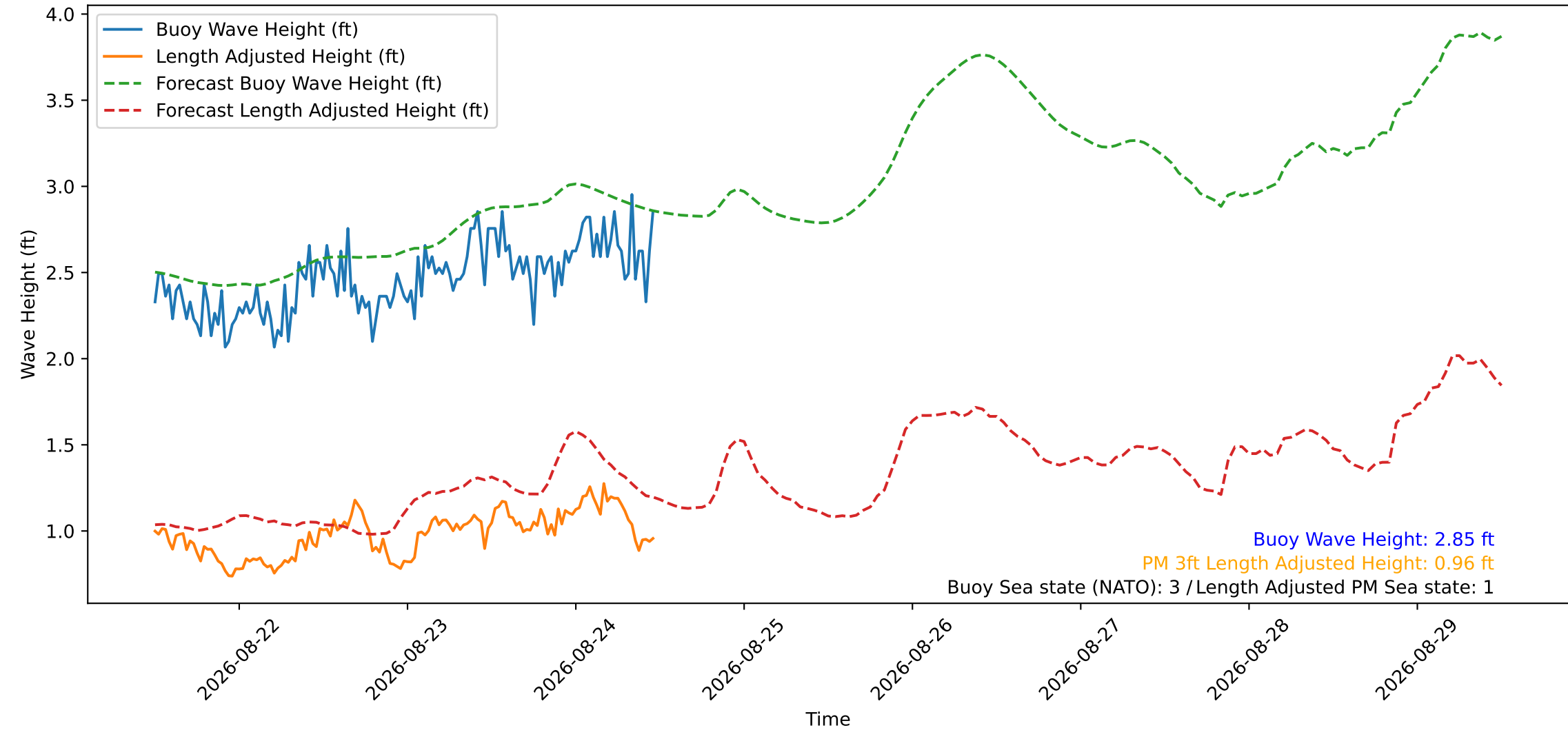
Wave Heights over Time for Red Beach at 2026-08-24 11:40:48
