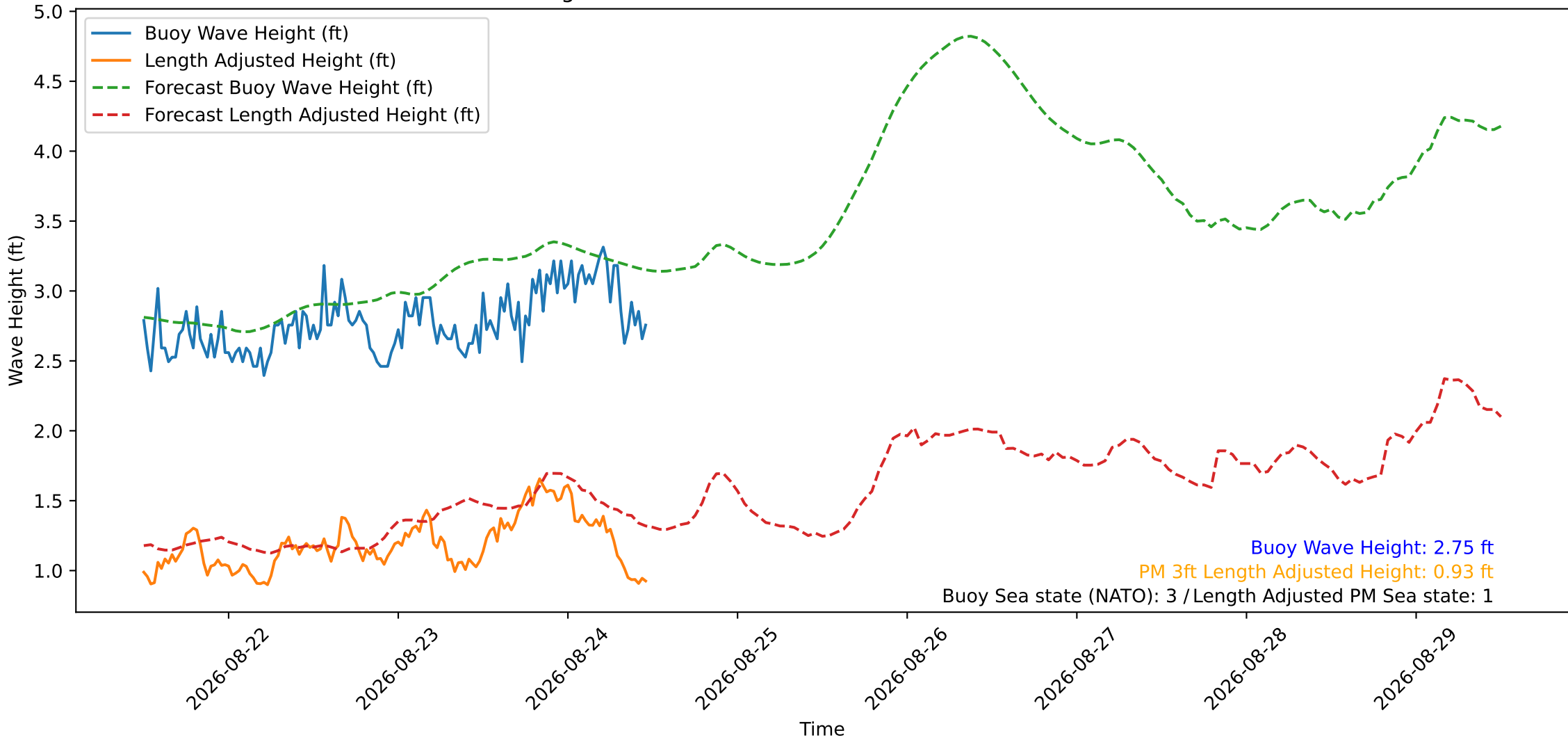
Wave Heights over Time for Green Beach at 2026-08-24 11:41:10
