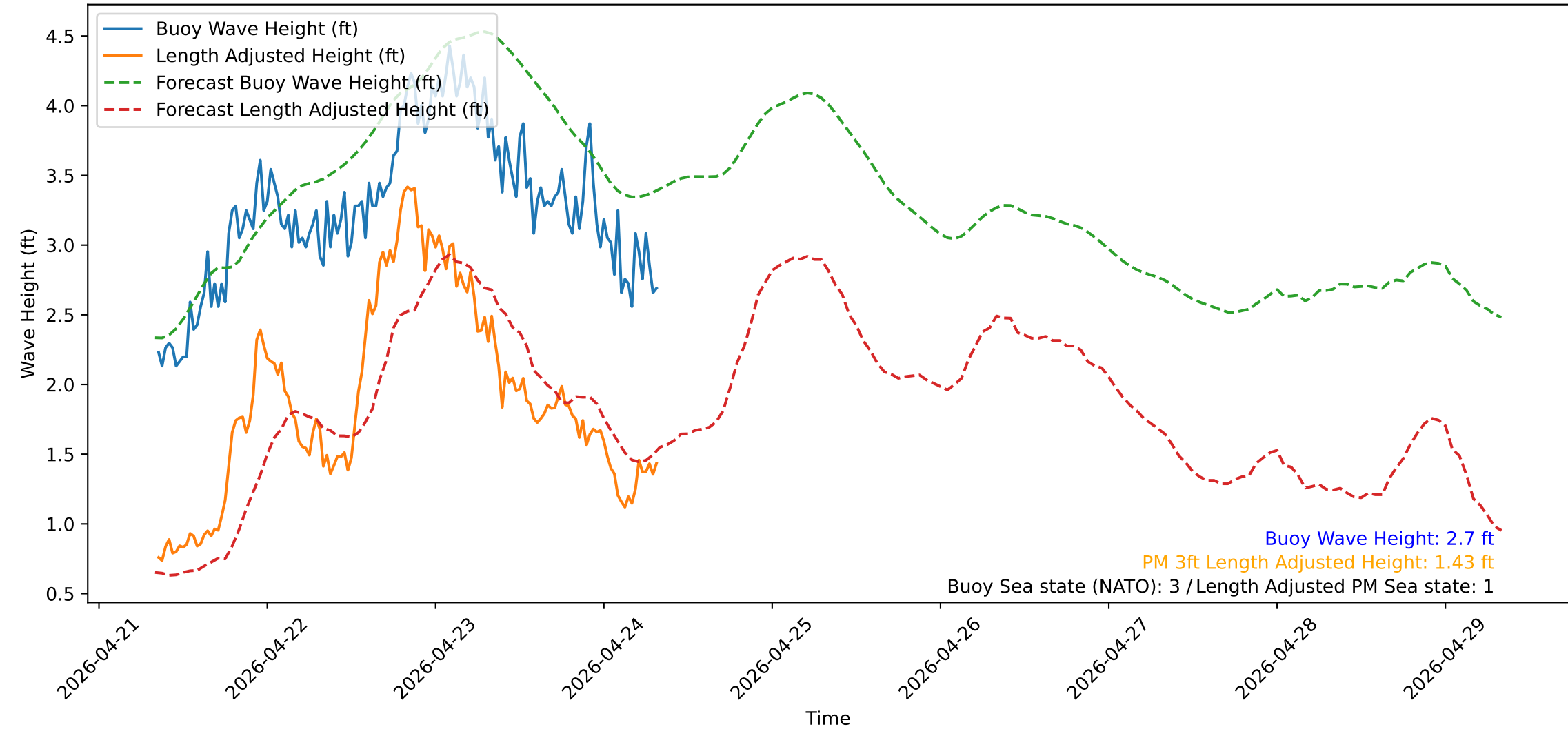
Wave Heights over Time for Oceanside Harbor at 2026-04-24 08:20:32
