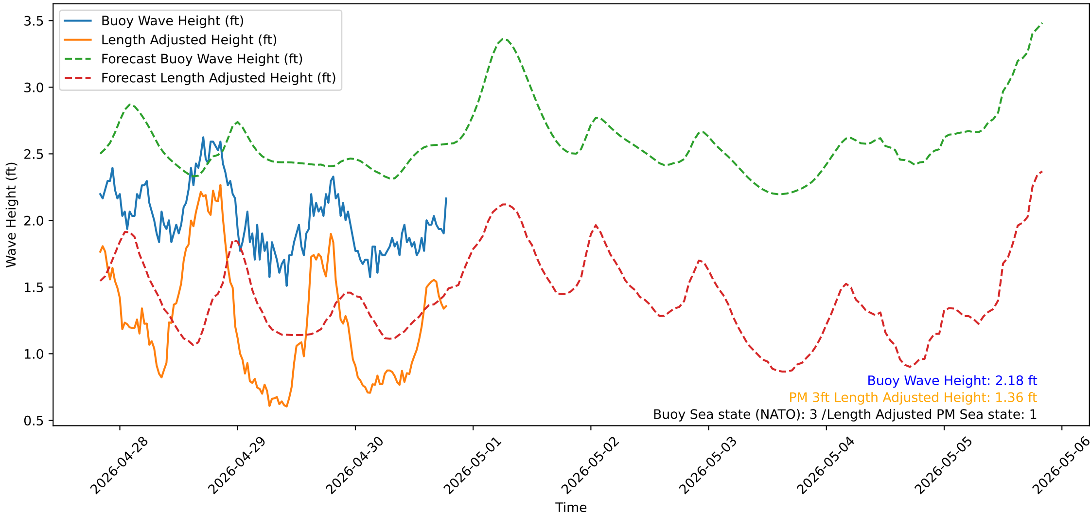
Wave Heights over Time for Red Beach at 2026-04-30 19:50:52
