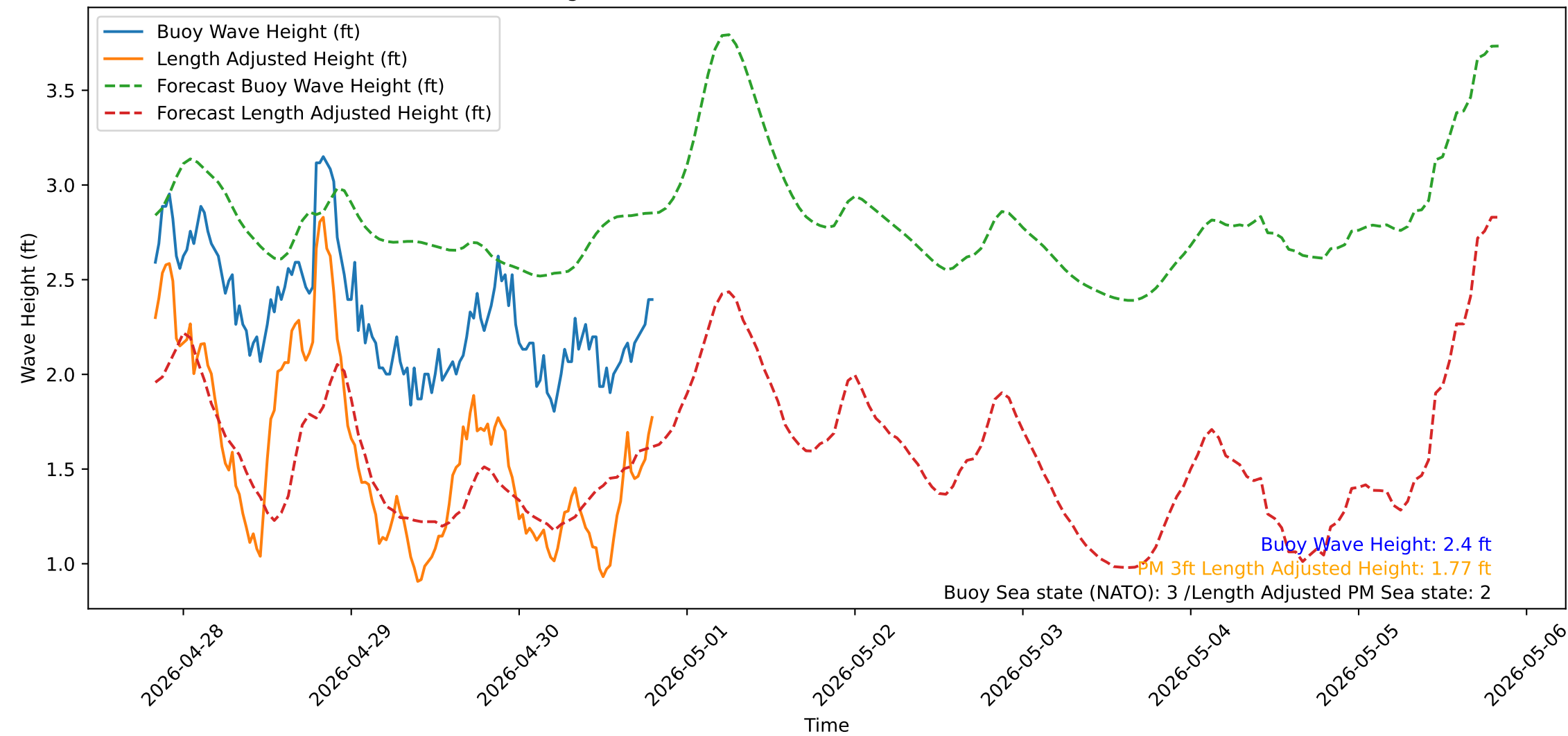
Wave Heights over Time for Green Beach at 2026-04-30 19:51:15
