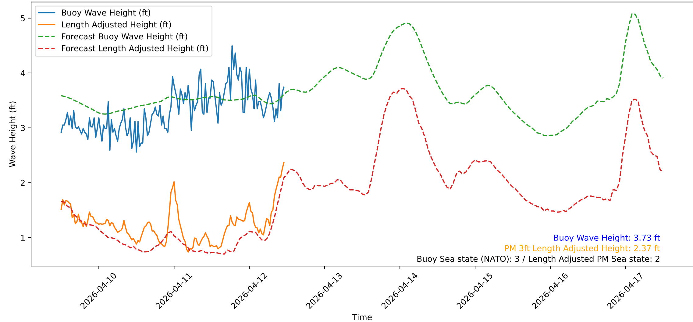
Wave Heights over Time for Green Beach at 2026-04-12 12:01:12
