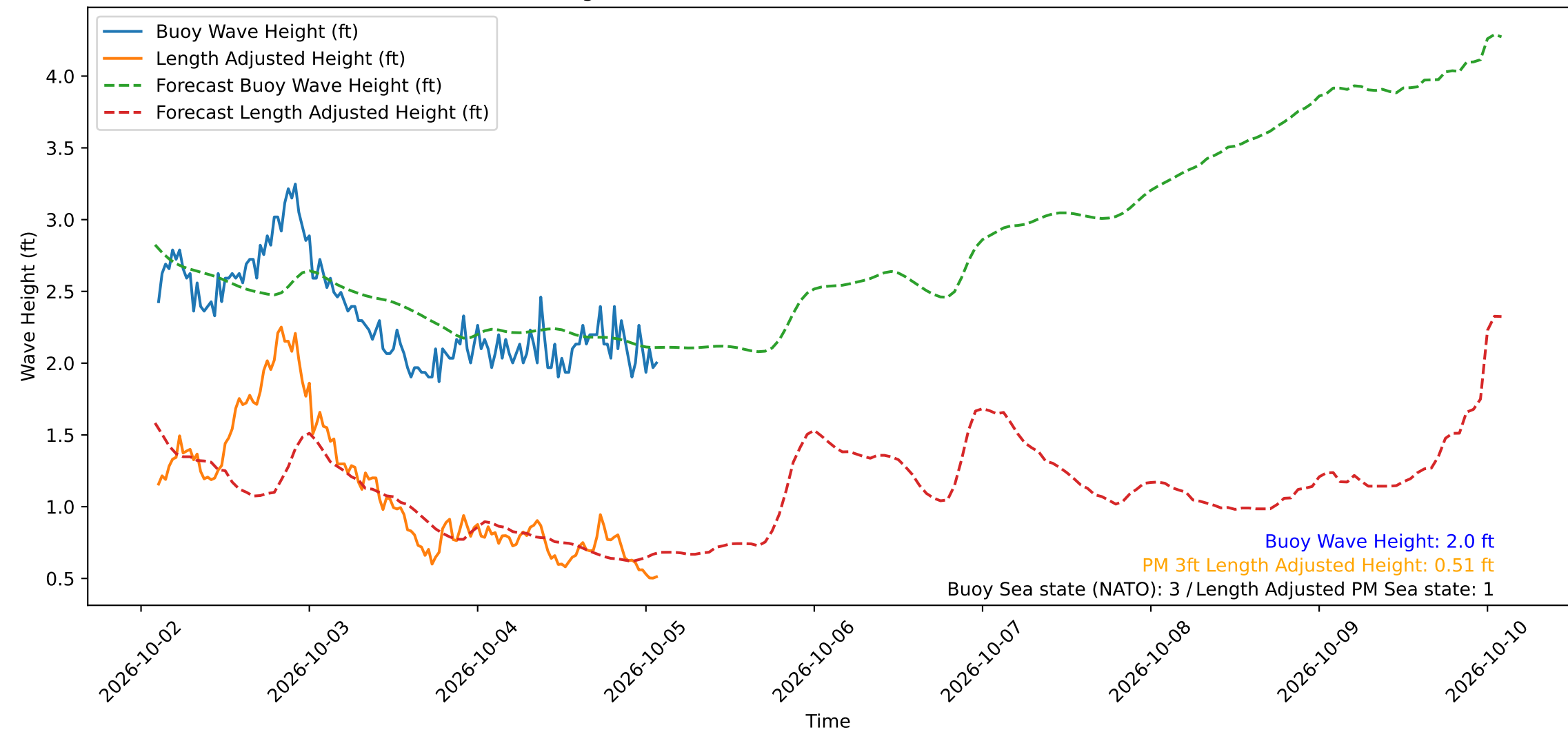
Wave Heights over Time for Red Beach at 2026-10-05 02:10:49
