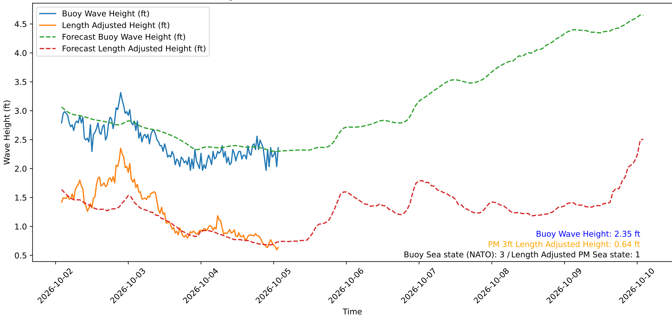
Wave Heights over Time for Oceanside Harbor at 2026-10-05 02:10:29
