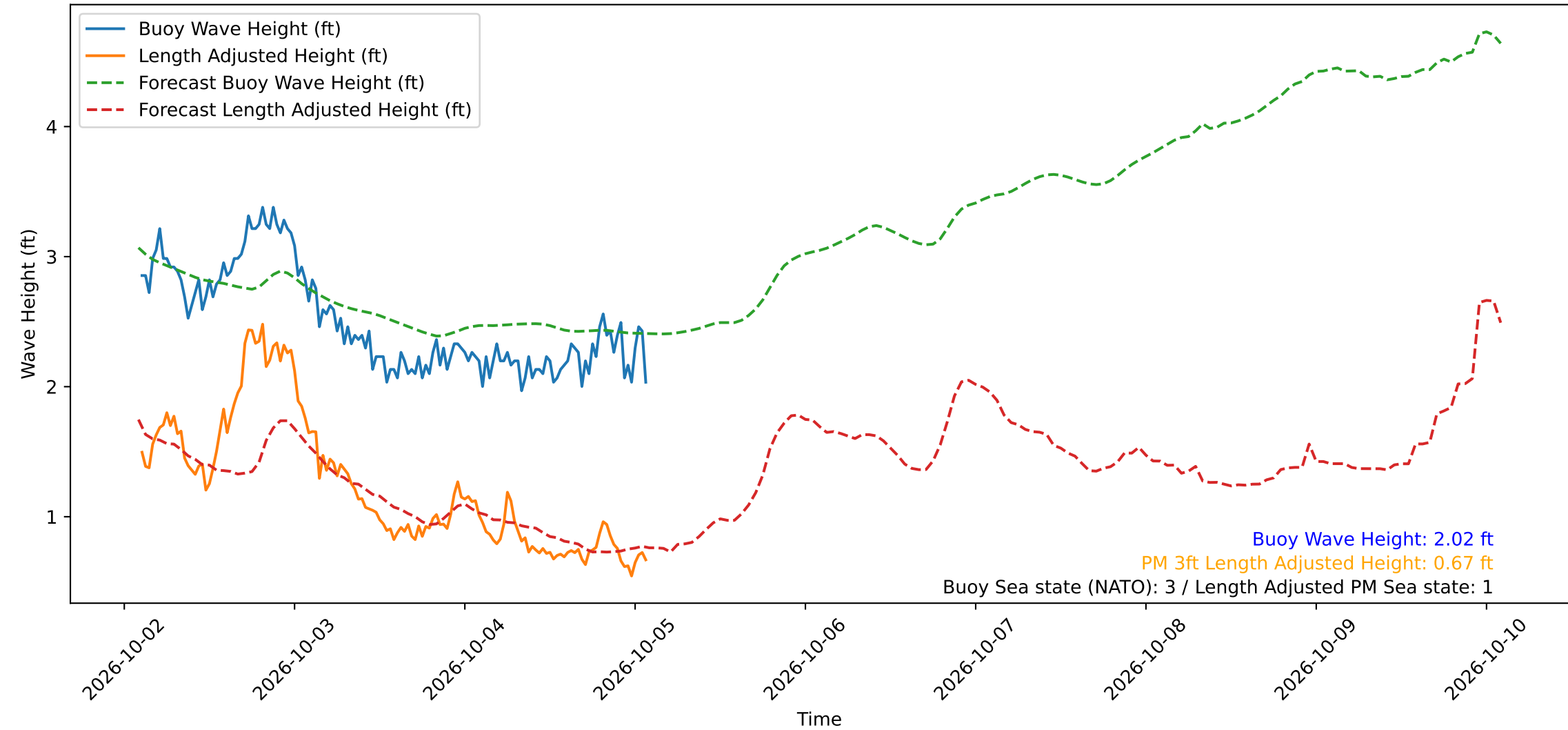
Wave Heights over Time for Green Beach at 2026-10-05 02:11:11
