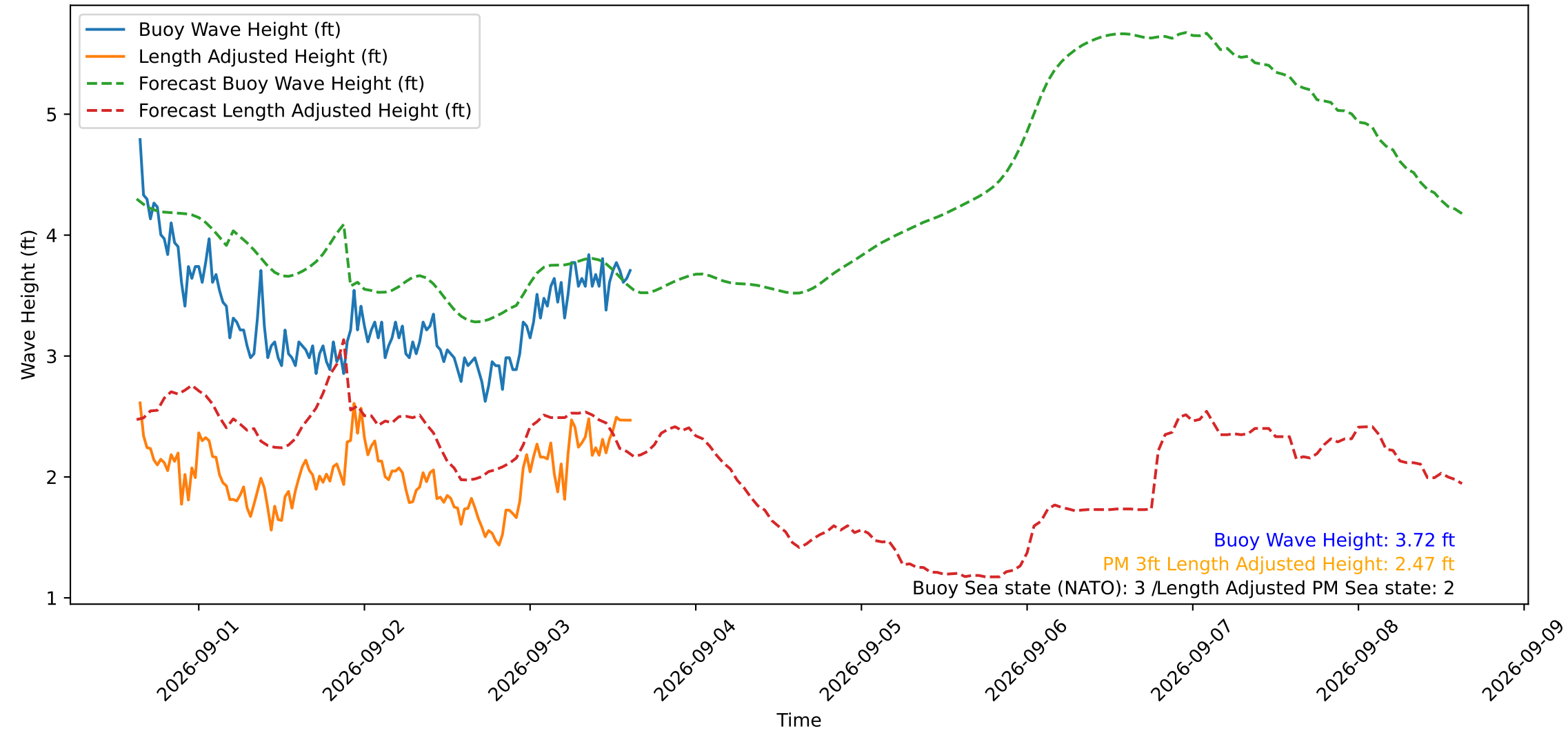
Wave Heights over Time for Oceanside Harbor at 2026-09-03 15:20:30
