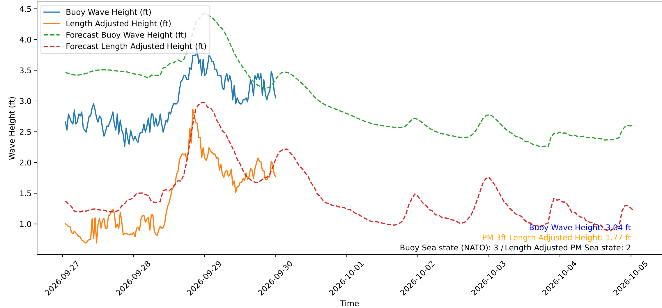
Wave Heights over Time for Red Beach at 2026-09-30 00:40:50
