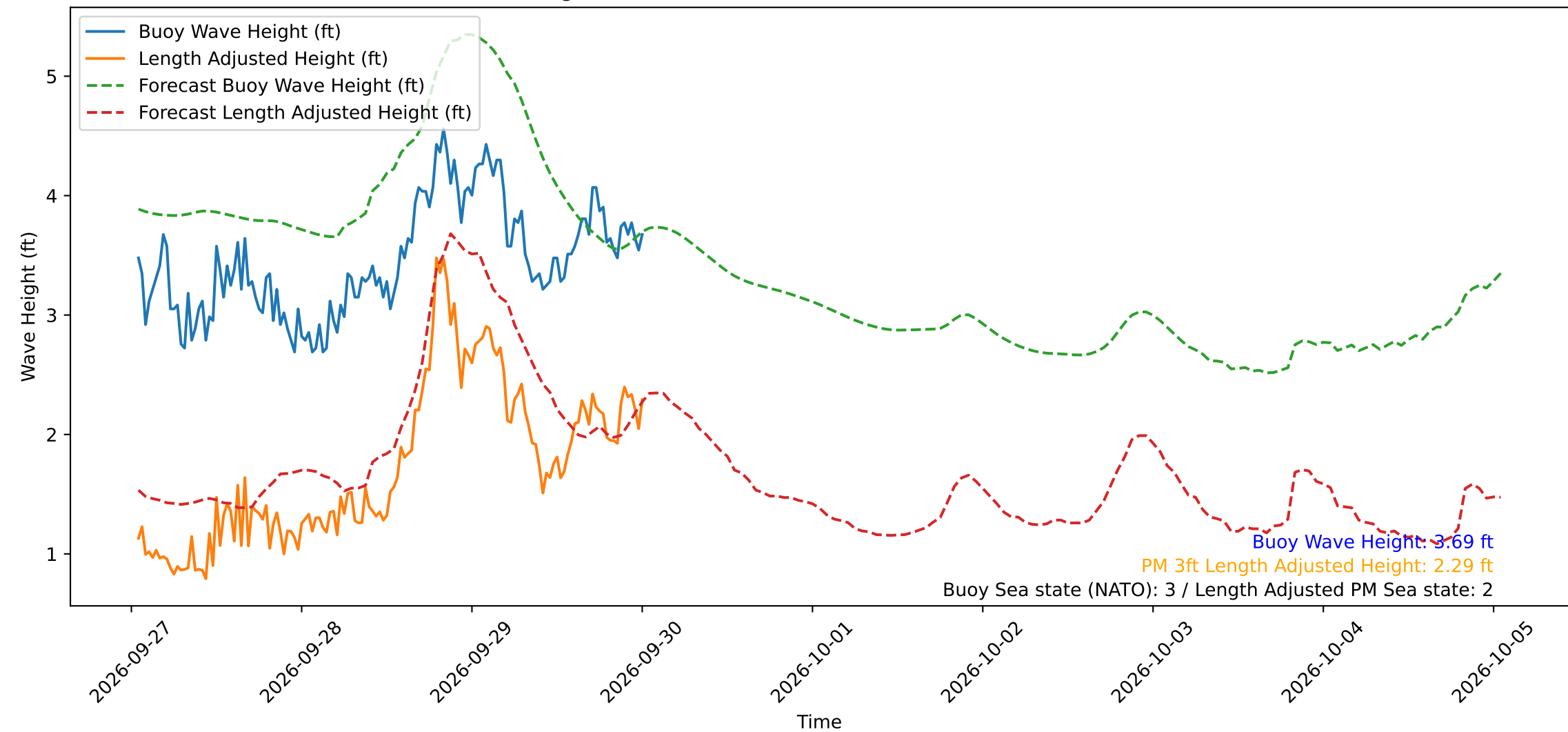
Wave Heights over Time for Green Beach at 2026-09-30 00:41:13
