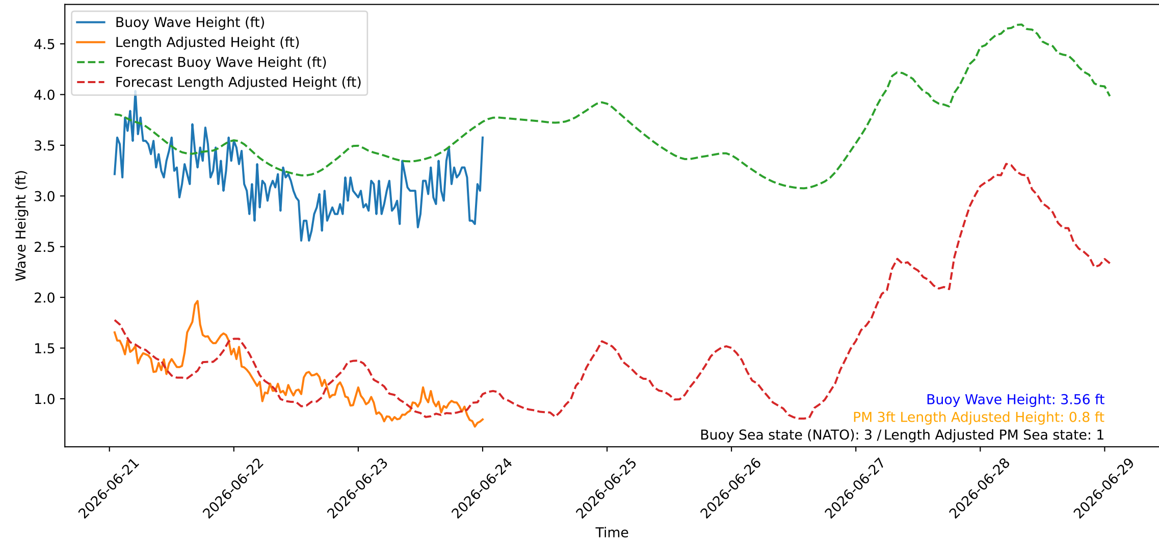
Wave Heights over Time for Oceanside Harbor at 2026-06-24 00:50:26
