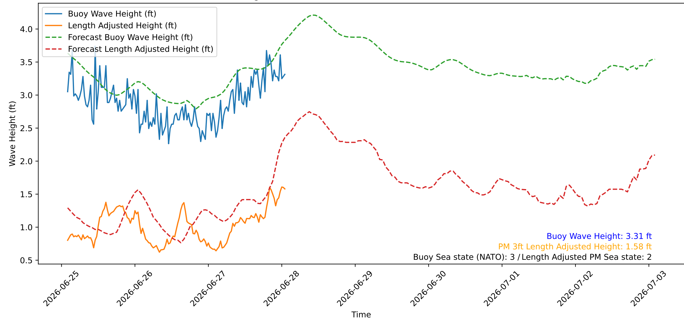
Wave Heights over Time for Red Beach at 2026-06-28 01:50:46
