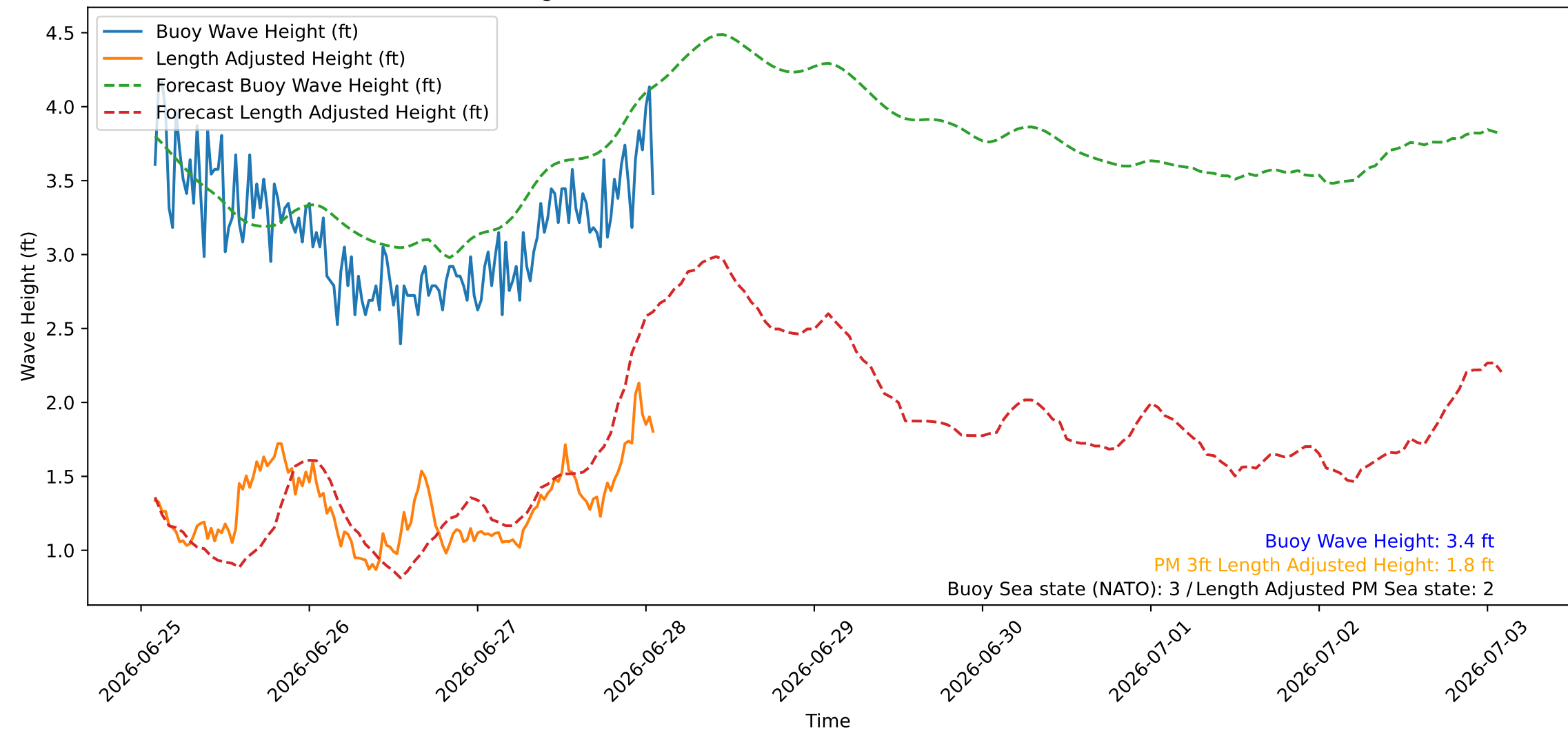
Wave Heights over Time for Oceanside Harbor at 2026-06-28 01:50:25
