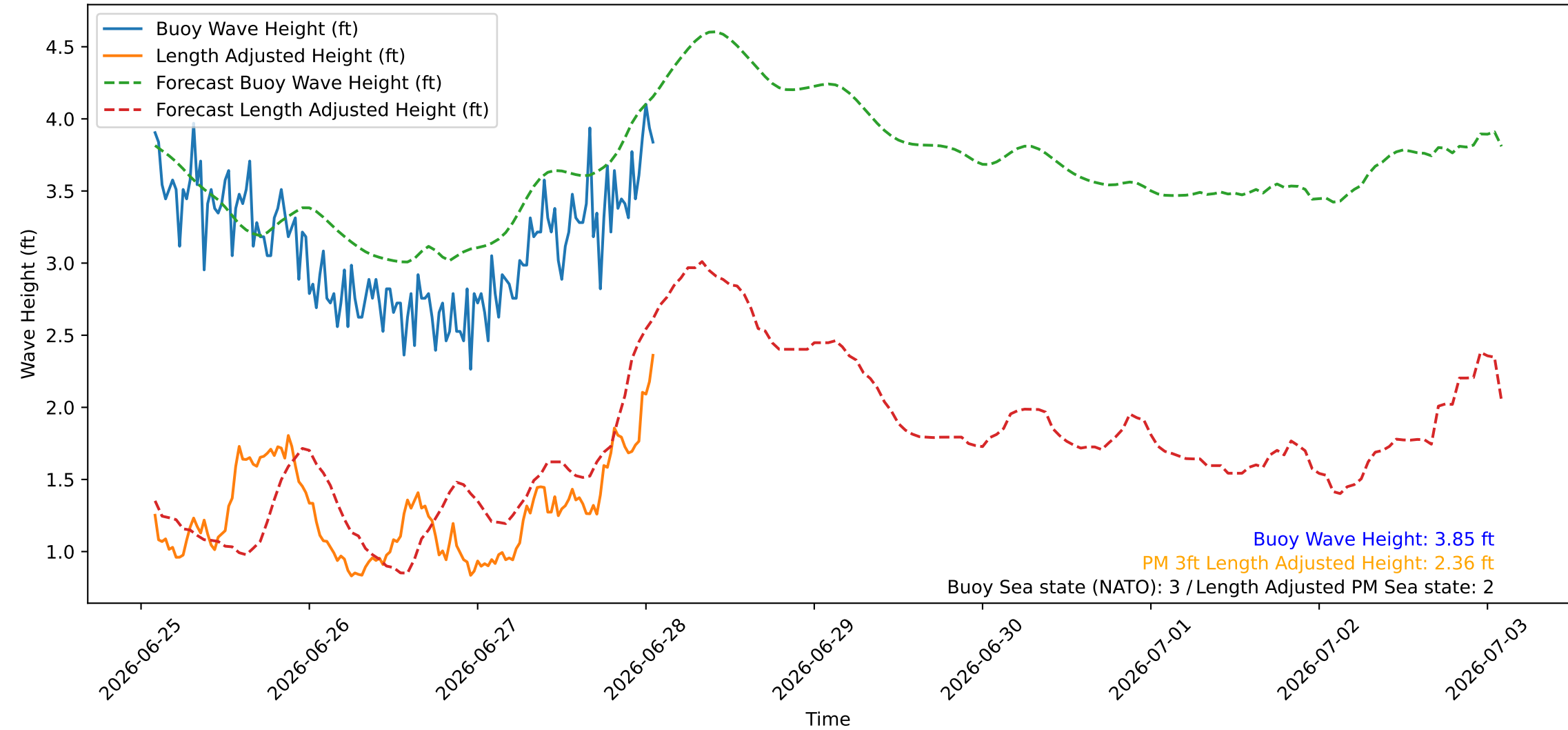
Wave Heights over Time for Green Beach at 2026-06-28 01:51:08
