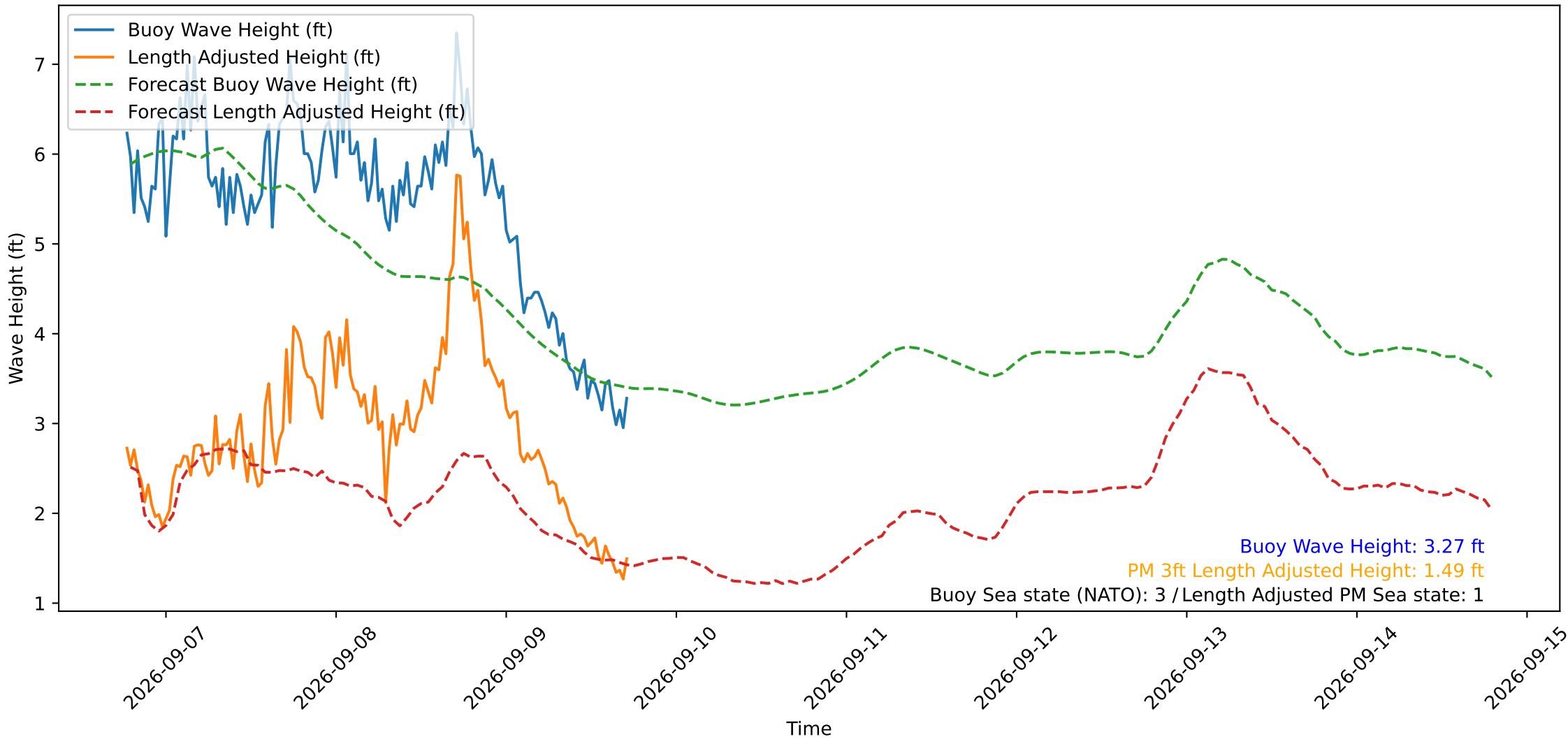
Wave Heights over Time for Oceanside Harbor at 2026-09-09 18:30:30
