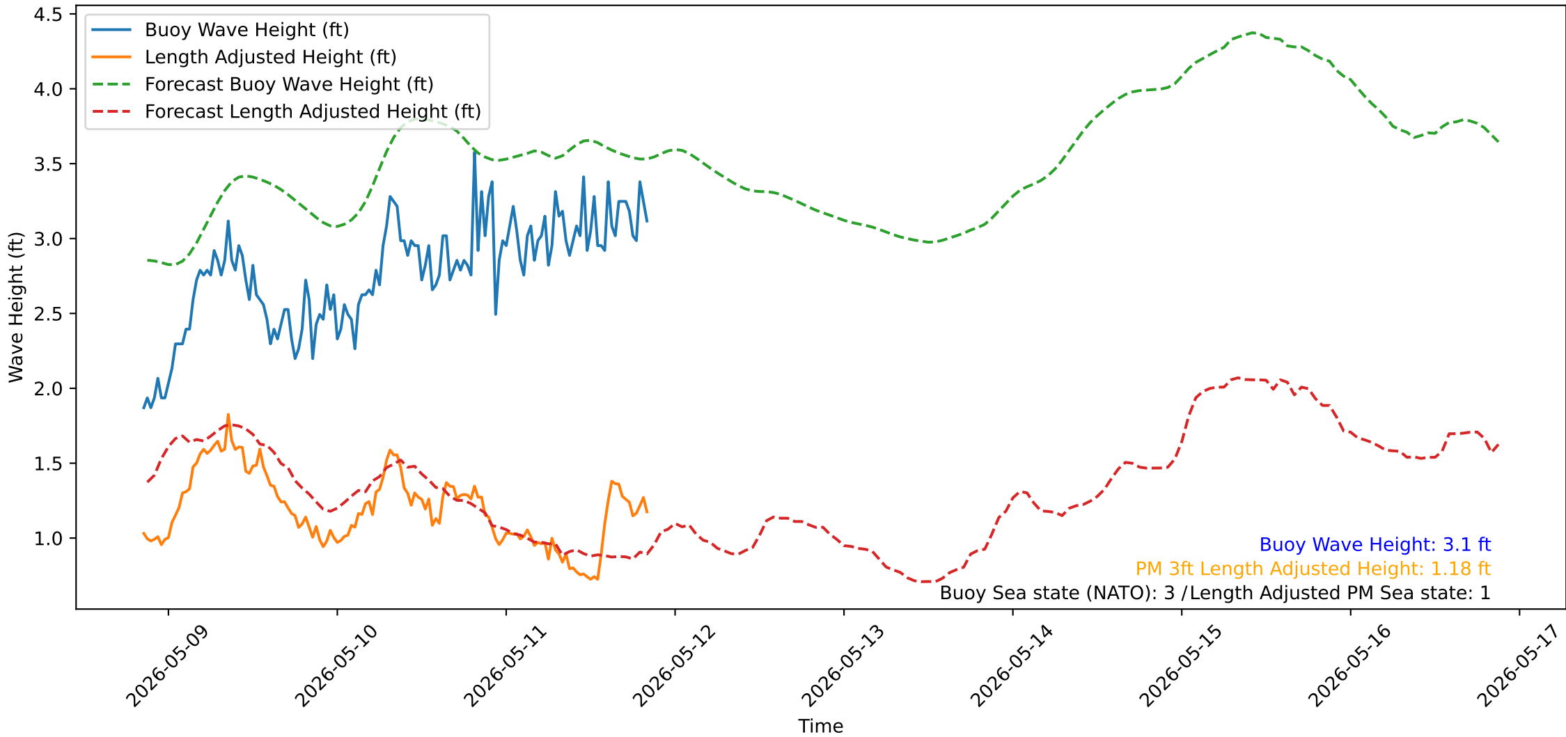
Wave Heights over Time for Oceanside Harbor at 2026-05-11 20:40:32
