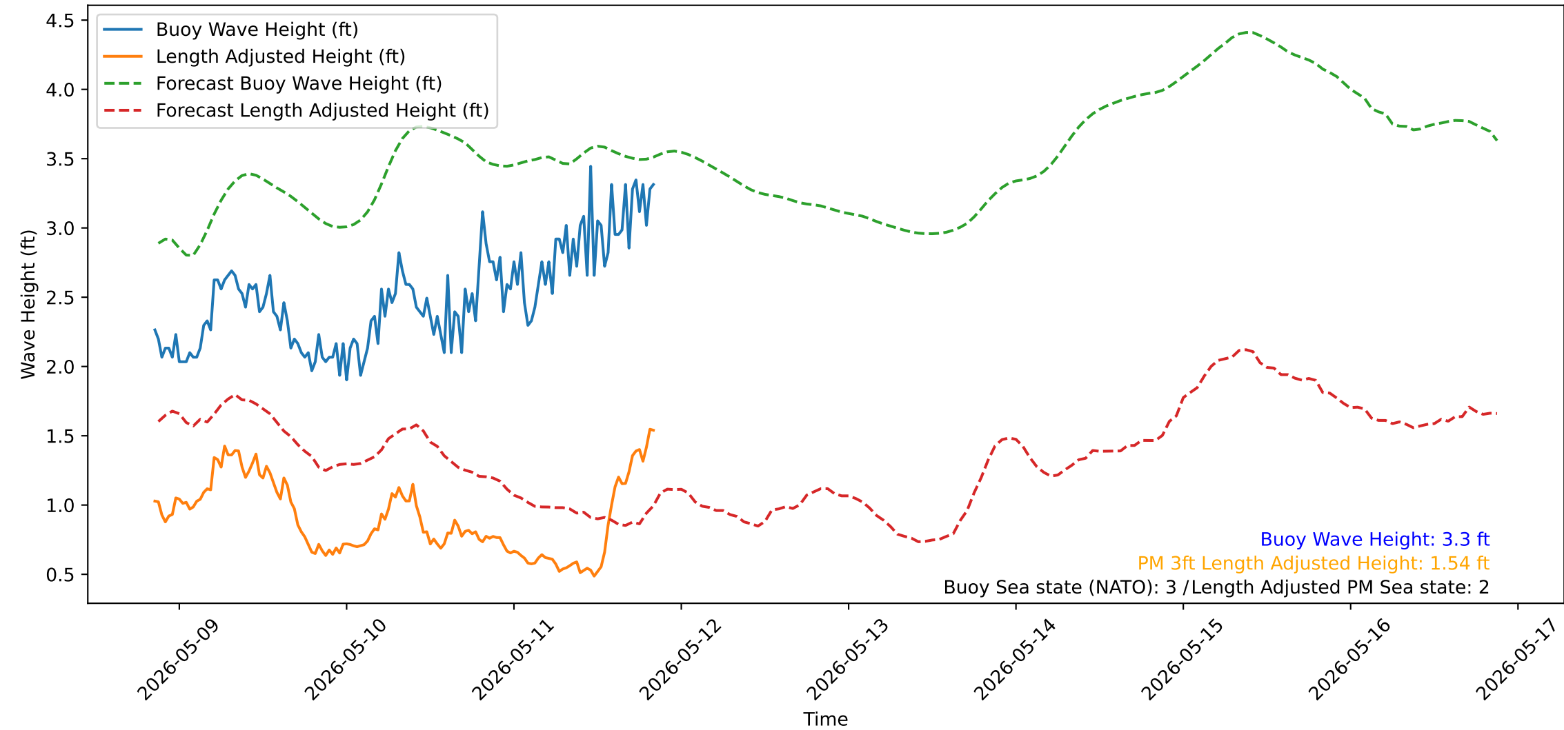
Wave Heights over Time for Green Beach at 2026-05-11 20:41:13
